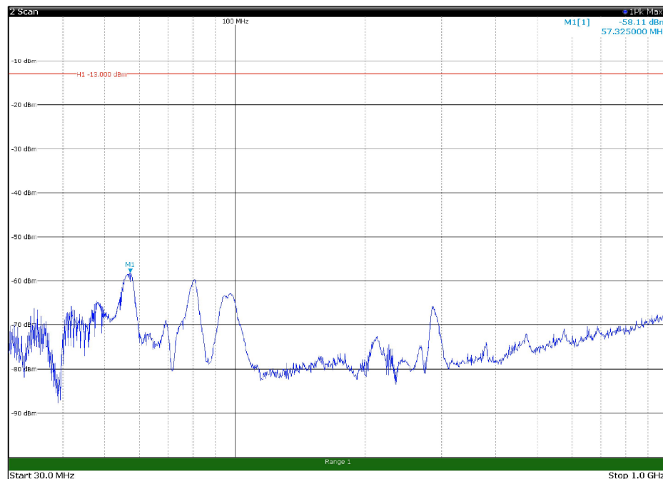
Channel: BOTTOM, Modulation: 16QAM, BW=5MHz, Range: 30MHz - 1GHz, Polarization: Vertical
