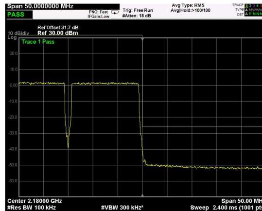
High Band Edge, 2 Carrier, Modulation: 64QAM, BW=15MHz
