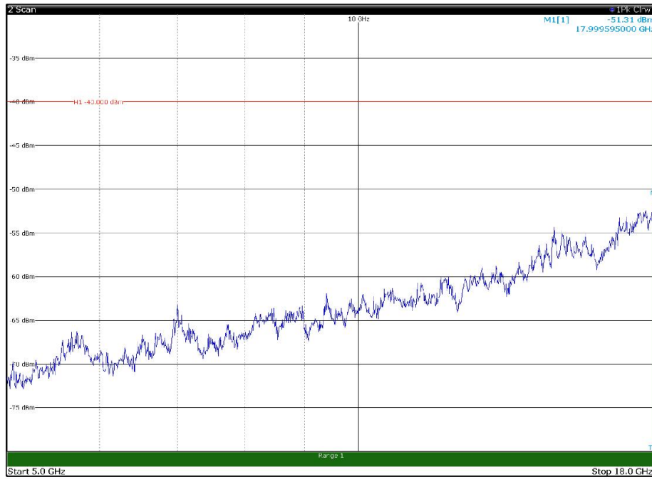
Channel: MIDDLE, Modulation: QPSK, BW=20MHz, Range: 5GHz - 18GHz, Polarization: Horizontal
