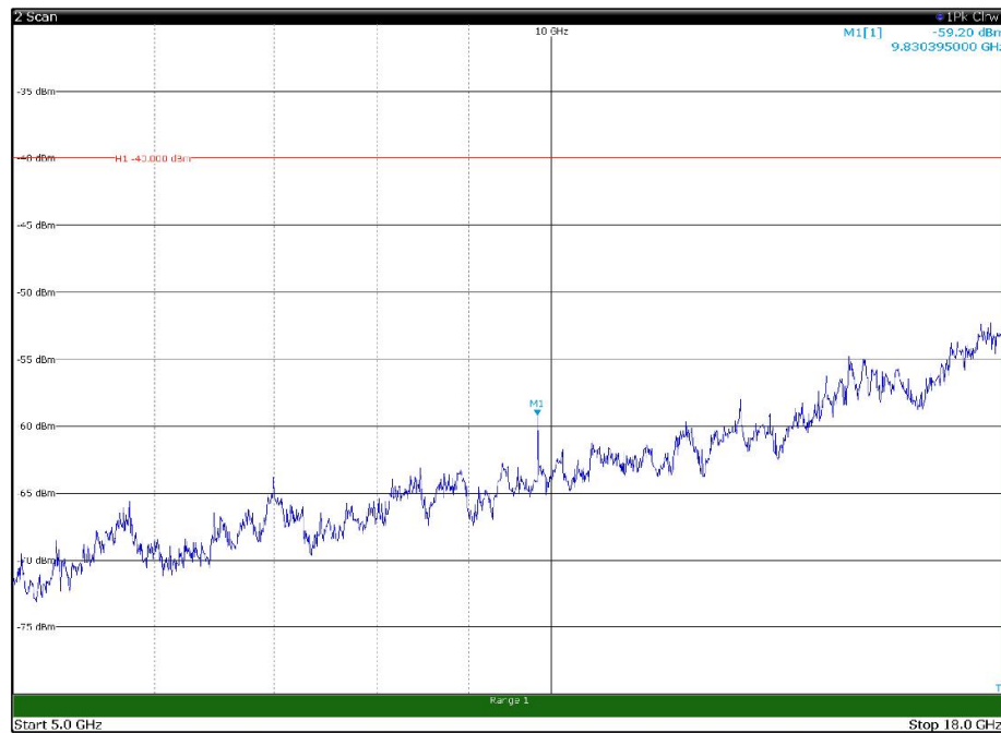
Channel: TOP, Modulation: 16QAM, BW=20MHz, Range: 5GHz - 18GHz, Polarization: Horizontal
