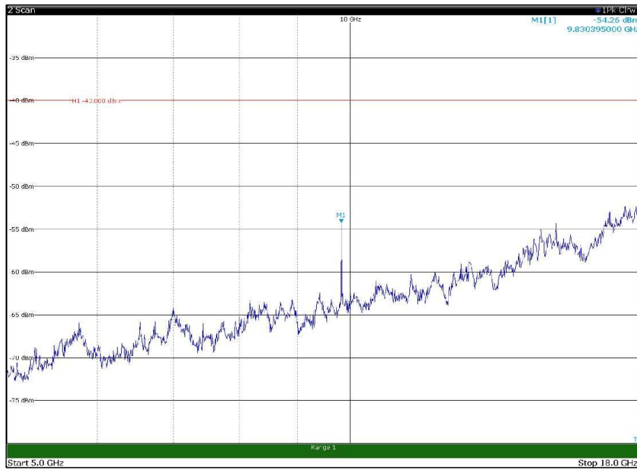
Channel: MIDDLE, Modulation: QPSK, BW=20MHz, Range: 5GHz - 18GHz, Polarization: Vertical
