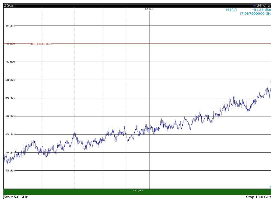
Channel: TOP, Modulation: 16QAM, BW=20MHz, Range: 5GHz - 18GHz, Polarization: Vertical
