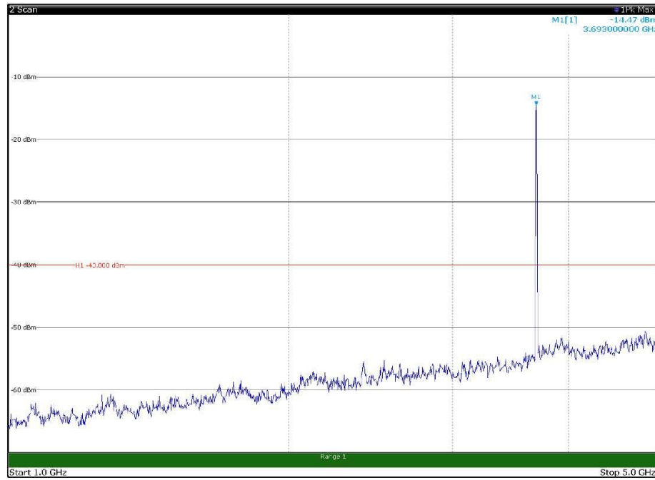
Channel: TOP, Modulation: QPSK, BW=10MHz, Range: 1GHz - 5GHz, Polarization: Horizontal
