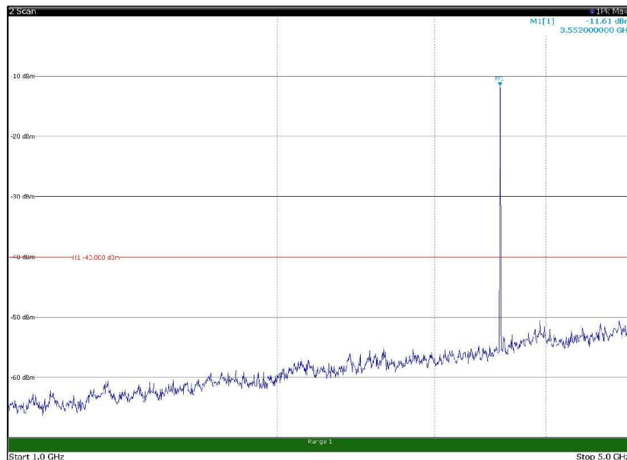
Channel: BOTTOM, Modulation: 16QAM, BW=10MHz, Range: 1GHz - 5GHz, Polarization: Vertical
