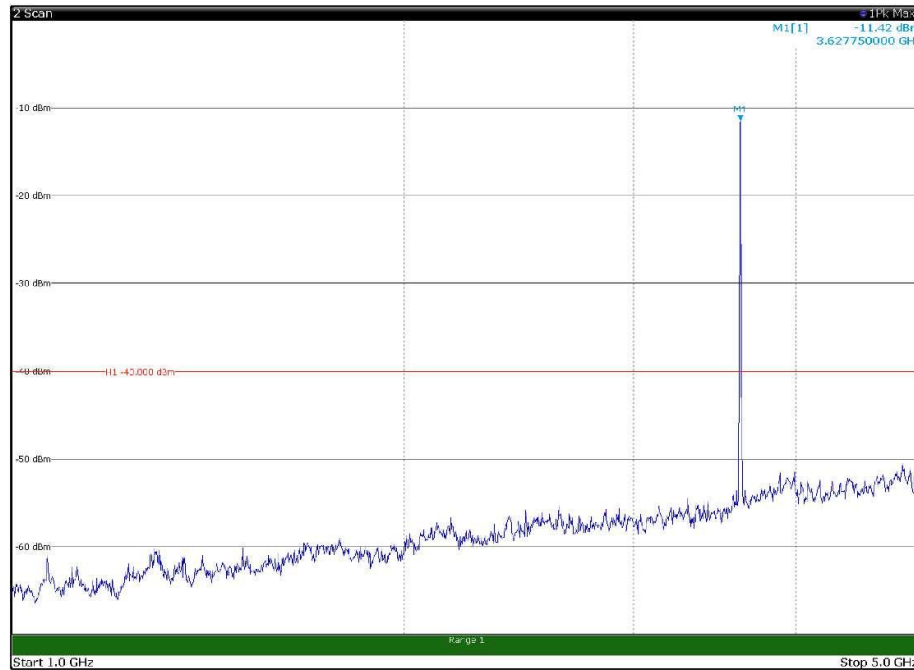
Channel: MIDDLE, Modulation: 16QAM, BW=10MHz, Range: 1GHz - 5GHz, Polarization: Horizontal
