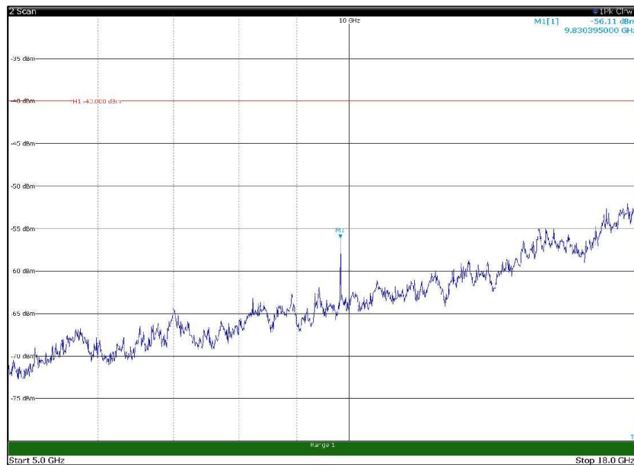
Channel: MIDDLE, Modulation: 64QAM, BW=10MHz, Range: 5GHz - 18GHz, Polarization: Vertical
