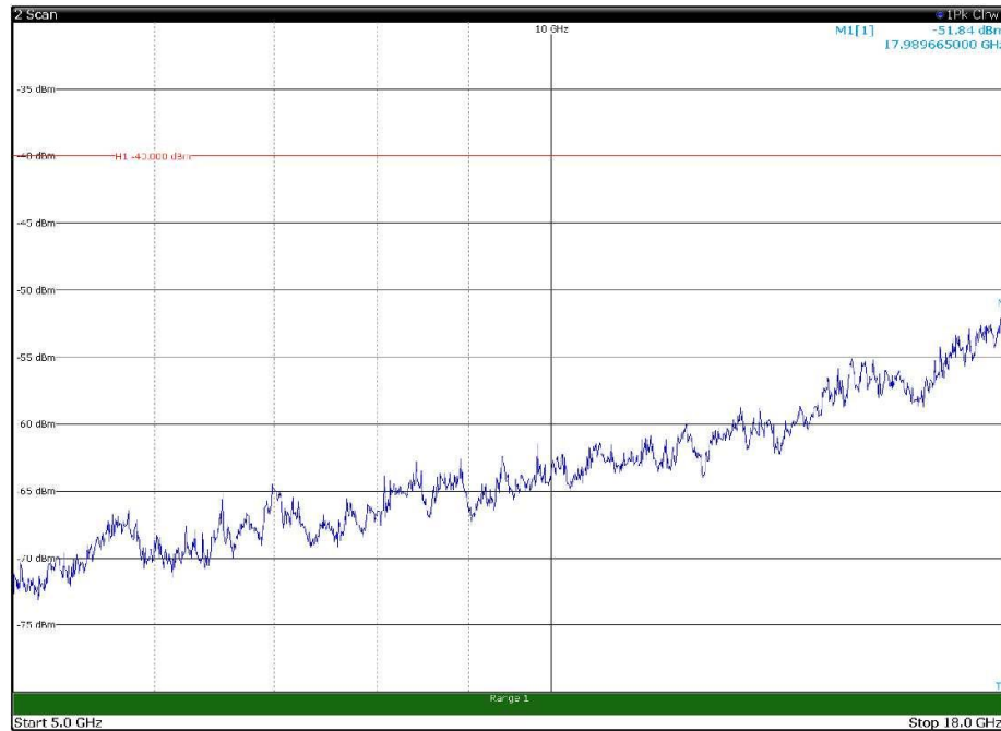
Channel: MIDDLE, Modulation: 64QAM, BW=10MHz, Range: 5GHz - 18GHz, Polarization: Horizontal
