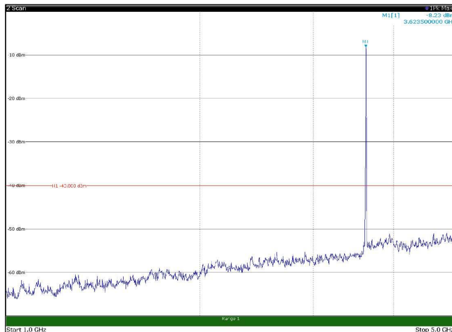
Channel: MIDDLE, Modulation: 16QAM, BW=10MHz, Range: 1GHz - 5GHz, Polarization: Vertical
