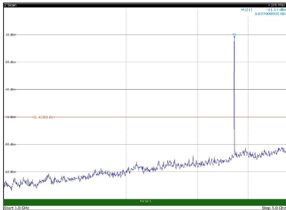
Channel: TOP, Modulation: QPSK, BW=10MHz, Range: 1GHz - 5GHz, Polarization: Vertical
