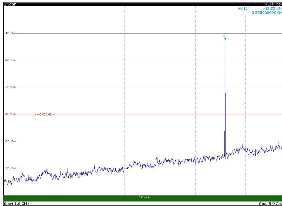
Channel: BOTTOM, Modulation: 16QAM, BW=10MHz, Range: 1GHz - 5GHz, Polarization: Horizontal
