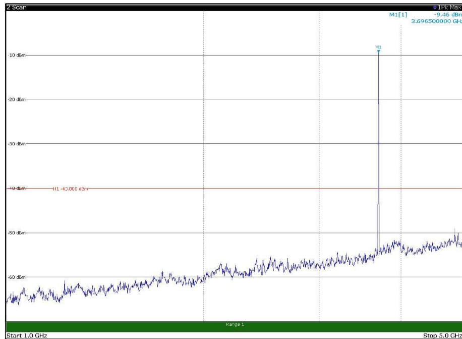
Channel: TOP, Modulation: 256QAM, BW=5MHz, Range: 1GHz - 5GHz, Polarization: Vertical
