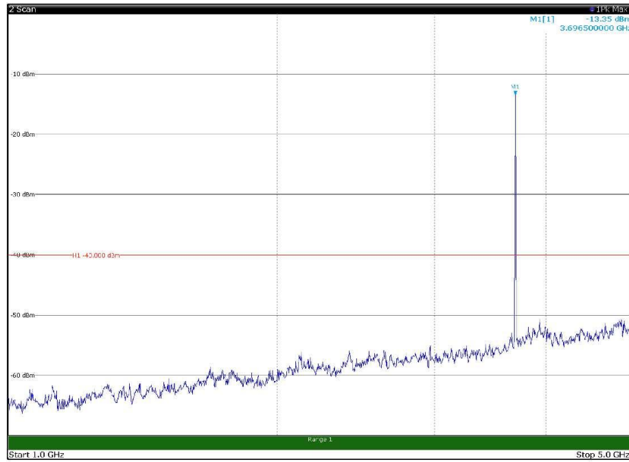
Channel: TOP, Modulation: 256QAM, BW=5MHz, Range: 1GHz - 5GHz, Polarization: Horizontal
