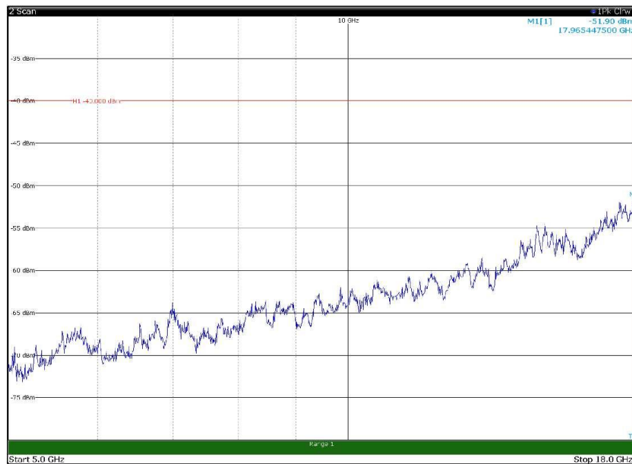
Channel: TOP, Modulation: 16QAM, BW=5MHz, Range: 5GHz - 18GHz, Polarization: Vertical
