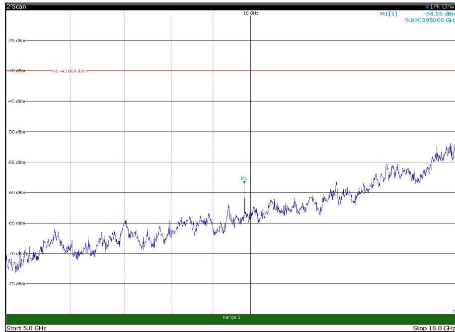
Channel: TOP, Modulation: 16QAM, BW=5MHz, Range: 5GHz - 18GHz, Polarization: Horizontal
