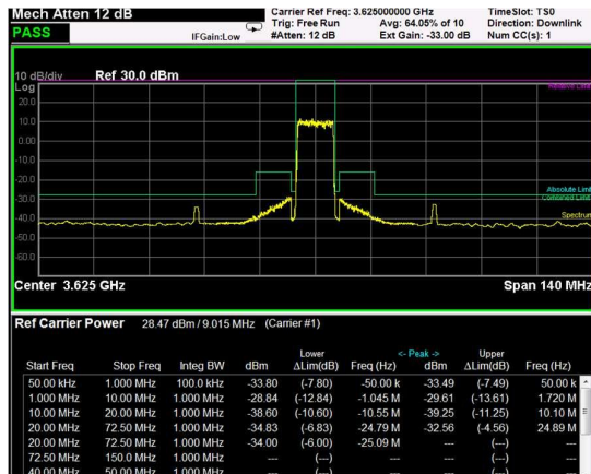
Middle Band Edge, 1 Carrier, Modulation: 256QAM, BW=10MHz
