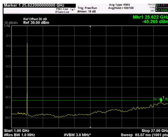
Channel: MIDDLE, Modulation: QPSK, BW=20MHz, Range: 1GHz - 27GHz
