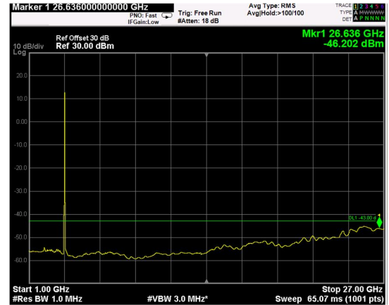
Channel: TOP, Modulation: 64QAM, BW=20MHz, Range: 1GHz - 27GHz
