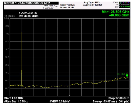
Channel: BOTTOM, Modulation: 256QAM, BW=20MHz, Range: 1GHz - 27GHz
