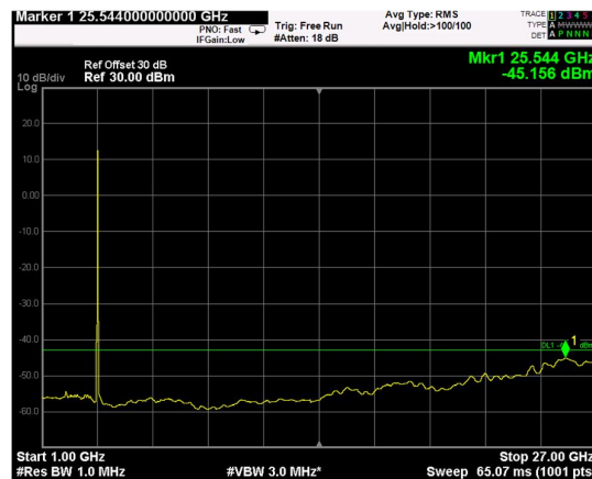
Channel: TOP, Modulation: QPSK, BW=10MHz, Range: 1GHz - 27GHz
