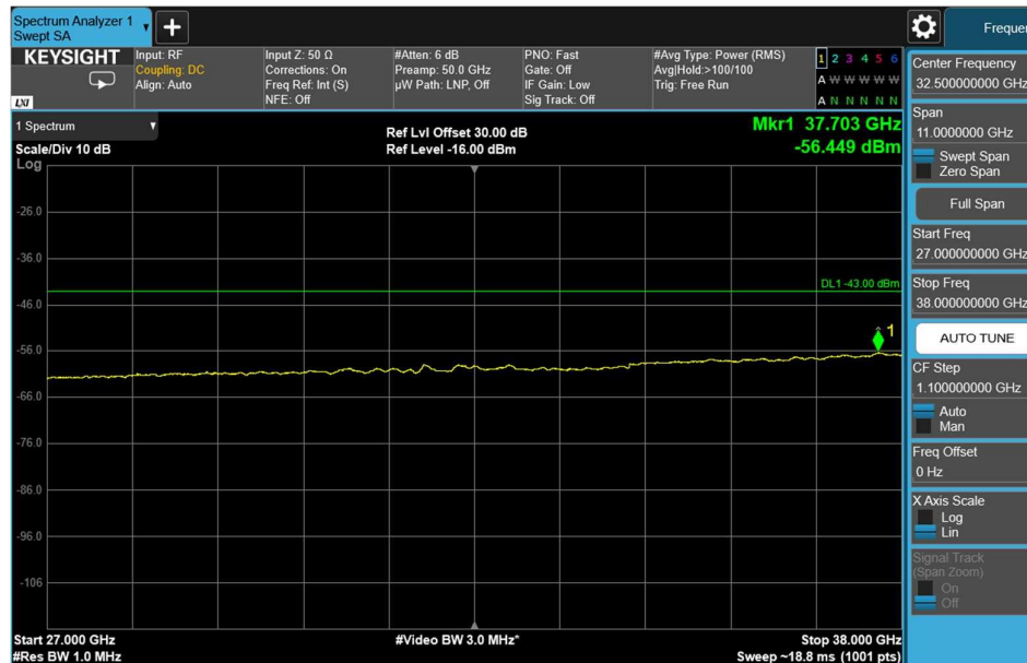
Channel: TOP, Modulation: 64QAM, BW=20MHz, Range: 27GHz - 38GHz
