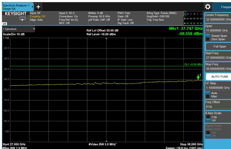
Channel: TOP, Modulation: 256QAM, BW=20MHz, Range: 27GHz - 38GHz
