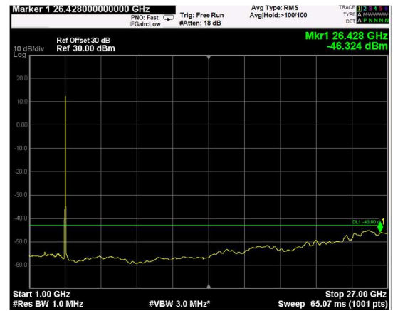
Channel: MIDDLE, Modulation: 64QAM, BW=5MHz, Range: 1GHz - 27GHz
