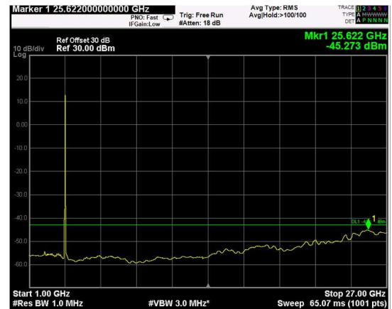
Channel: BOTTOM, Modulation: 256QAM, BW=5MHz, Range: 1GHz - 27GHz
