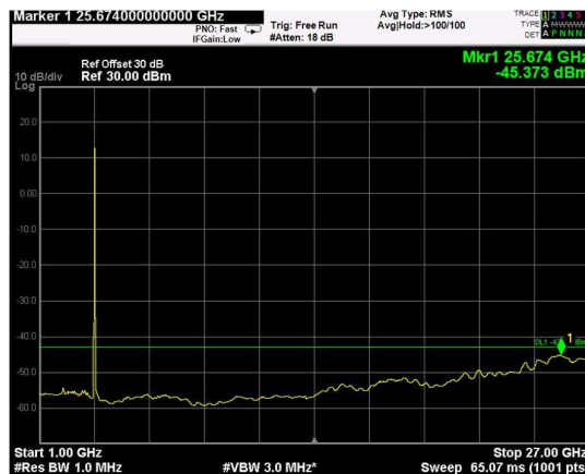
Channel: MIDDLE, Modulation: 256QAM, BW=5MHz, Range: 1GHz - 27GHz
