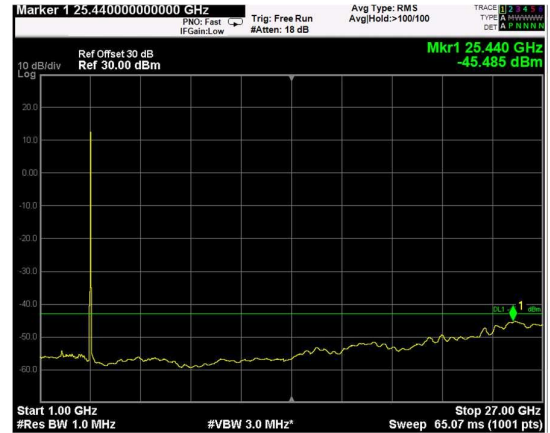
Channel: MIDDLE, Modulation: 256QAM, BW=20MHz, Range: 1GHz - 27GHz
