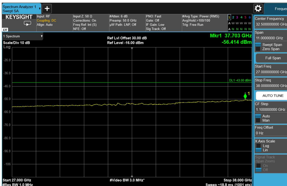
Channel: MIDDLE, Modulation: 64QAM, BW=20MHz, Range: 27GHz - 38GHz
