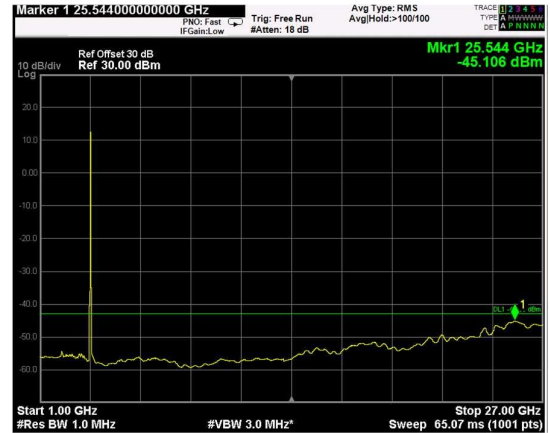
Channel: TOP, Modulation: 16QAM, BW=15MHz, Range: 1GHz - 27GHz
