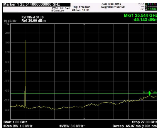
Channel: TOP, Modulation: QPSK, BW=20MHz, Range: 1GHz - 27GHz
