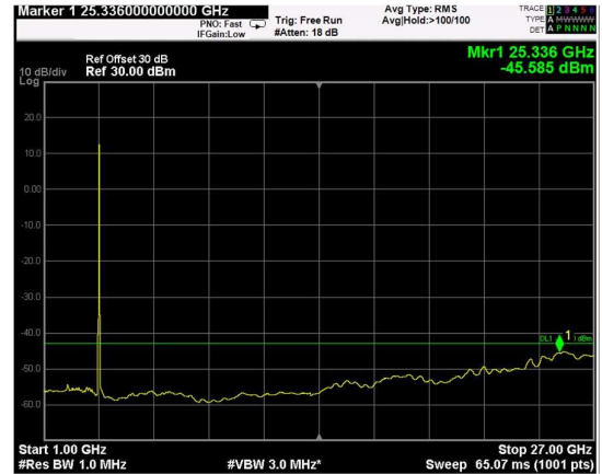
Channel: MIDDLE, Modulation: 64QAM, BW=15MHz, Range: 1GHz - 27GHz
