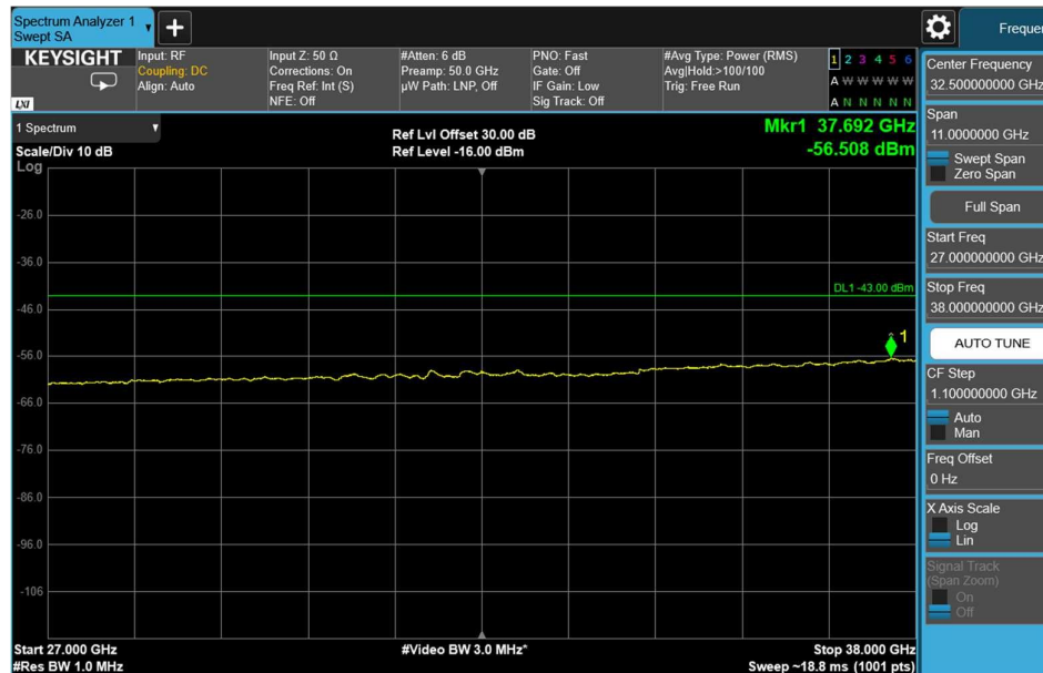
Channel: TOP, Modulation: 16QAM, BW=15MHz, Range: 27GHz - 38GHz
