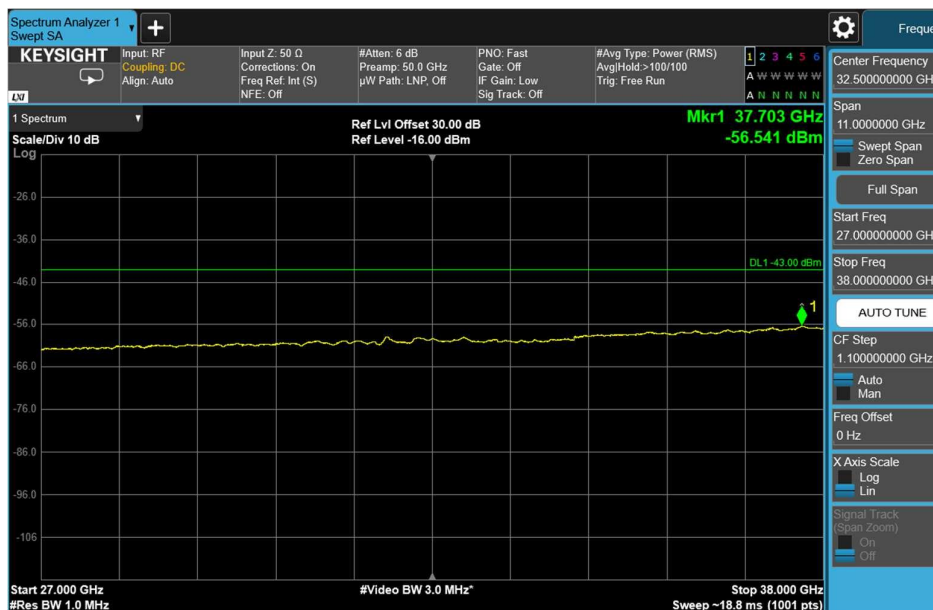
Channel: BOTTOM, Modulation: QPSK, BW=20MHz, Range: 27GHz - 38GHz
