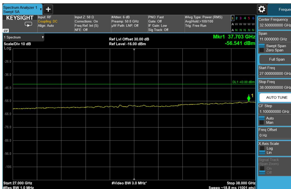
Channel: BOTTOM, Modulation: 64QAM, BW=15MHz, Range: 27GHz - 38GHz
