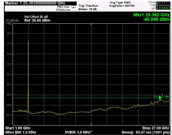
Channel: MIDDLE, Modulation: 16QAM, BW=20MHz, Range: 1GHz - 27GHz
