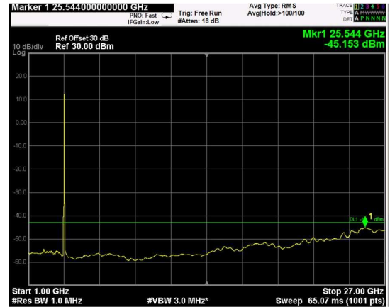
Channel: MIDDLE, Modulation: 256QAM, BW=15MHz, Range: 1GHz - 27GHz
