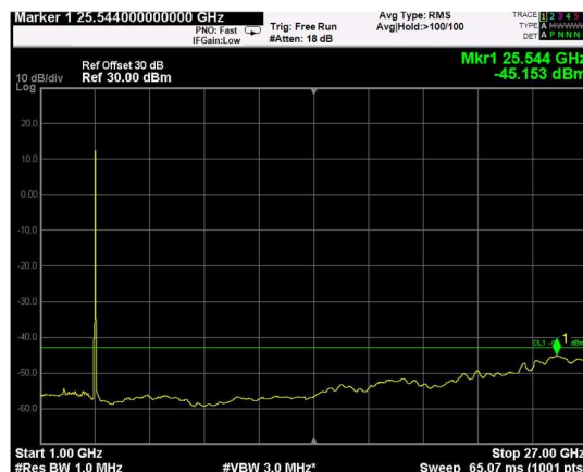
Channel: BOTTOM, Modulation: QPSK, BW=15MHz, Range: 1GHz - 27GHz
