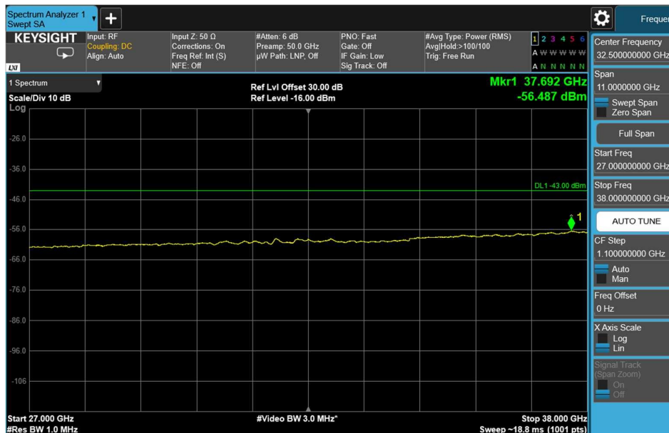
Channel: BOTTOM, Modulation: QPSK, BW=15MHz, Range: 27GHz - 38GHz
