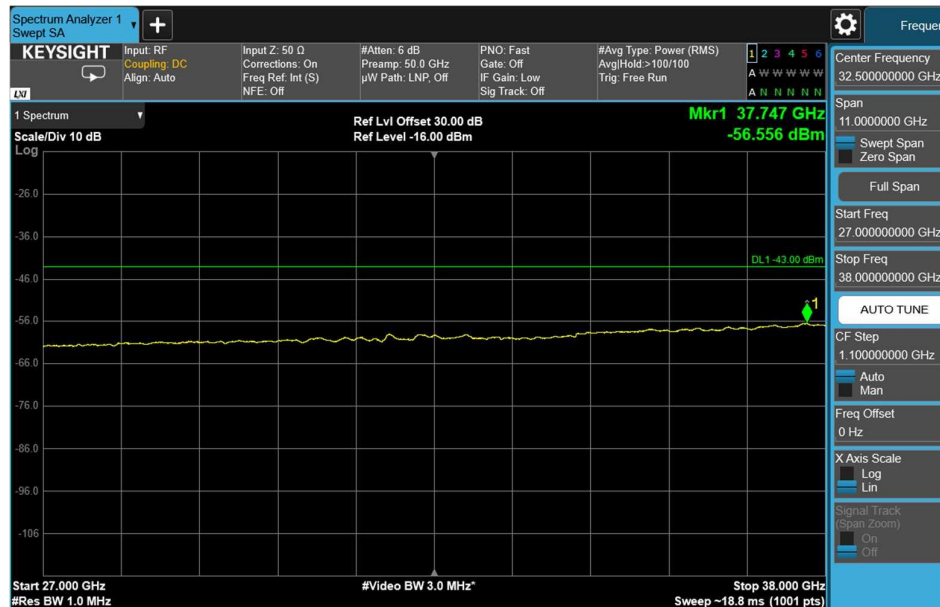
Channel: BOTTOM, Modulation: 256QAM, BW=15MHz, Range: 27GHz - 38GHz
