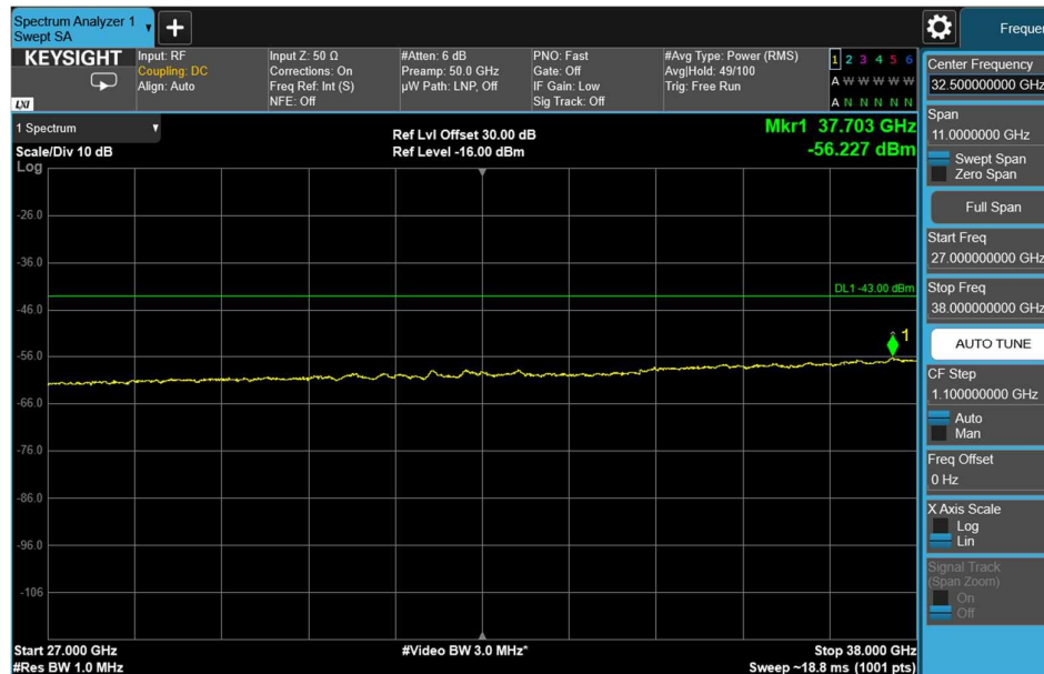
Channel: MIDDLE, Modulation: 16QAM, BW=15MHz, Range: 27GHz - 38GHz
