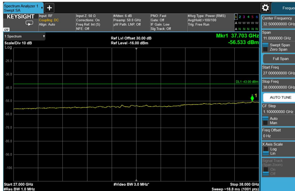
Channel: BOTTOM, Modulation: 16QAM, BW=15MHz, Range: 27GHz - 38GHz
