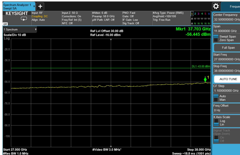
Channel: MIDDLE, Modulation: 64QAM, BW=15MHz, Range: 27GHz - 38GHz
