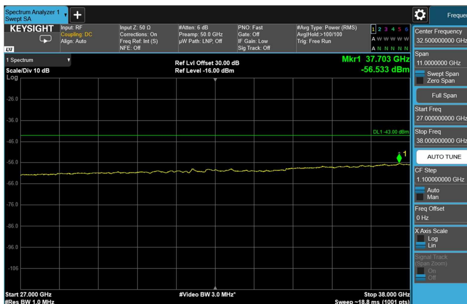
Channel: TOP, Modulation: 256QAM, BW=15MHz, Range: 27GHz - 38GHz
