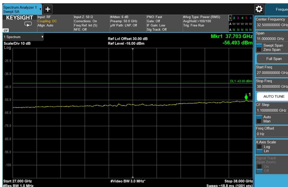
Channel: TOP, Modulation: QPSK, BW=15MHz, Range: 27GHz - 38GHz
