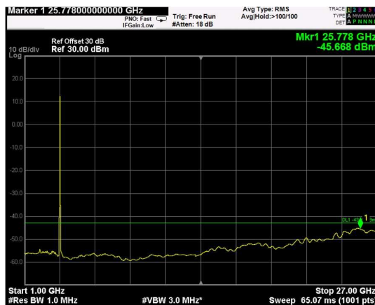
Channel: TOP, Modulation: 64QAM, BW=10MHz, Range: 1GHz - 27GHz
