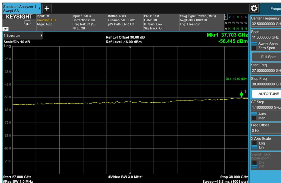
Channel: BOTTOM, Modulation: QPSK, BW=10MHz, Range: 27GHz - 38GHz
