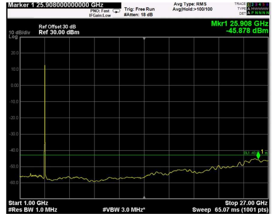
Channel: MIDDLE, Modulation: 256QAM, BW=10MHz, Range: 1GHz - 27GHz
