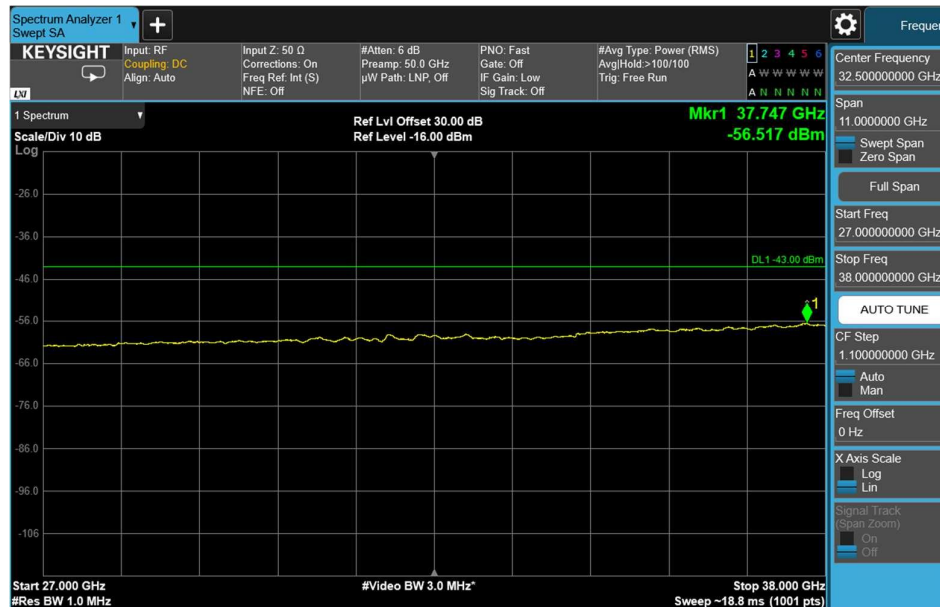
Channel: MIDDLE, Modulation: 256QAM, BW=10MHz, Range: 27GHz - 38GHz
