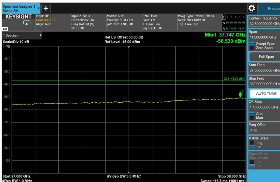
Channel: TOP, Modulation: 64QAM, BW=10MHz, Range: 27GHz - 38GHz
