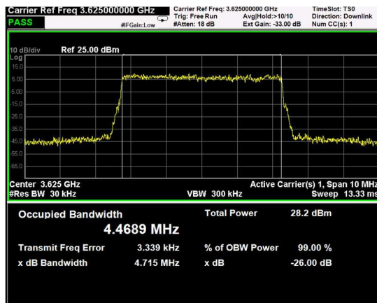
Channel: MIDDLE, Modulation: 16QAM, BW=5MHz
