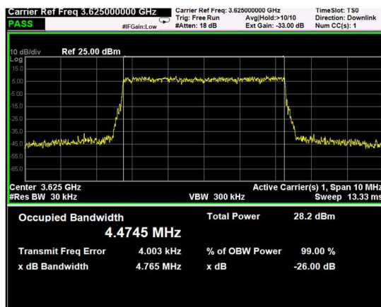
Channel: MIDDLE, Modulation: 256QAM, BW=5MHz
