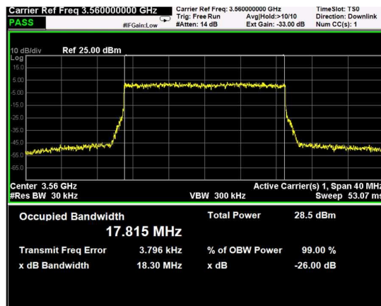
Channel: BOTTOM, Modulation: 16QAM, BW=20MHz
