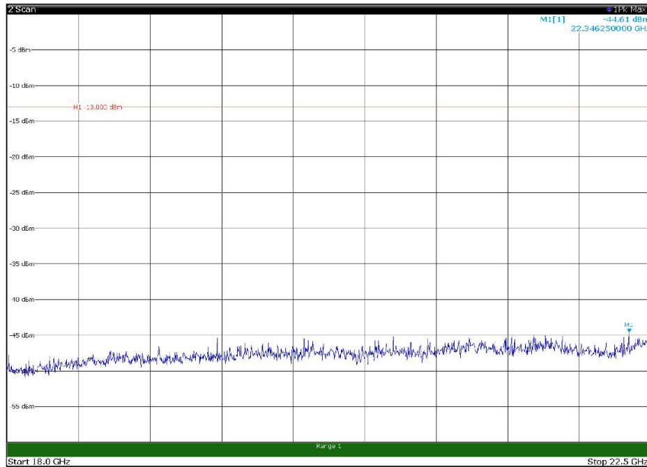
Channel: TOP, Modulation: 64QAM, BW=15MHz, Range: 18GHz - 22.5GHz, Polarization: Horizontal
