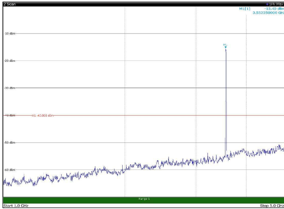
Channel: BOTTOM, Modulation: 64QAM, BW=20MHz, Range: 1GHz - 5GHz, Polarization: Horizontal
