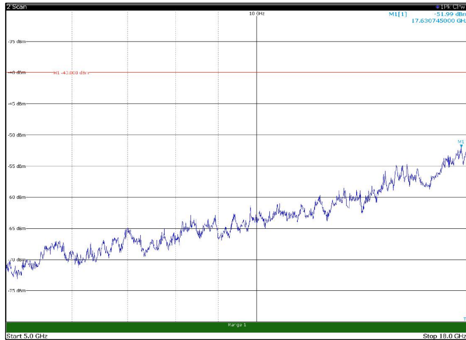
Channel: MIDDLE, Modulation: 64QAM, BW=20MHz, Range: 5GHz - 18GHz, Polarization: Horizontal
