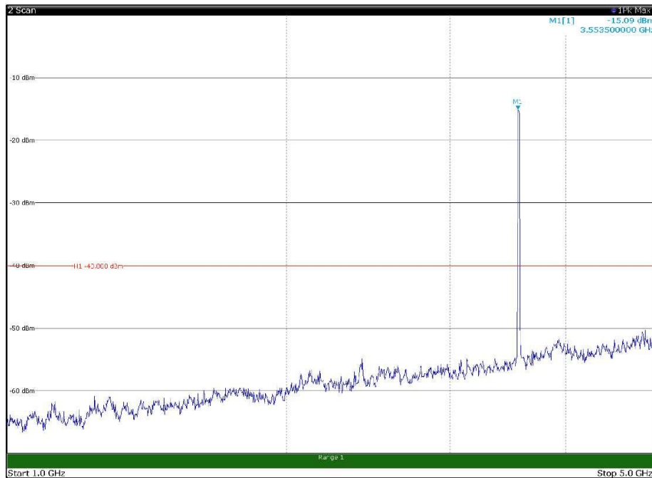
Channel: BOTTOM, Modulation: 64QAM, BW=20MHz, Range: 1GHz - 5GHz, Polarization: Vertical
