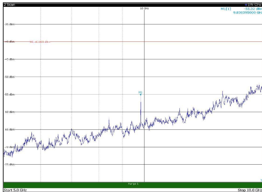
Channel: MIDDLE, Modulation: 64QAM, BW=20MHz, Range: 5GHz - 18GHz, Polarization: Vertical
