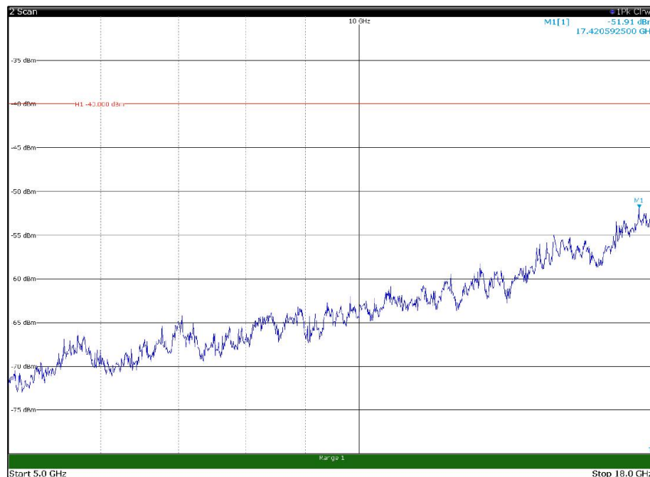
Channel: TOP, Modulation: 16QAM, BW=10MHz, Range: 5GHz - 18GHz, Polarization: Vertical
