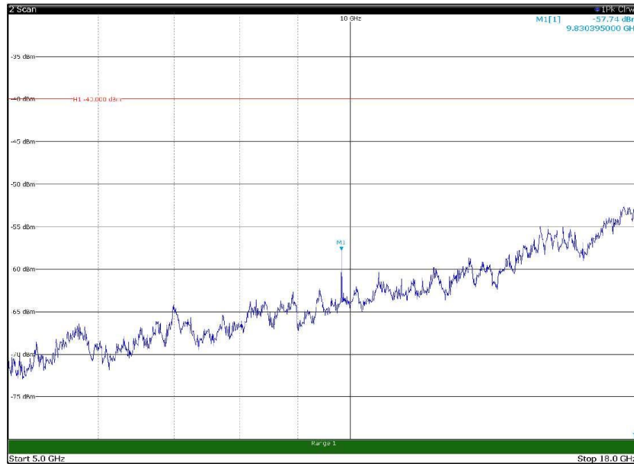
Channel: TOP, Modulation: 16QAM, BW=10MHz, Range: 5GHz - 18GHz, Polarization: Horizontal
