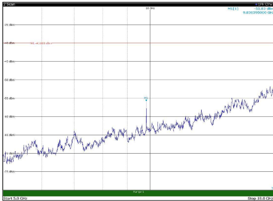
Channel: MIDDLE, Modulation: QPSK, BW=10MHz, Range: 5GHz - 18GHz, Polarization: Vertical
