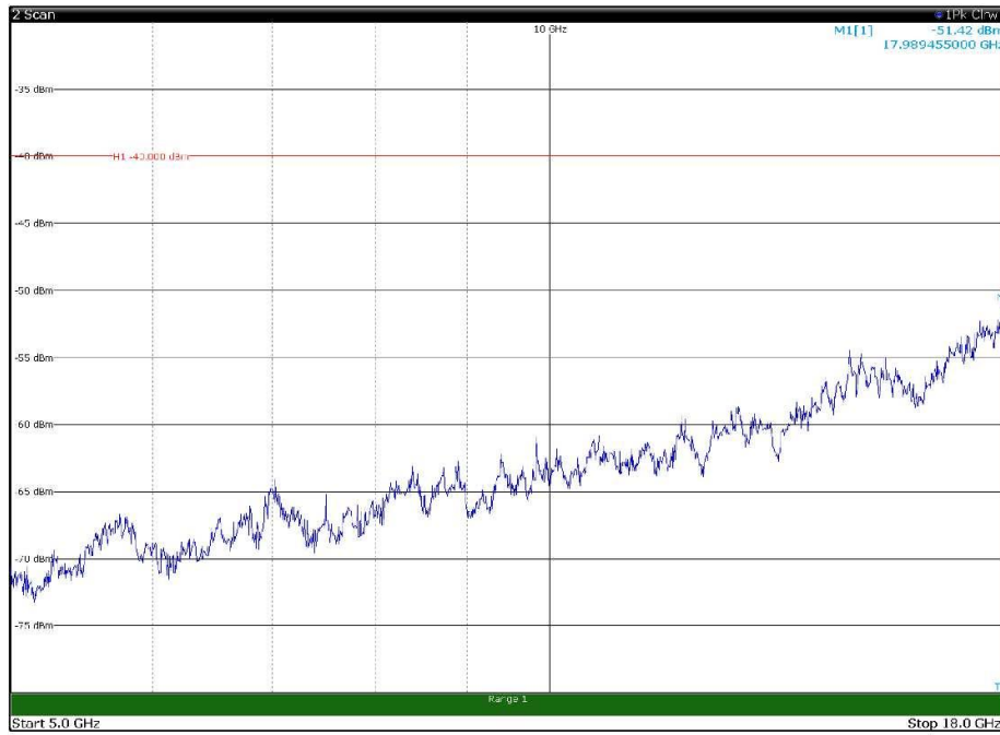
Channel: MIDDLE, Modulation: QPSK, BW=10MHz, Range: 5GHz - 18GHz, Polarization: Horizontal
