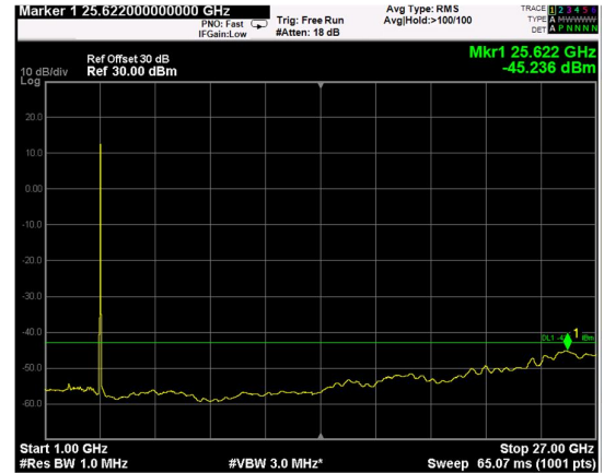
Channel: MIDDLE, Modulation: 64QAM, BW=20MHz, Range: 1GHz - 27GHz
