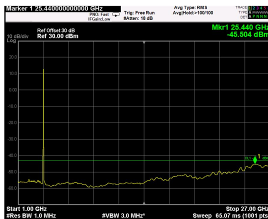
Channel: TOP, Modulation: 16QAM, BW=20MHz, Range: 1GHz - 27GHz
