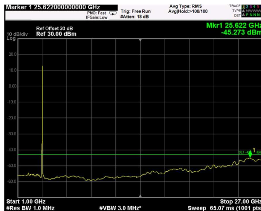
Channel: BOTTOM, Modulation: 256QAM, BW=5MHz, Range: 1GHz - 27GHz
