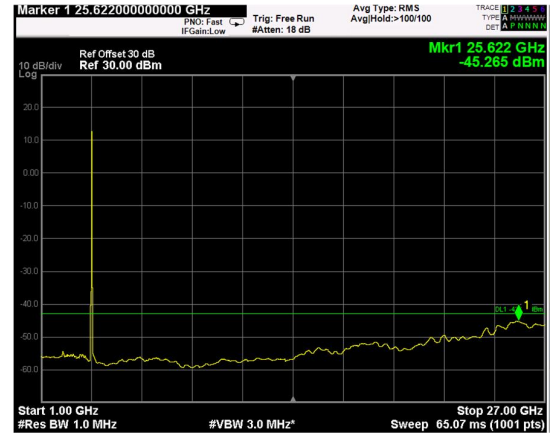
Channel: BOTTOM, Modulation: 16QAM, BW=10MHz, Range: 1GHz - 27GHz
