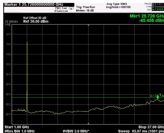
Channel: TOP, Modulation: 64QAM, BW=5MHz, Range: 1GHz - 27GHz
