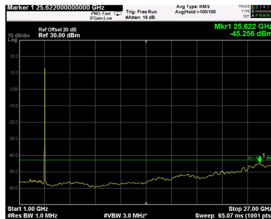
Channel: BOTTOM, Modulation: 256QAM, BW=10MHz, Range: 1GHz - 27GHz
