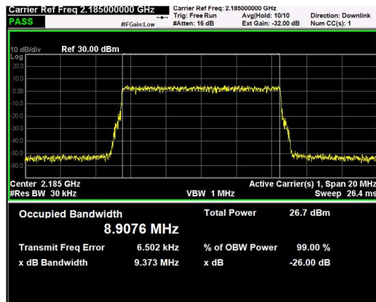
Channel: BOTTOM, Modulation: 256QAM, BW=10MHz
