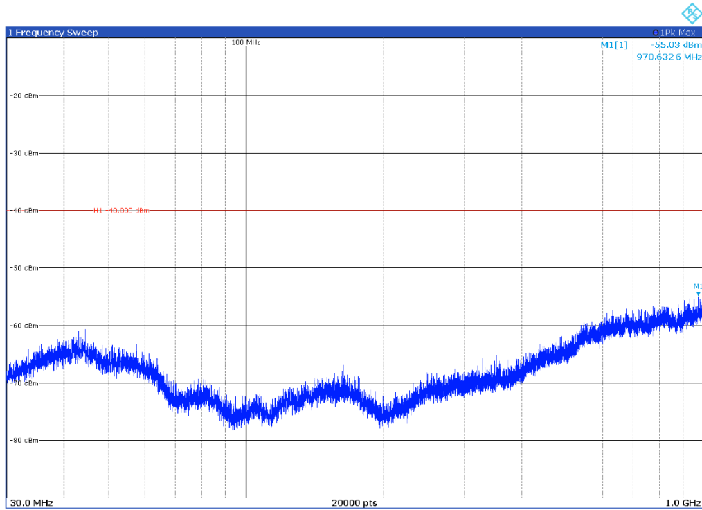
Channel: MIDDLE, Modulation: 64QAM, BW=20 MHz, Range: 30 MHz-1000 MHz, Polarization: Horizontal
