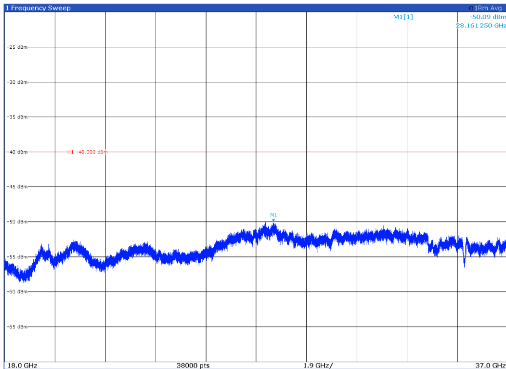
Channel: BOTTOM, Modulation: 64QAM, BW=25 MHz, Range: 18 GHz-37 GHz, Polarization: Vertical
