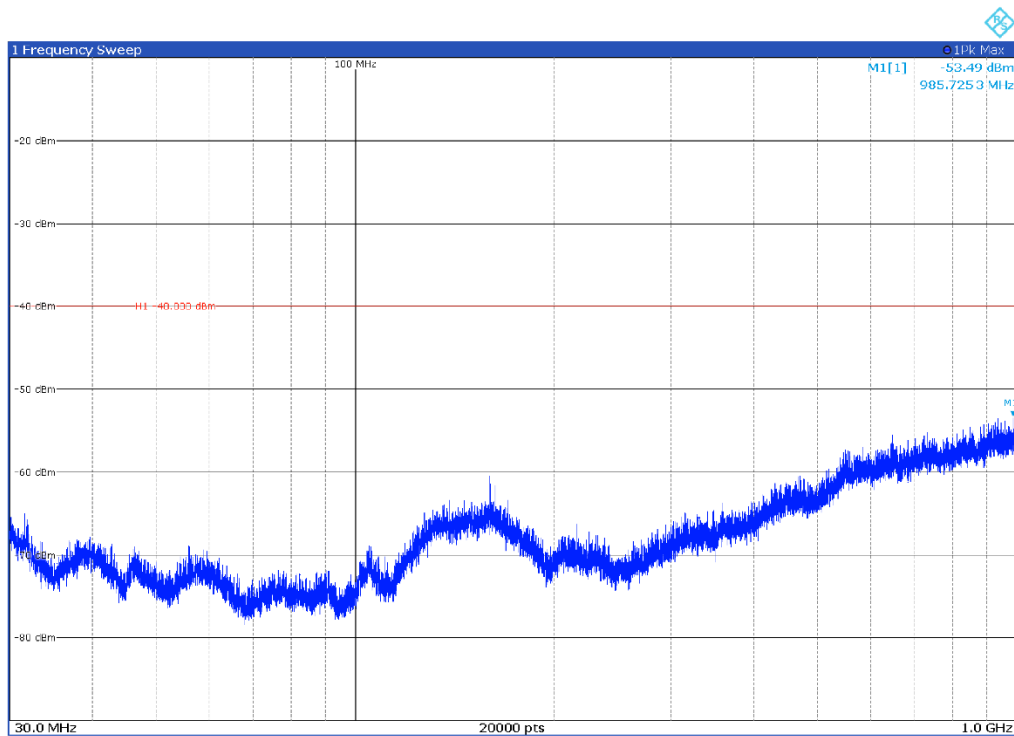
Channel: MIDDLE, Modulation: 64QAM, BW=25 MHz, Range: 30 MHz-1000 MHz, Polarization: Vertical
