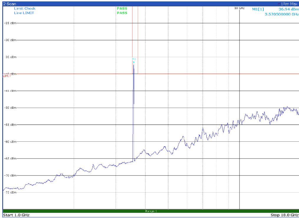
Channel: BOTTOM, Modulation: 64QAM, BW=40 MHz, Range: 1 GHz-18 GHz, Polarization: Horizontal
