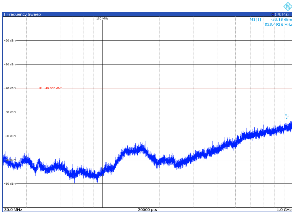
Channel: BOTTOM, Modulation: 64QAM, BW=25 MHz, Range: 30 MHz-1000 MHz, Polarization: Vertical
