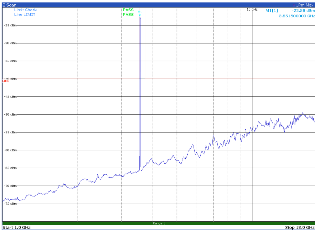
Channel: BOTTOM, Modulation: 64QAM, BW=25 MHz, Range: 1 GHz-18 GHz, Polarization: Vertical
