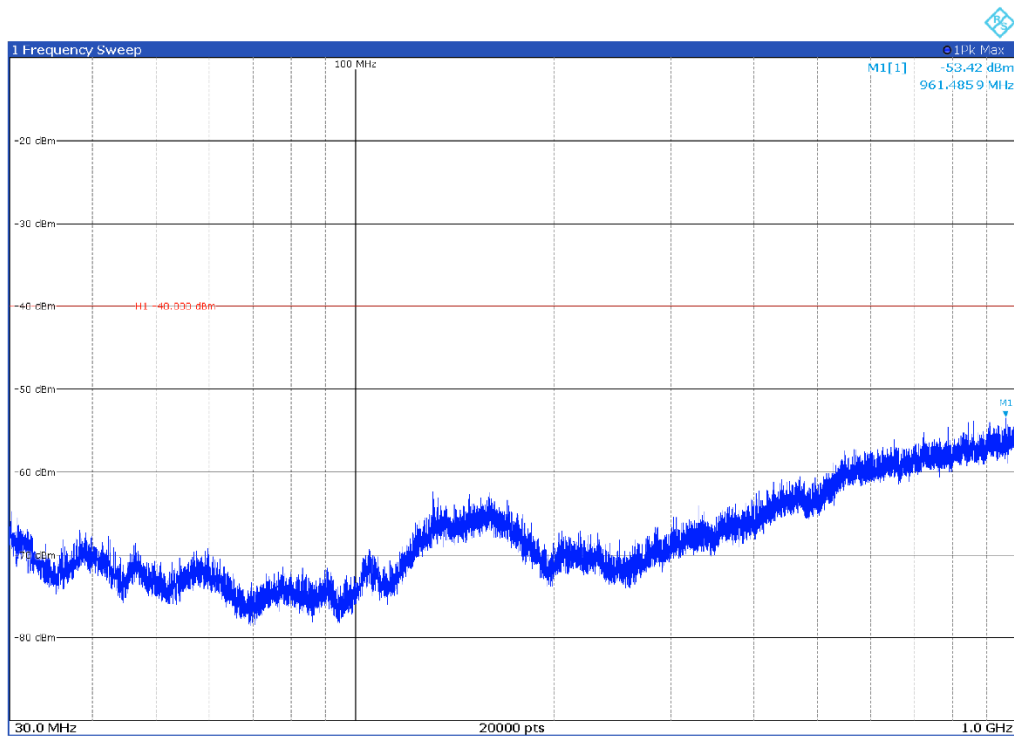
Channel: TOP, Modulation: 64QAM, BW=40 MHz, Range: 30 MHz-1000 MHz, Polarization: Vertical
