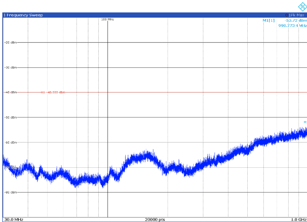
Channel: TOP, Modulation: 64QAM, BW=20 MHz, Range: 30 MHz-1000 MHz, Polarization: Vertical
