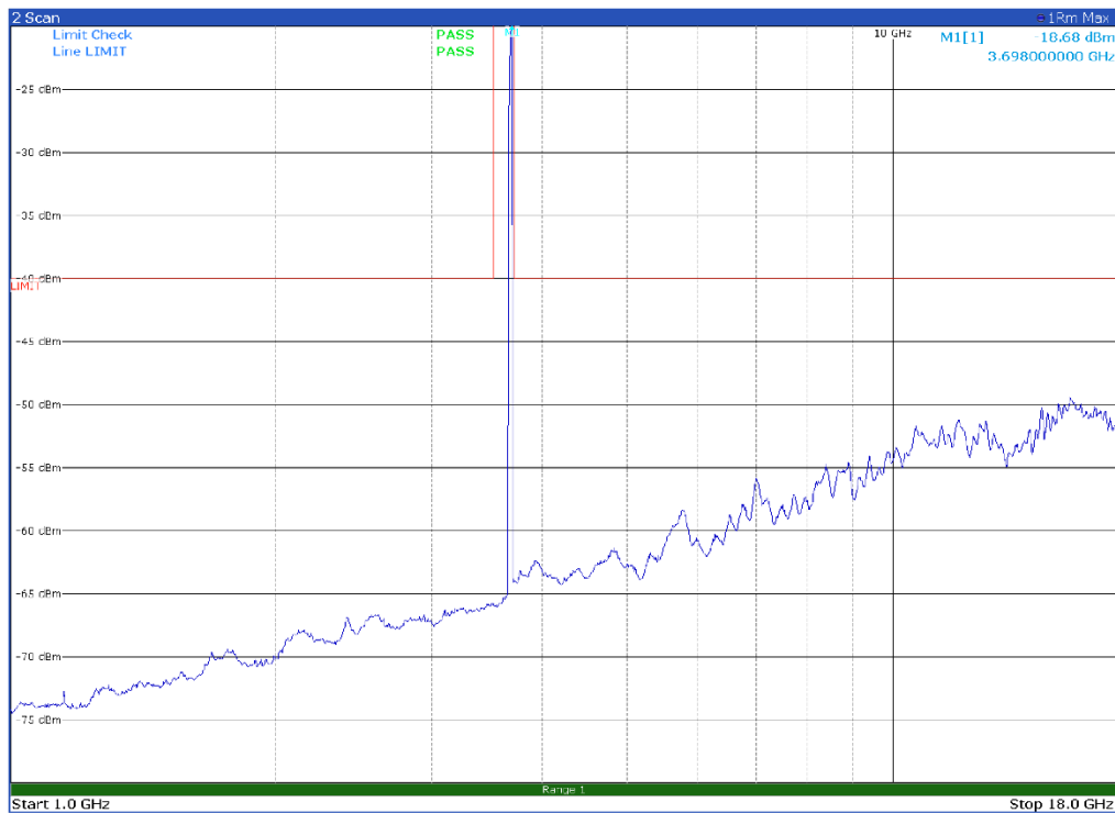
Channel: TOP, Modulation: 64QAM, BW=30 MHz, Range: 1 GHz-18 GHz, Polarization: Vertical
