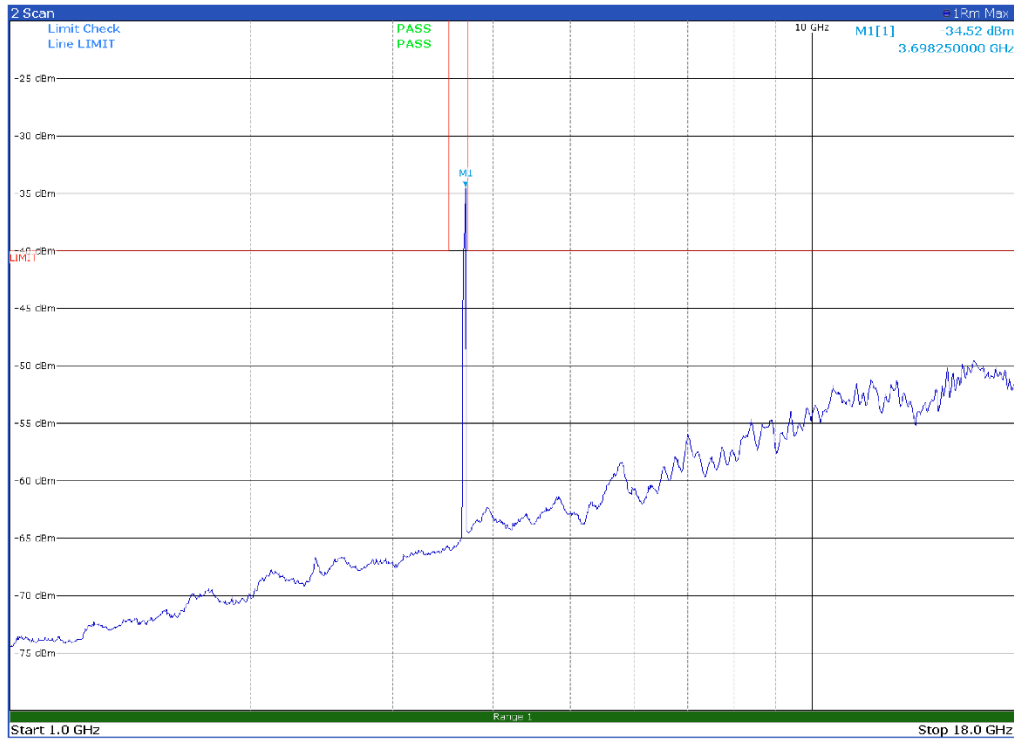
Channel: TOP, Modulation: 64QAM, BW=30 MHz, Range: 1 GHz-18 GHz, Polarization: Horizontal
