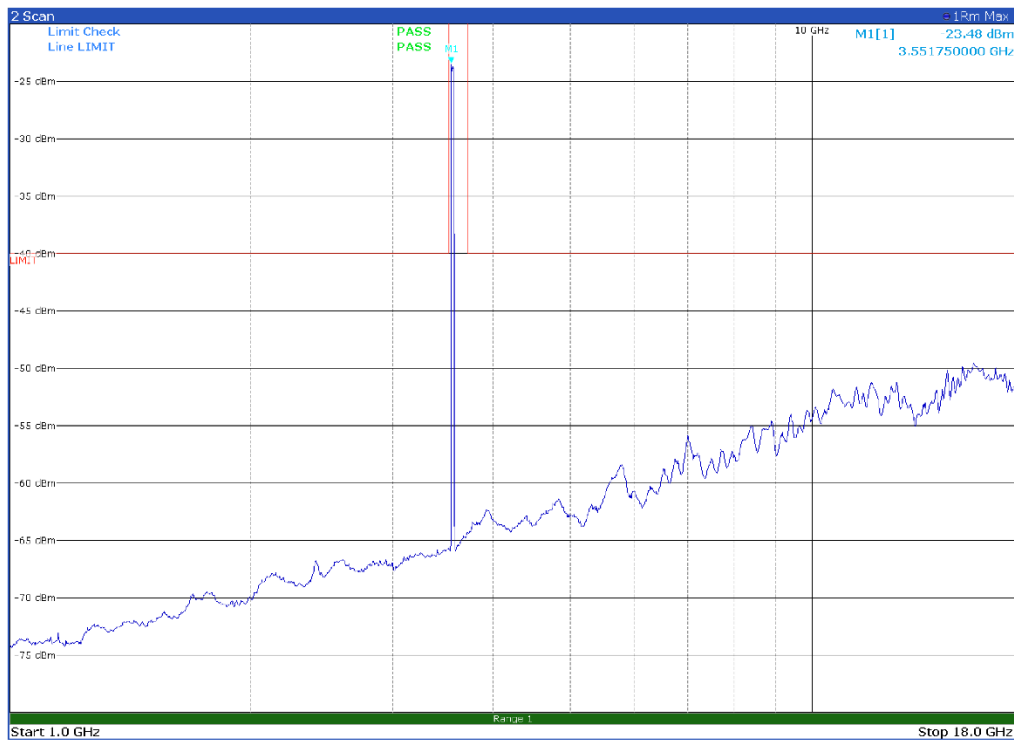
Channel: BOTTOM, Modulation: 64QAM, BW=30 MHz, Range: 1 GHz-18 GHz, Polarization: Vertical
