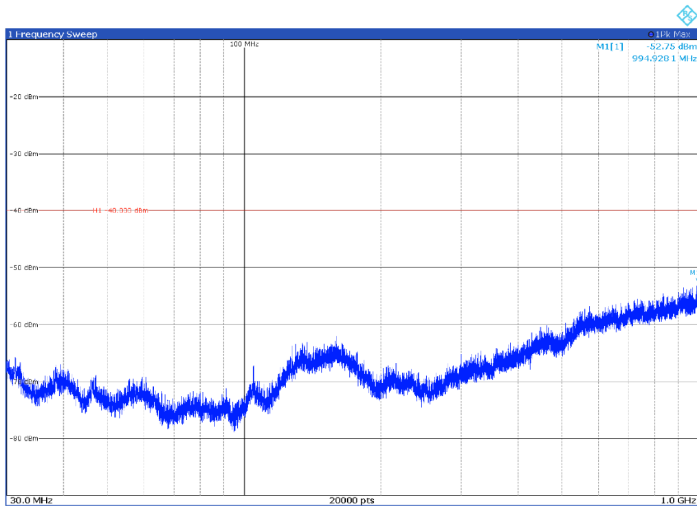
Channel: BOTTOM, Modulation: 64QAM, BW=40 MHz, Range: 30 MHz-1000 MHz, Polarization: Vertical
