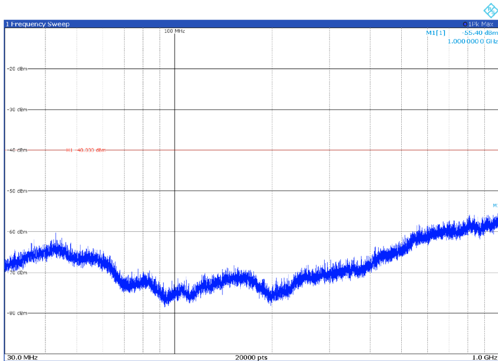
Channel: MIDDLE, Modulation: 64QAM, BW=40 MHz, Range: 30 MHz-1000 MHz, Polarization: Horizontal
