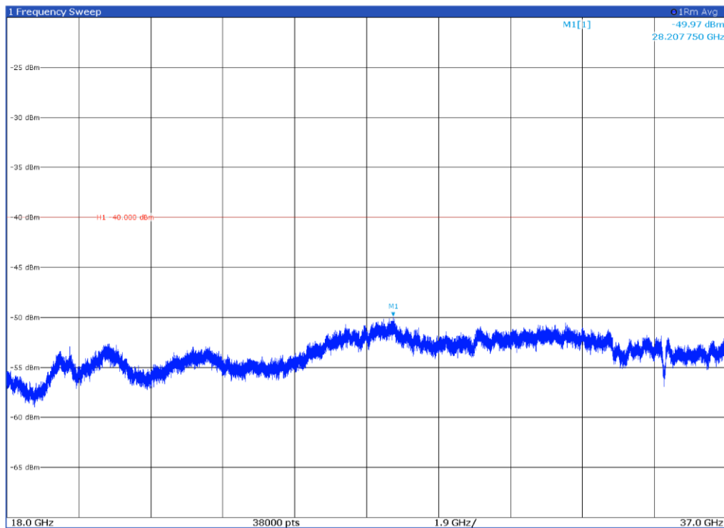
Channel: TOP, Modulation: 64QAM, BW=25 MHz, Range: 18 GHz-37 GHz, Polarization: Vertical
