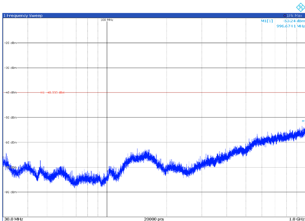
Channel: BOTTOM, Modulation: 64QAM, BW=30 MHz, Range: 30 MHz-1000 MHz, Polarization: Vertical
