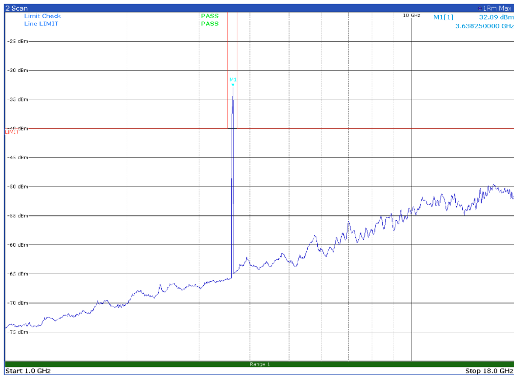
Channel: MIDDLE, Modulation: 64QAM, BW=30 MHz, Range: 1 GHz-18 GHz, Polarization: Vertical
