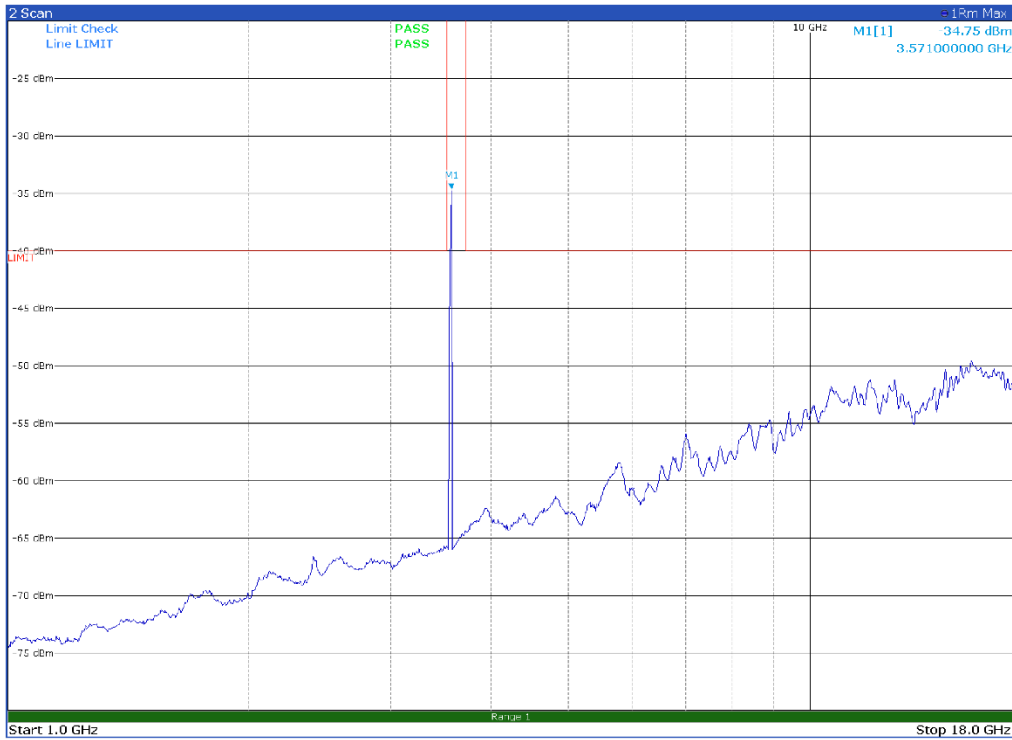
Channel: BOTTOM, Modulation: 64QAM, BW=25 MHz, Range: 1 GHz-18 GHz, Polarization: Horizontal
