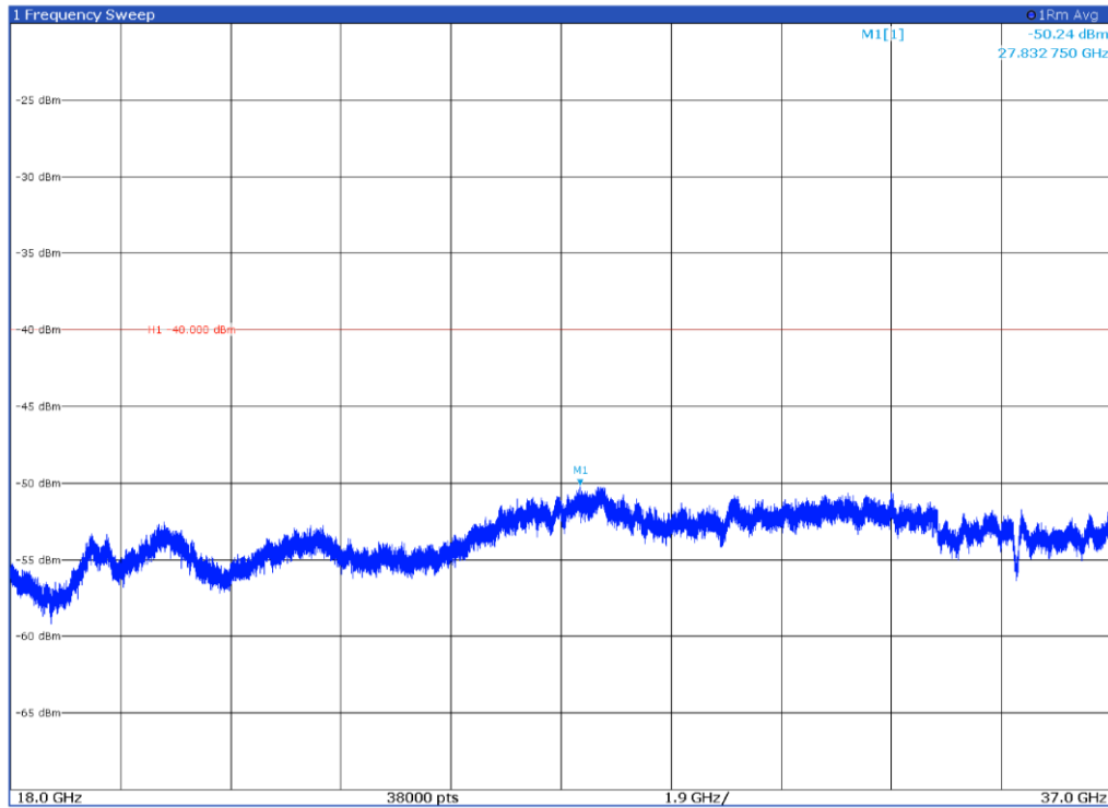
Channel: BOTTOM, Modulation: 64QAM, BW=25 MHz, Range: 18 GHz-37 GHz, Polarization: Horizontal
