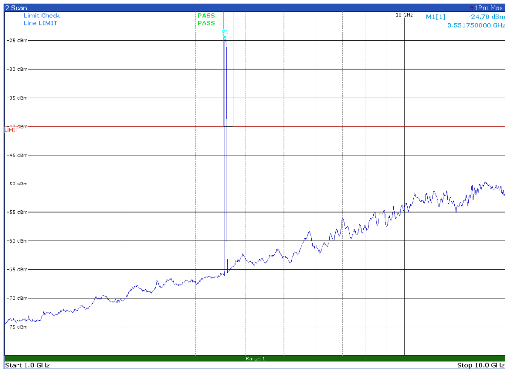
Channel: BOTTOM, Modulation: 64QAM, BW=40 MHz, Range: 1 GHz-18 GHz, Polarization: Vertical
