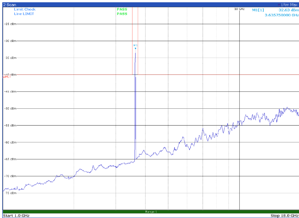
Channel: MIDDLE, Modulation: 64QAM, BW=25 MHz, Range: 1 GHz-18 GHz, Polarization: Vertical
