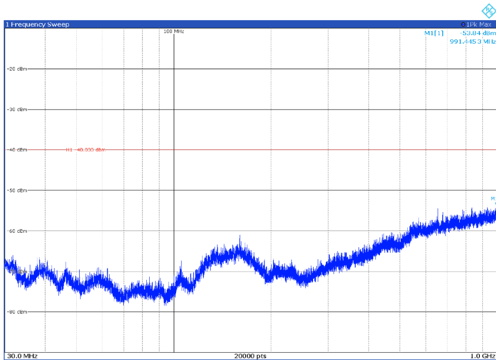
Channel: MIDDLE, Modulation: 64QAM, BW=30 MHz, Range: 30 MHz-1000 MHz, Polarization: Vertical
