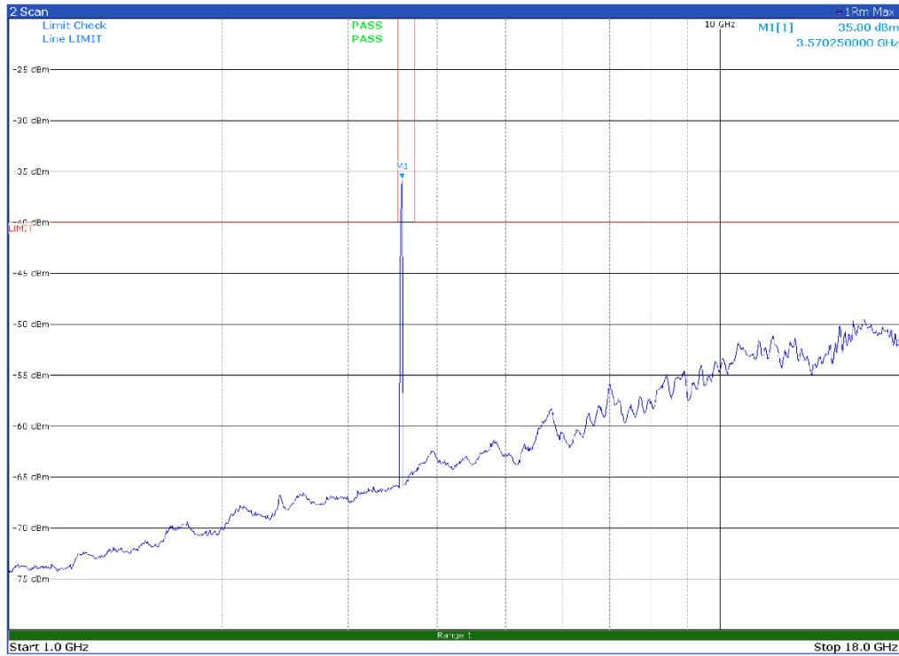
Channel: BOTTOM, Modulation: 64QAM, BW=30 MHz, Range: 1 GHz-18 GHz, Polarization: Horizontal
