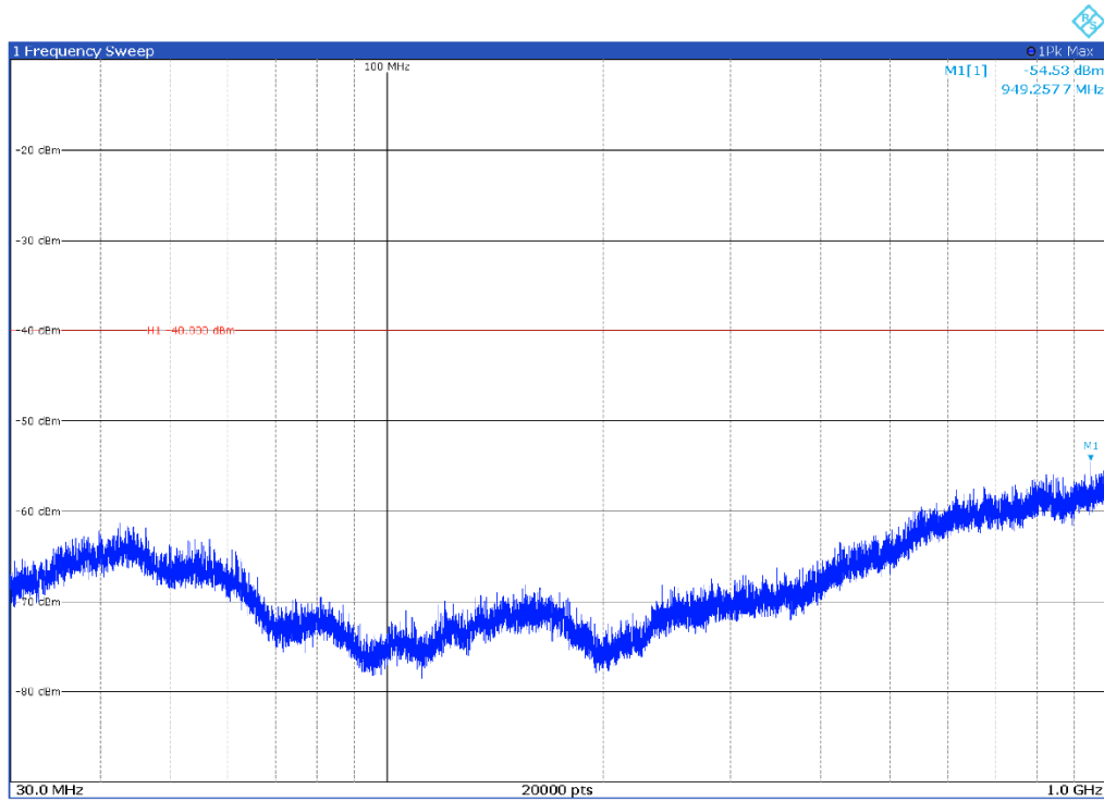
Channel: MIDDLE, Modulation: 64QAM, BW=30 MHz, Range: 30 MHz-1000 MHz, Polarization: Horizontal
