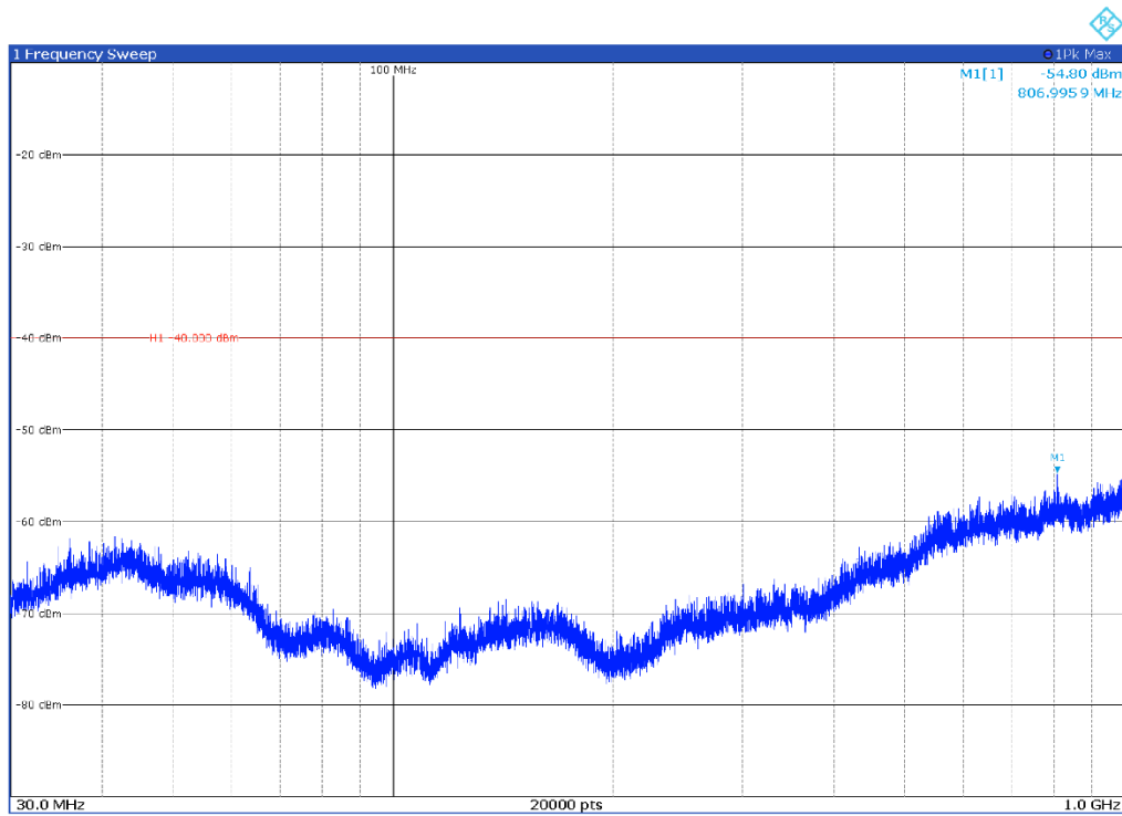
Channel: MIDDLE, Modulation: 64QAM, BW=15 MHz, Range: 30 MHz-1000 MHz, Polarization: Horizontal
