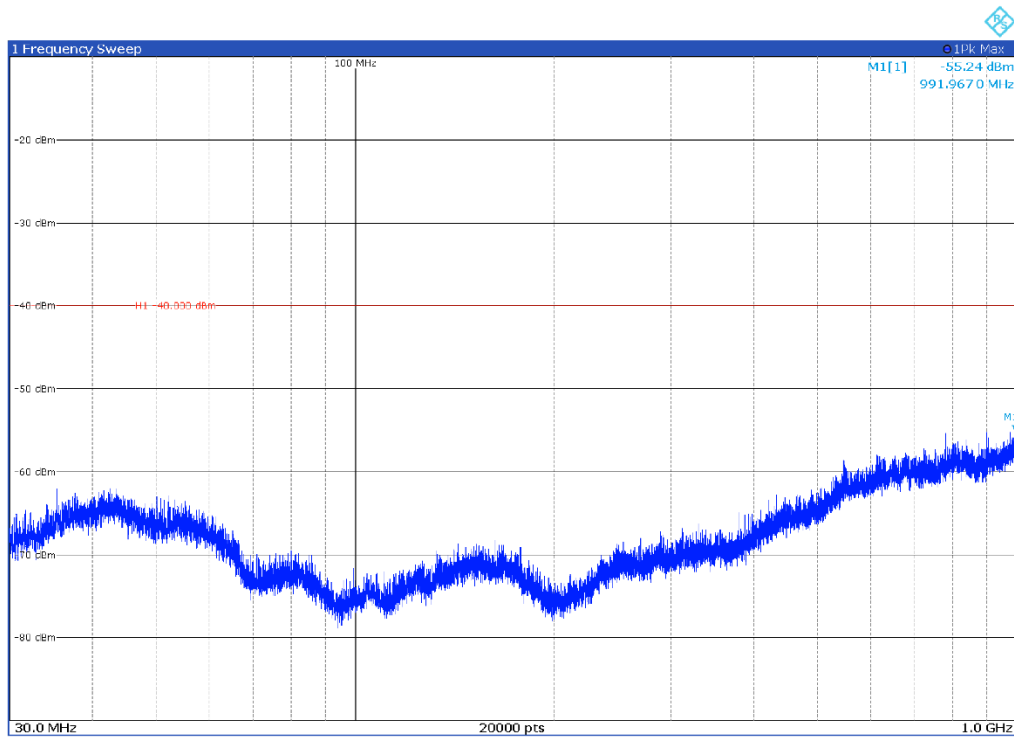
Channel: MIDDLE, Modulation: 64QAM, BW=25 MHz, Range: 30 MHz-1000 MHz, Polarization: Horizontal
