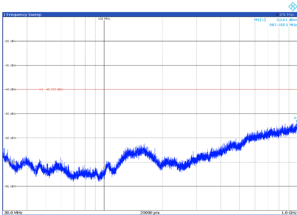
Channel: BOTTOM, Modulation: 64QAM, BW=15 MHz, Range: 30 MHz-1000 MHz, Polarization: Vertical
