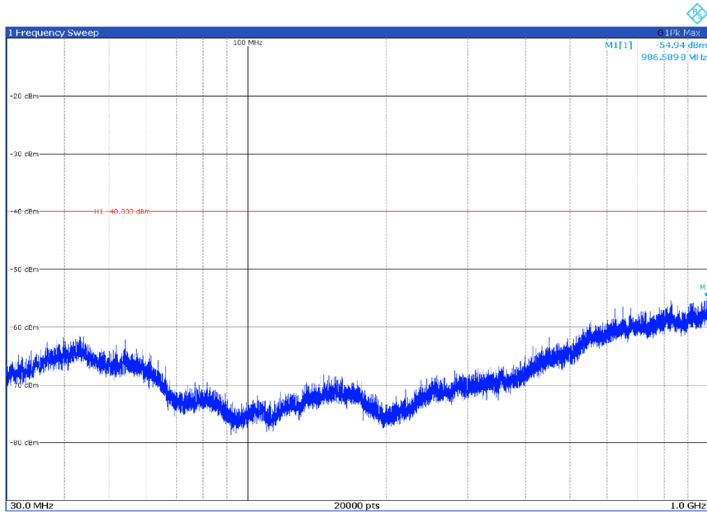
Channel: BOTTOM, Modulation: 64QAM, BW=20 MHz, Range: 30 MHz-1000 MHz, Polarization: Horizontal
