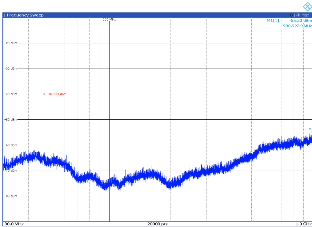
Channel: TOP, Modulation: 64QAM, BW=40 MHz, Range: 30 MHz-1000 MHz, Polarization: Horizontal
