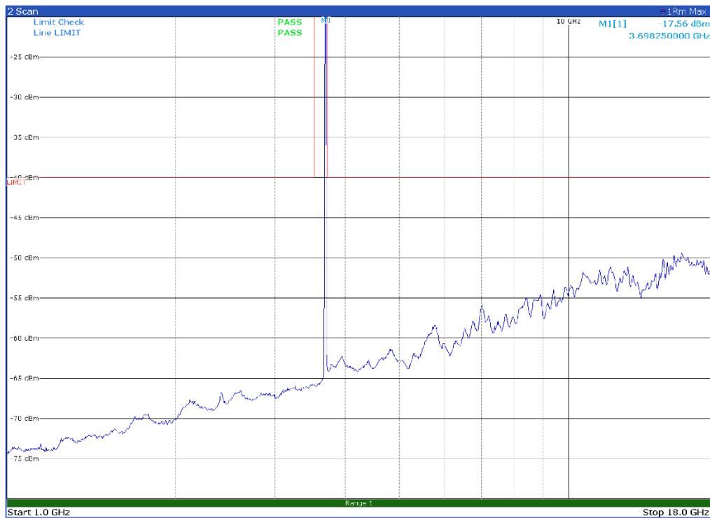
Channel: TOP, Modulation: 64QAM, BW=25 MHz, Range: 1 GHz-18 GHz, Polarization: Vertical
