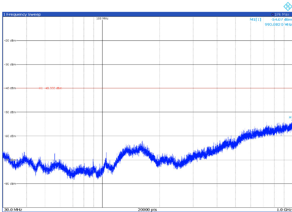
Channel: MIDDLE, Modulation: 64QAM, BW=20 MHz, Range: 30 MHz-1000 MHz, Polarization: Vertical
