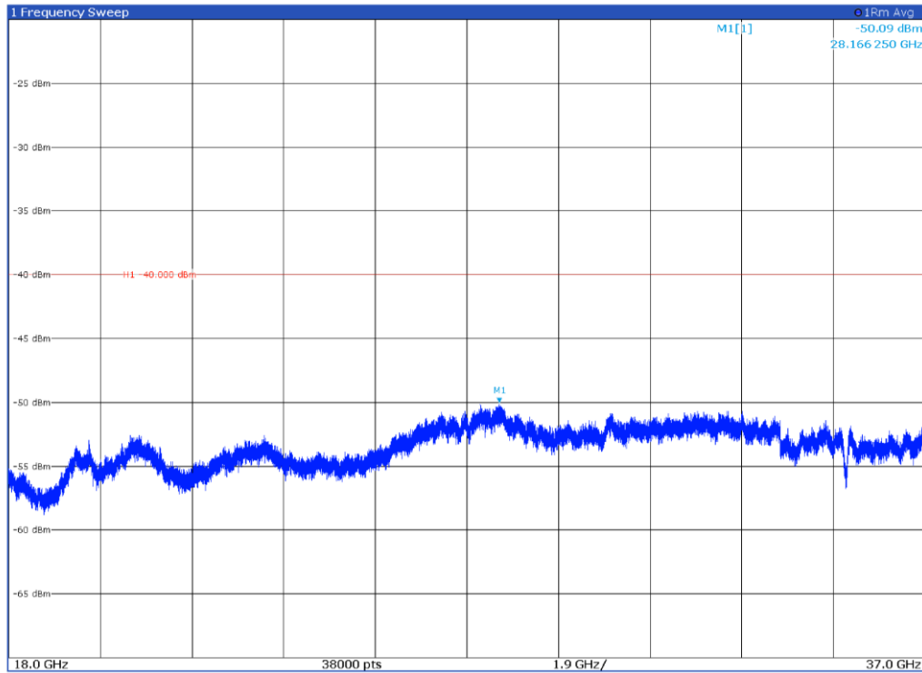
Channel: MIDDLE, Modulation: 64QAM, BW=30 MHz, Range: 18 GHz-37 GHz, Polarization: Horizontal
