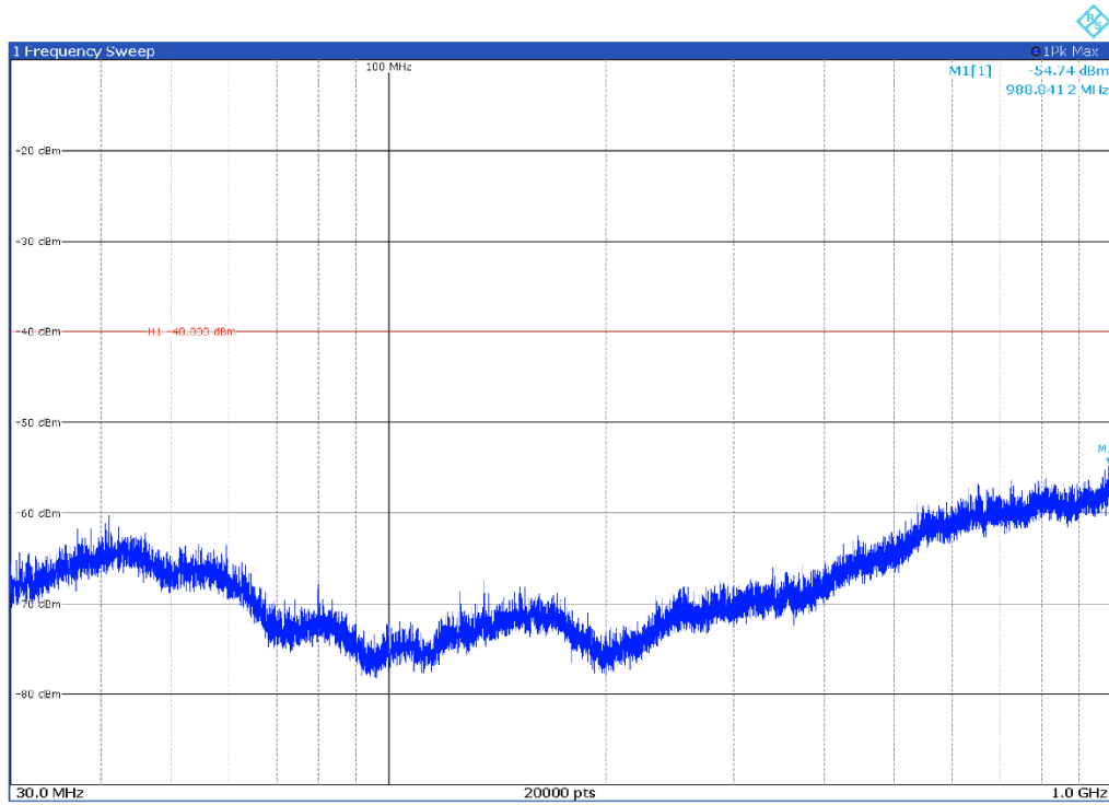
Channel: BOTTOM, Modulation: 64QAM, BW=40 MHz, Range: 30 MHz-1000 MHz, Polarization: Horizontal
