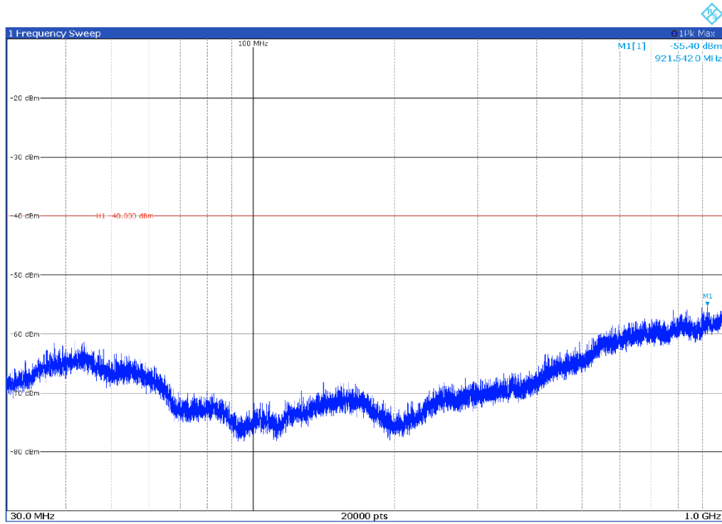
Channel: BOTTOM, Modulation: 64QAM, BW=25 MHz, Range: 30 MHz-1000 MHz, Polarization: Horizontal
