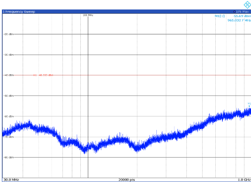
Channel: BOTTOM, Modulation: 64QAM, BW=30 MHz, Range: 30 MHz-1000 MHz, Polarization: Horizontal
