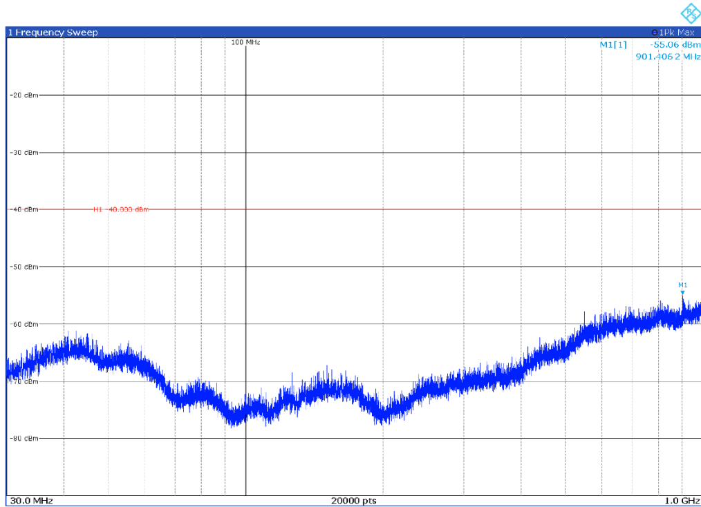
Channel: BOTTOM, Modulation: 64QAM, BW=15 MHz, Range: 30 MHz-1000 MHz, Polarization: Horizontal
