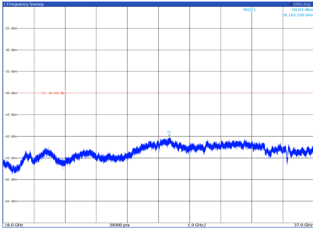
Channel: TOP, Modulation: 64QAM, BW=25 MHz, Range: 18 GHz-37 GHz, Polarization: Horizontal
