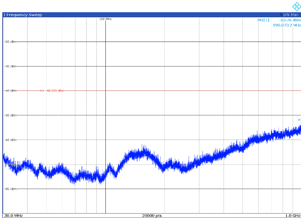
Channel: MIDDLE, Modulation: 64QAM, BW=15 MHz, Range: 30 MHz-1000 MHz, Polarization: Vertical
