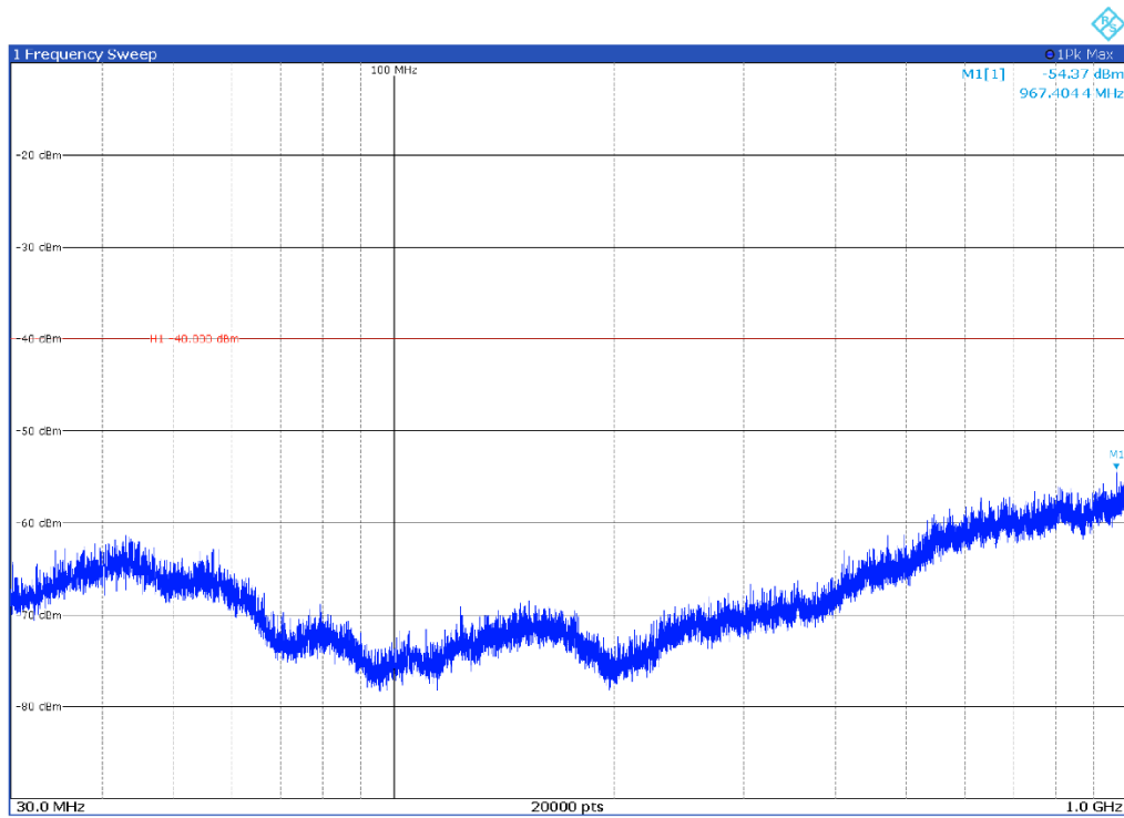
Channel: TOP, Modulation: 64QAM, BW=30 MHz, Range: 30 MHz-1000 MHz, Polarization: Horizontal
