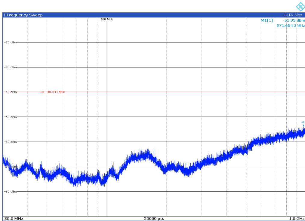
Channel: MIDDLE, Modulation: 64QAM, BW=40 MHz, Range: 30 MHz-1000 MHz, Polarization: Vertical
