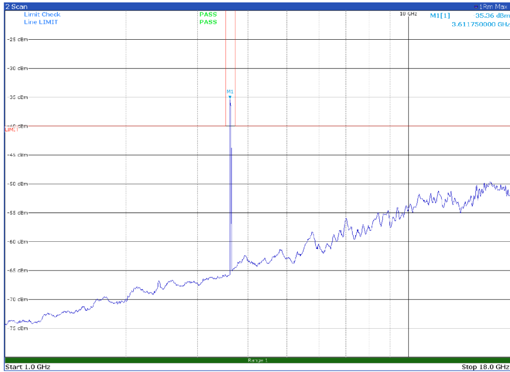
Channel: MIDDLE, Modulation: 64QAM, BW=30 MHz, Range: 1 GHz-18 GHz, Polarization: Horizontal
