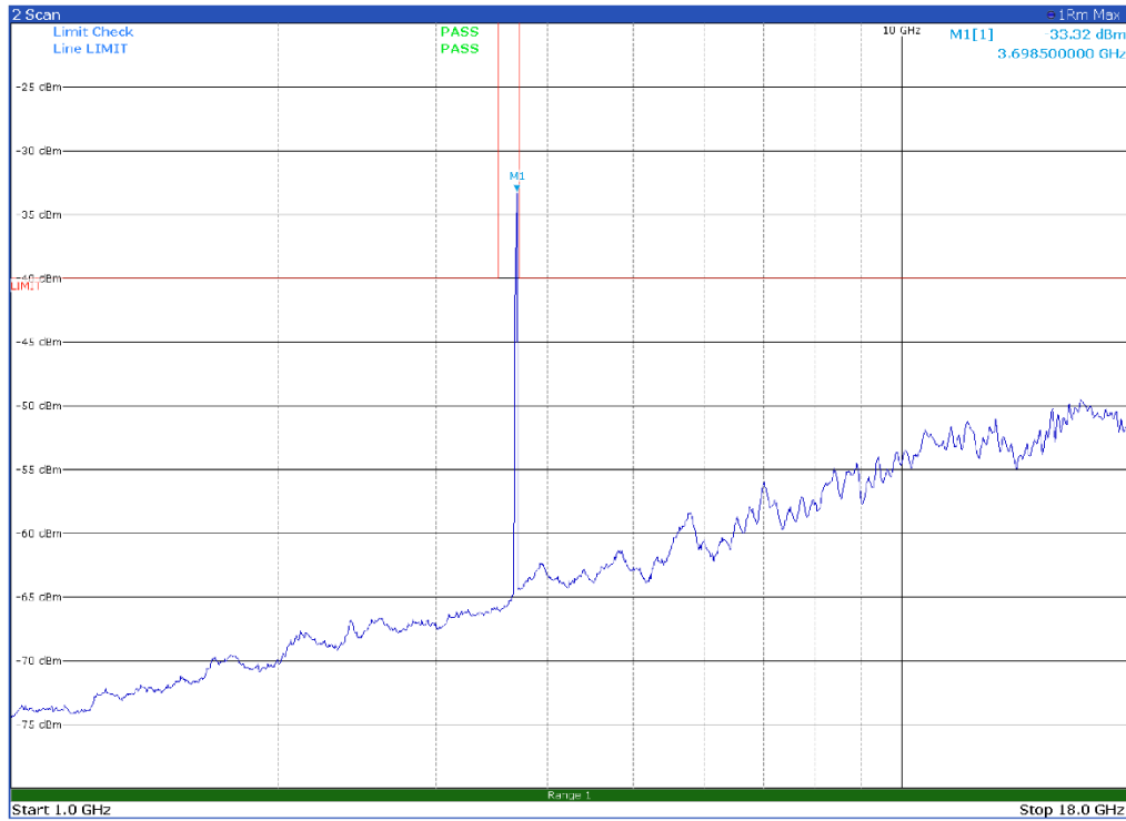
Channel: TOP, Modulation: 64QAM, BW=25 MHz, Range: 1 GHz-18 GHz, Polarization: Horizontal
