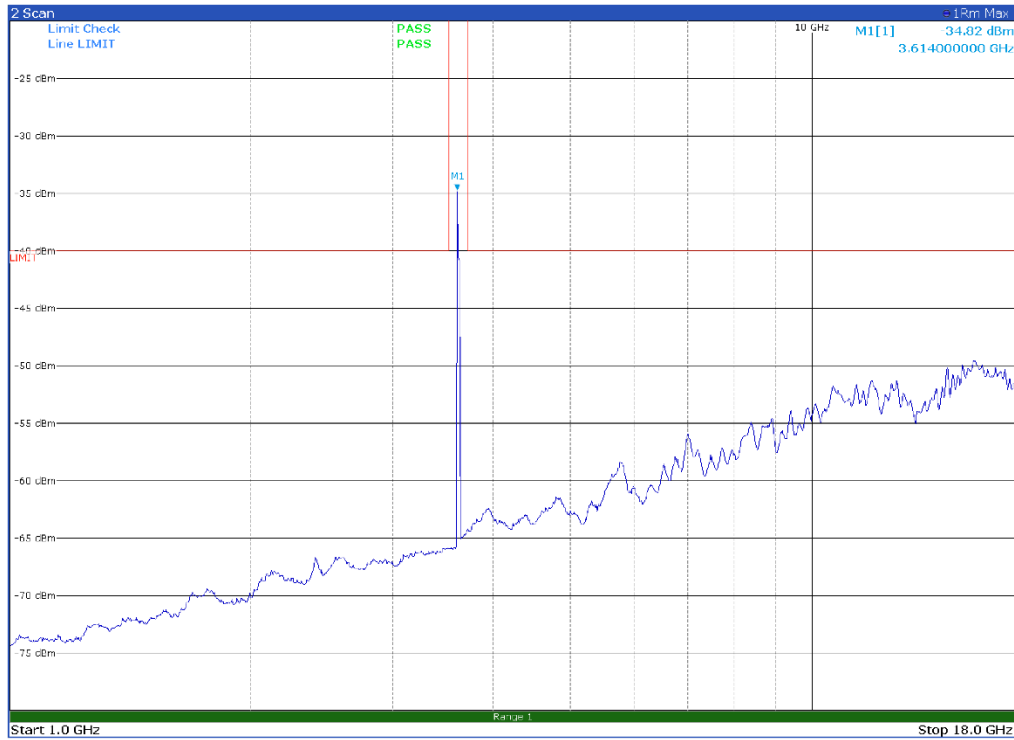
Channel: MIDDLE, Modulation: 64QAM, BW=25 MHz, Range: 1 GHz-18 GHz, Polarization: Horizontal
