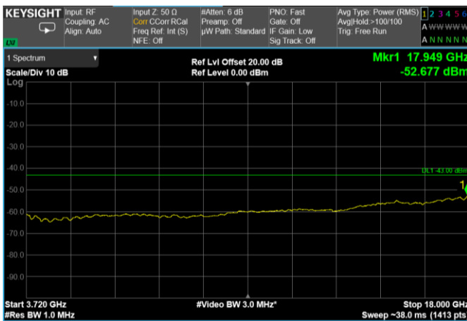
Channel: MIDDLE, Modulation: 64QAM, BW=60MHz, Range: 3720 MHz – 18 GHz
