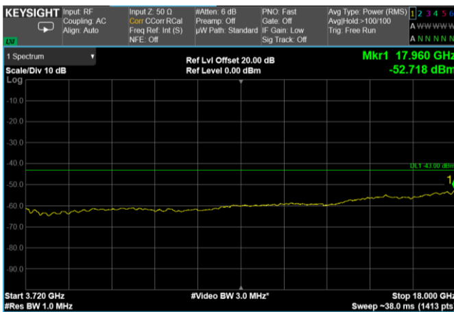
Channel: TOP, Modulation: 64QAM, BW=40MHz, Range: 3720 MHz – 18 GHz
