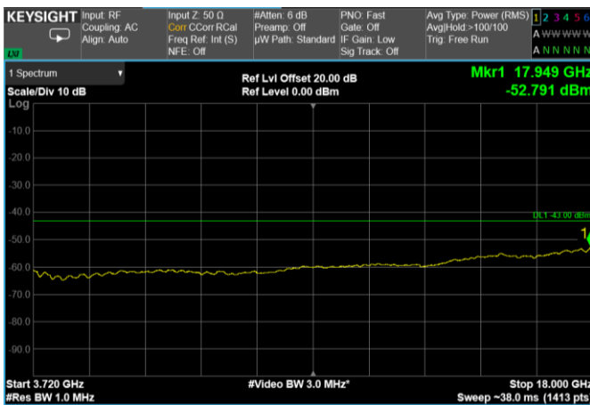
Channel: TOP, Modulation: 64QAM, BW=60MHz, Range: 3720 MHz - 18 GHz
