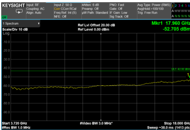
Channel: MIDDLE, Modulation: 64QAM, BW=50MHz, Range: 3720 MHz – 18 GHz
