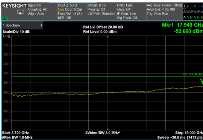
Channel: TOP, Modulation: 64QAM, BW=20MHz, Range: 3720 MHz - 18 GHz
