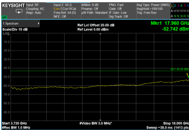
Channel: TOP, Modulation: 64QAM, BW=30MHz, Range: 3720 MHz - 18 GHz
