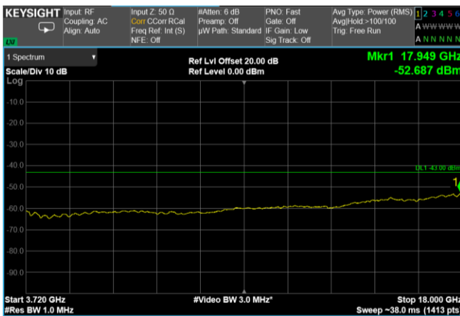
Channel: BOTTOM, Modulation: 64QAM, BW=40MHz, Range: 3720 MHz - 18 GHz
