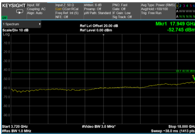
Channel: TOP, Modulation: 64QAM, BW=50MHz, Range: 3720 MHz - 18 GHz
