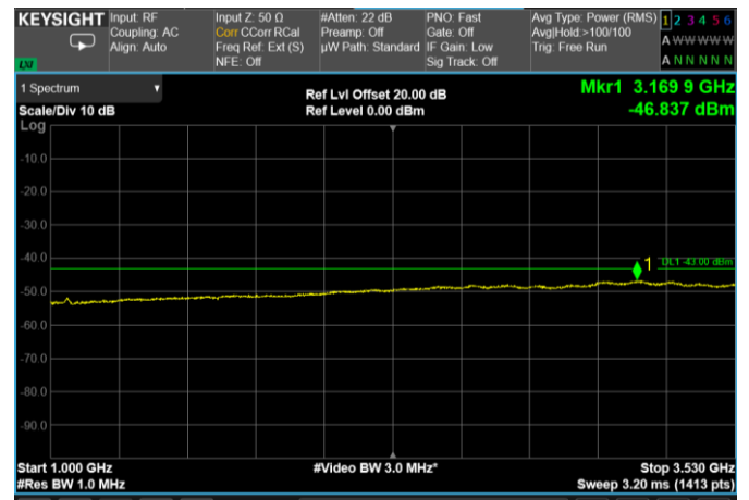
Channel: MIDDLE, Modulation: 64QAM, BW=25MHz, Range: 1000 MHz – 3530 MHz
