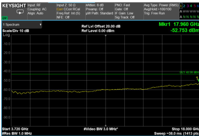
Channel: MIDDLE, Modulation: 64QAM, BW=20MHz, Range: 3720 MHz – 18 GHz
