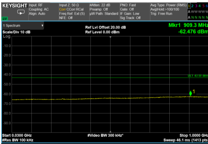
Channel: TOP, Modulation: 64QAM, BW=10MHz, Range: 30 MHz - 1000 MHz
