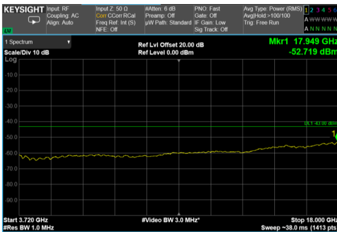
Channel: BOTTOM, Modulation: 64QAM, BW=50MHz, Range: 3720 MHz - 18 GHz
