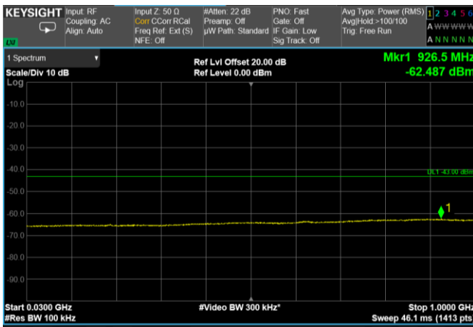
Channel: MIDDLE, Modulation: 64QAM, BW=20MHz, Range: 30 MHz – 1000 MHz
