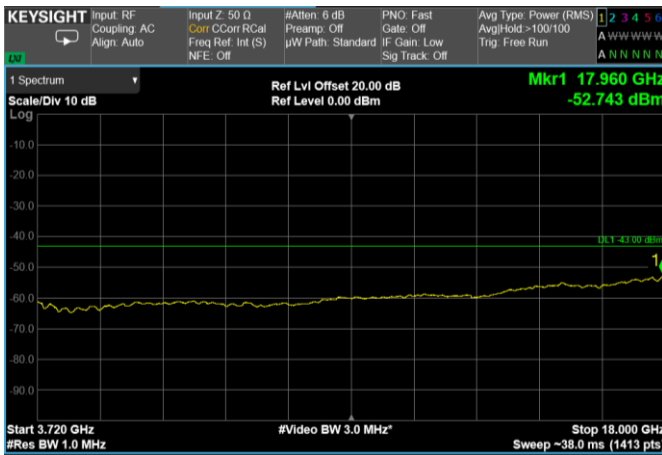
Channel: BOTTOM, Modulation: 64QAM, BW=20MHz, Range: 3720 MHz - 18 GHz
