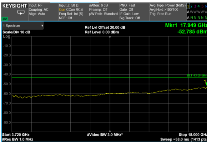
Channel: MIDDLE, Modulation: 64QAM, BW=30MHz, Range: 3720 MHz – 18 GHz
