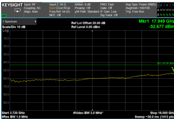
Channel: MIDDLE, Modulation: 64QAM, BW=15MHz, Range: 3720 MHz - 18 GHz
