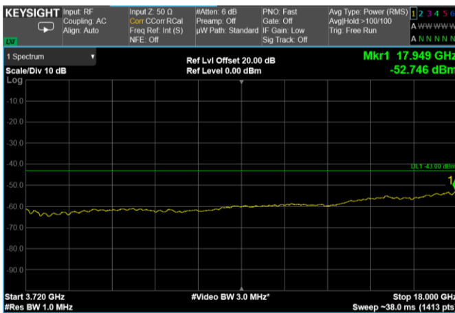
Channel: BOTTOM, Modulation: 64QAM, BW=30MHz, Range: 3720 MHz - 18 GHz
