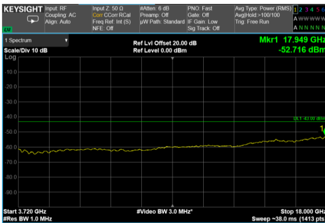
Channel: MIDDLE, Modulation: 64QAM, BW=40MHz, Range: 3720 MHz – 18 GHz
