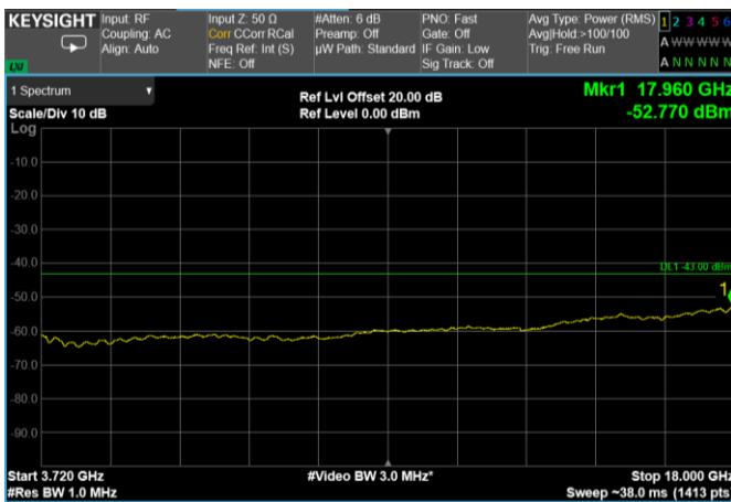
Channel: TOP, Modulation: 64QAM, BW=10MHz, Range: 3720 MHz - 18 GHz
