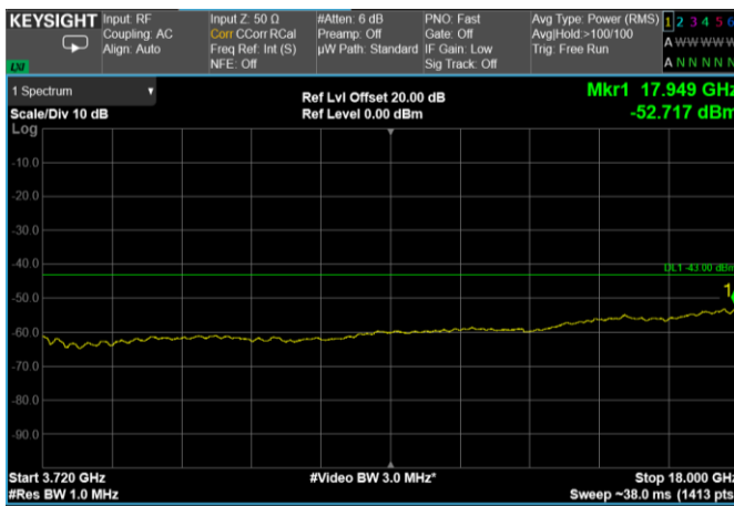
Channel: MIDDLE, Modulation: 64QAM, BW=25MHz, Range: 3720 MHz – 18 GHz
