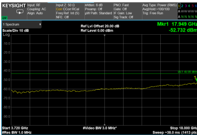
Channel: TOP, Modulation: 64QAM, BW=15MHz, Range: 3720 MHz - 18 GHz
