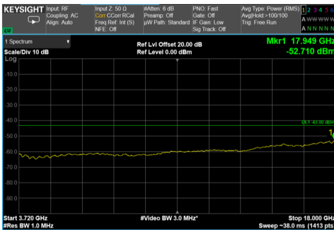
Channel: BOTTOM, Modulation: 64QAM, BW=60MHz, Range: 3720 MHz - 18 GHz
