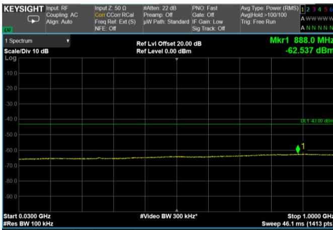
Channel: TOP, Modulation: 64QAM, BW=15MHz, Range: 30 MHz - 1000 MHz
