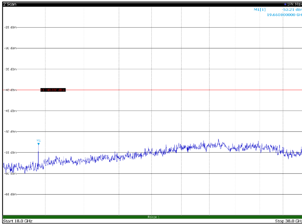
Channel: MIDDLE, Modulation: 64QAM, BW=15MHz, Range: 18GHz - 38GHz, Polarization: Horizontal
