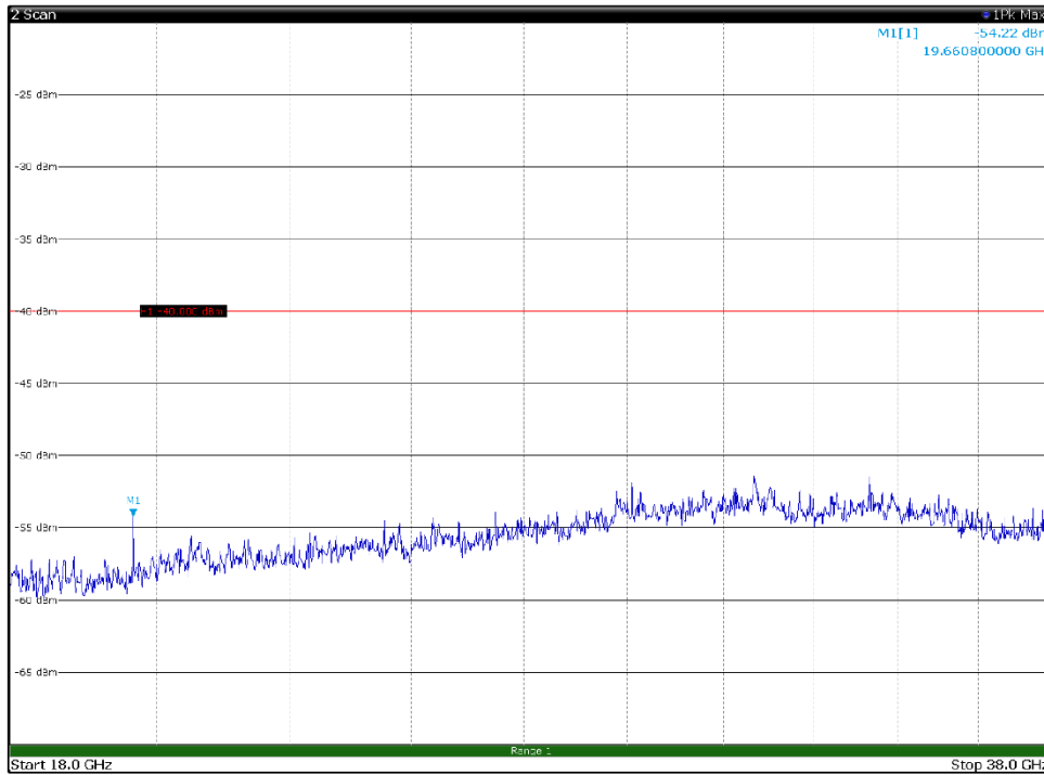
Channel: MIDDLE, Modulation: 256QAM, BW=10MHz, Range: 18GHz - 38GHz, Polarization: Horizontal
