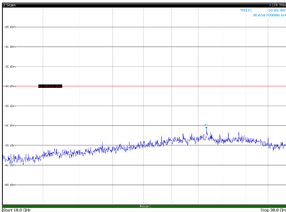
Channel: MIDDLE, Modulation: 256QAM, BW=10MHz, Range: 18GHz - 38GHz, Polarization: Vertical
