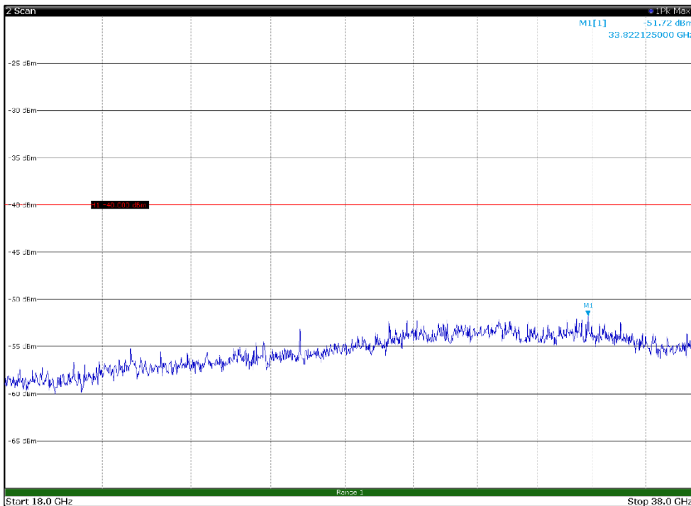
Channel: MIDDLE, Modulation: 16QAM, BW=20MHz, Range: 18GHz - 38GHz, Polarization: Vertical
