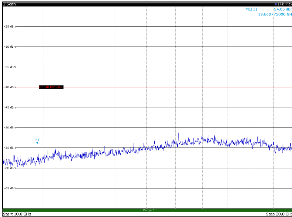
Channel: BOTTOM, Modulation: QPSK, BW=15MHz, Range: 18GHz - 38GHz, Polarization: Horizontal
