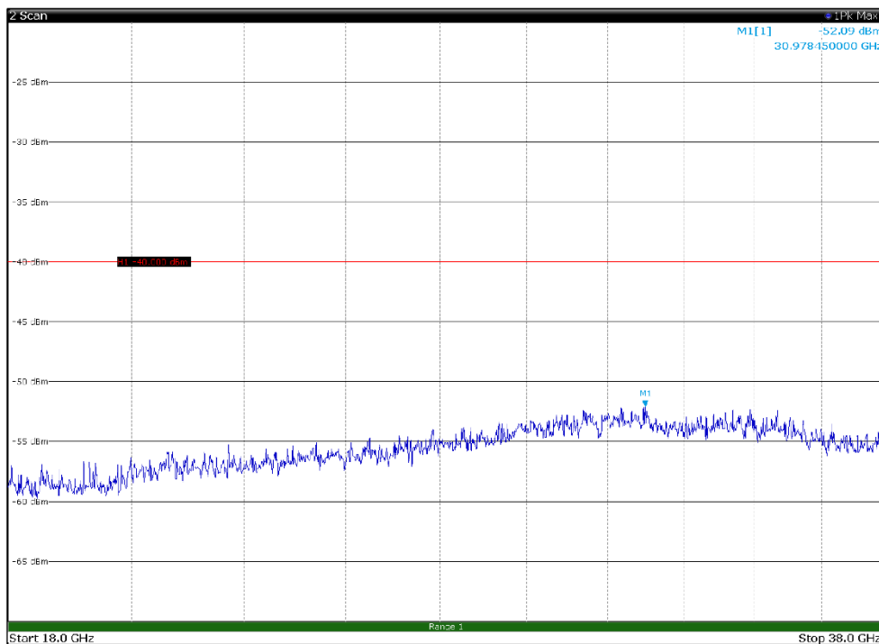
Channel: TOP, Modulation: QPSK, BW=20MHz, Range: 18GHz - 38GHz, Polarization: Vertical
