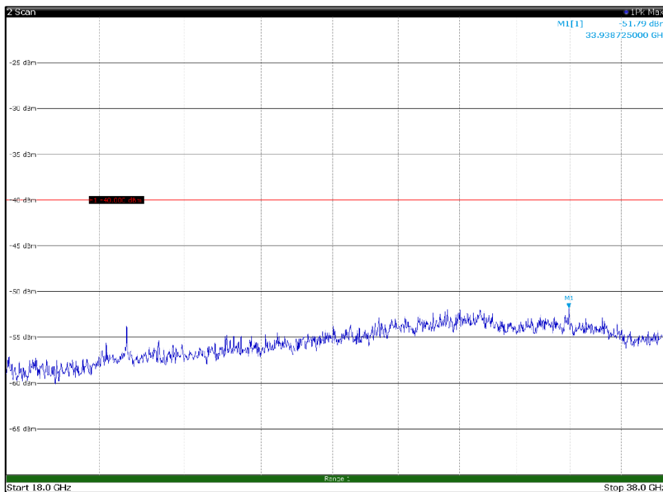
Channel: BOTTOM, Modulation: QPSK, BW=15MHz, Range: 18GHz - 38GHz, Polarization: Vertical
