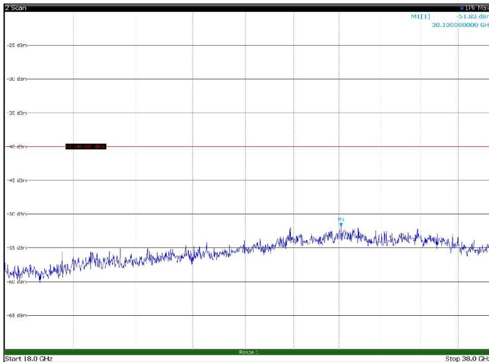
Channel: MIDDLE, Modulation: QPSK, BW=15MHz, Range: 18GHz - 38GHz, Polarization: Vertical
