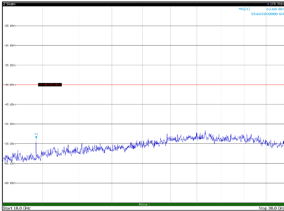
Channel: BOTTOM, Modulation: 64QAM, BW=10MHz, Range: 18GHz - 38GHz, Polarization: Horizontal
