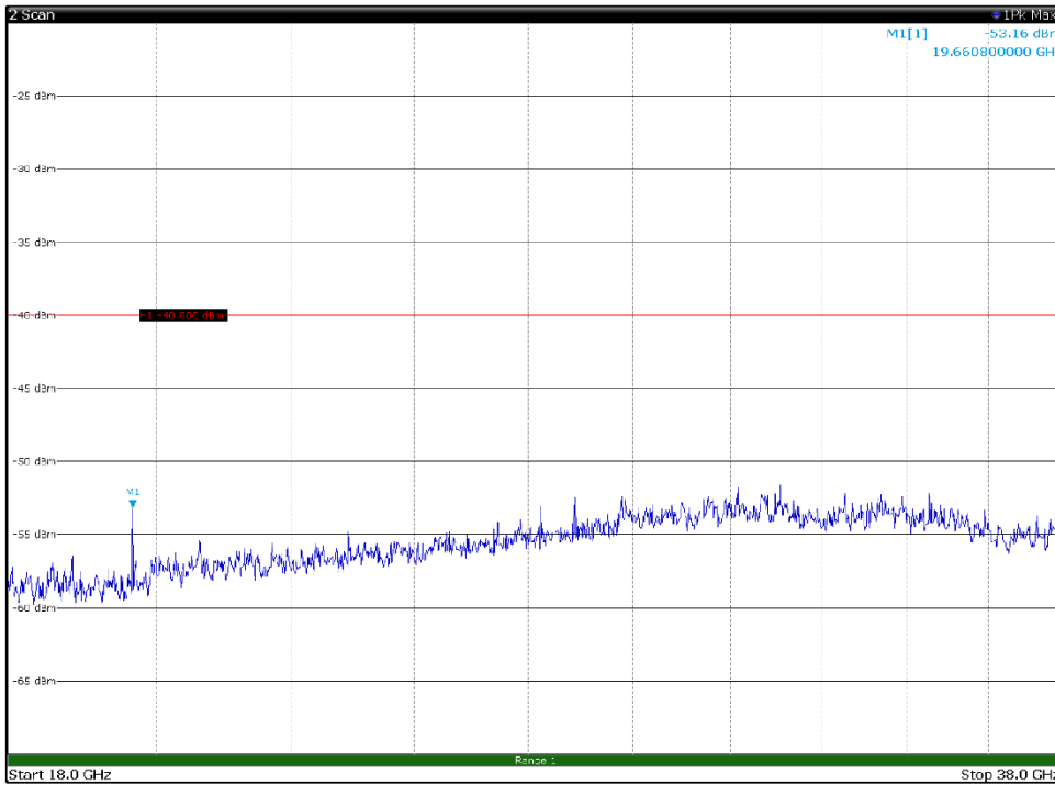
Channel: MIDDLE, Modulation: 16QAM, BW=15MHz, Range: 18GHz - 38GHz, Polarization: Horizontal
