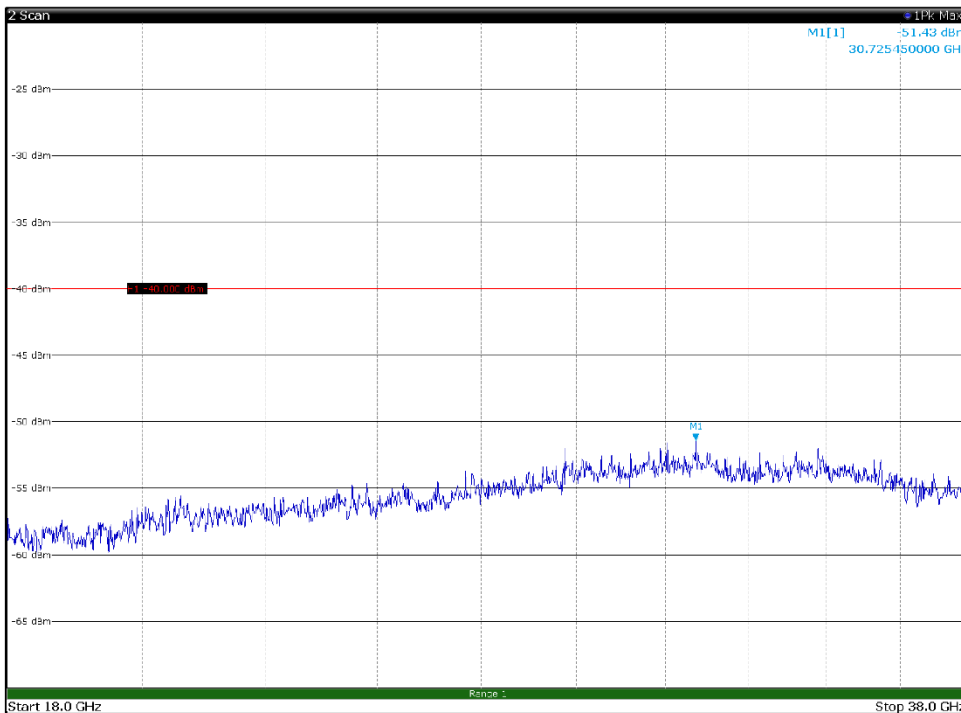
Channel: MIDDLE, Modulation: 16QAM, BW=15MHz, Range: 18GHz - 38GHz, Polarization: Vertical
