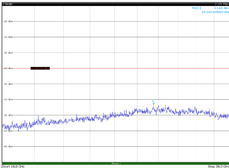
Channel: MIDDLE, Modulation: QPSK, BW=20MHz, Range: 18GHz - 38GHz, Polarization: Vertical
