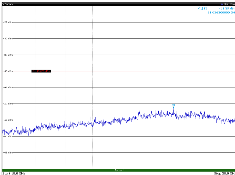
Channel: MIDDLE, Modulation: 64QAM, BW=15MHz, Range: 18GHz - 38GHz, Polarization: Vertical
