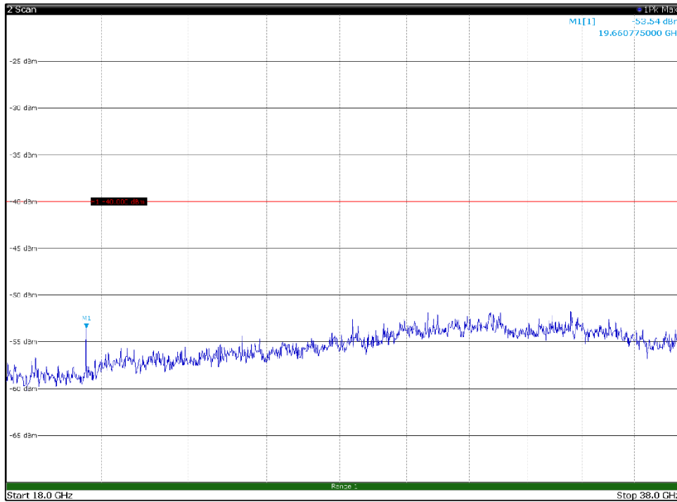
Channel: MIDDLE, Modulation: 256QAM, BW=15MHz, Range: 18GHz - 38GHz, Polarization: Horizontal
