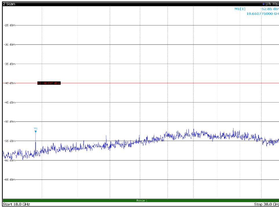
Channel: BOTTOM, Modulation: 256QAM, BW=15MHz, Range: 18GHz - 38GHz, Polarization: Horizontal
