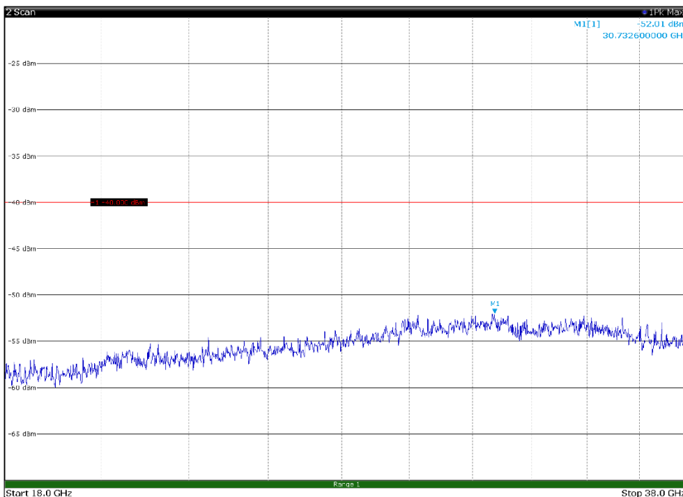
Channel: MIDDLE, Modulation: 256QAM, BW=5MHz, Range: 18GHz - 38GHz, Polarization: Vertical
