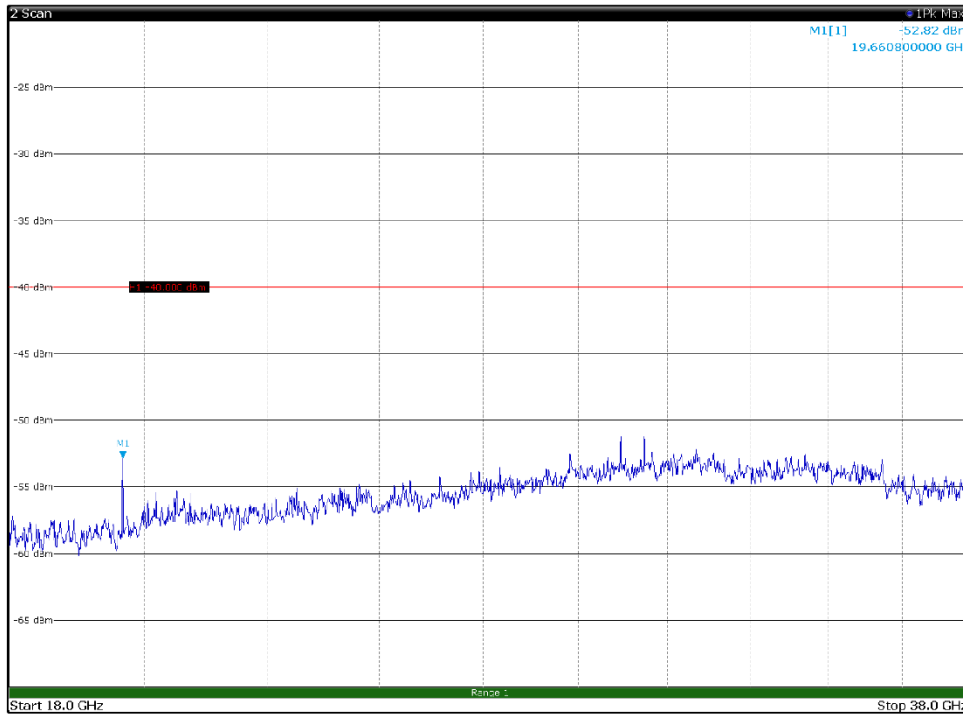
Channel: MIDDLE, Modulation: QPSK, BW=10MHz, Range: 18GHz - 38GHz, Polarization: Horizontal
