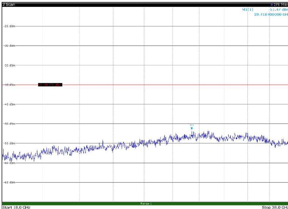
Channel: TOP, Modulation: 16QAM, BW=5MHz, Range: 18GHz - 38GHz, Polarization: Vertical
