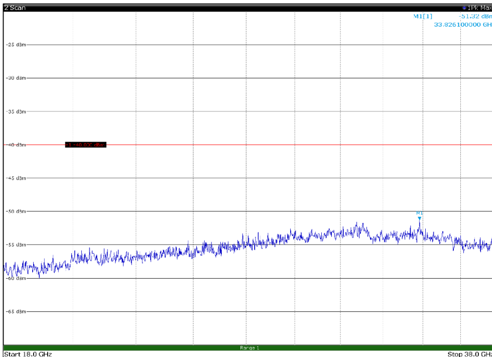
Channel: BOTTOM, Modulation: 256QAM, BW=5MHz, Range: 18GHz - 38GHz, Polarization: Vertical
