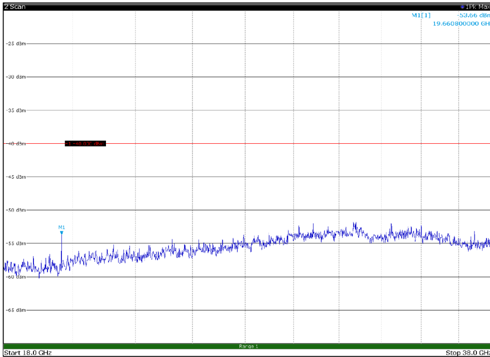
Channel: MIDDLE, Modulation: 256QAM, BW=5MHz, Range: 18GHz - 38GHz, Polarization: Horizontal
