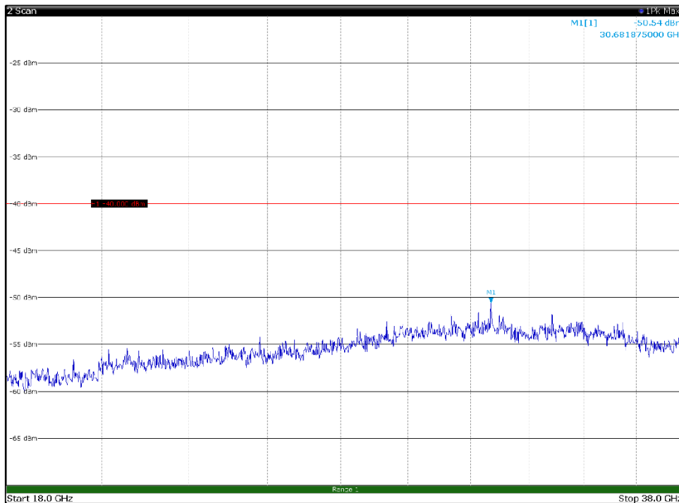
Channel: MIDDLE, Modulation: 16QAM, BW=10MHz, Range: 18GHz - 38GHz, Polarization: Vertical
