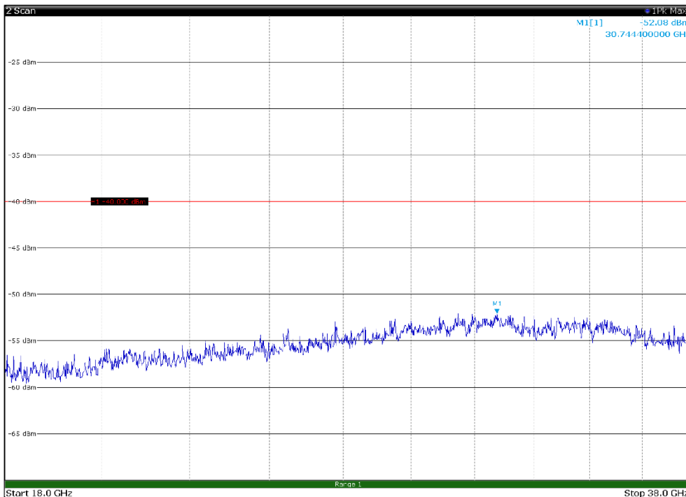
Channel: TOP, Modulation: QPSK, BW=5MHz, Range: 18GHz - 38GHz, Polarization: Vertical
