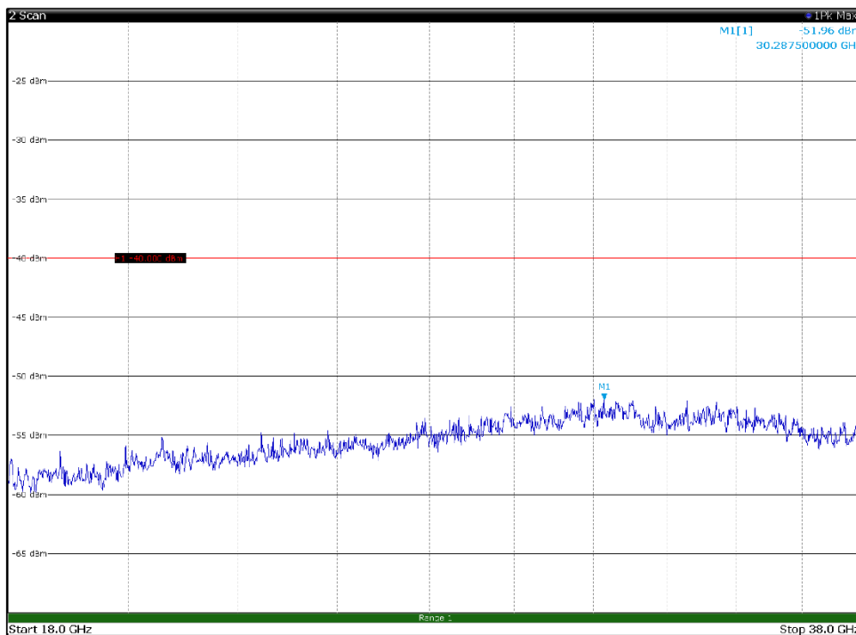
Channel: BOTTOM, Modulation: QPSK, BW=10MHz, Range: 18GHz - 38GHz, Polarization: Vertical
