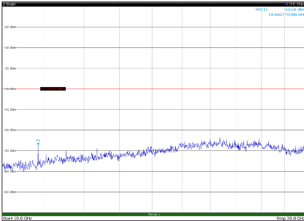
Channel: TOP, Modulation: QPSK, BW=5MHz, Range: 18GHz - 38GHz, Polarization: Horizontal
