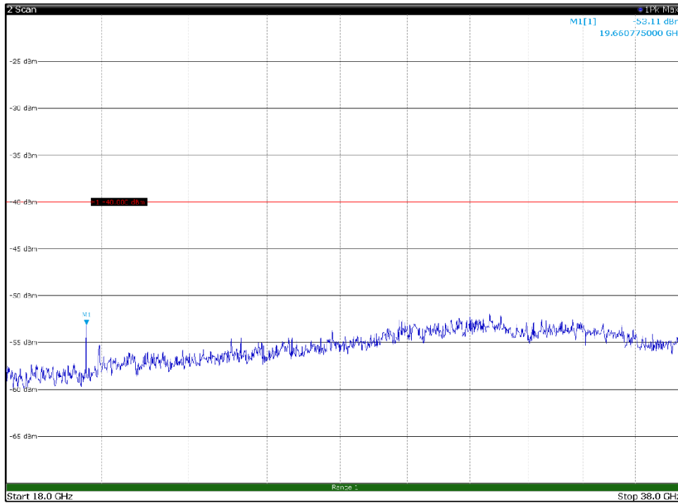
Channel: TOP, Modulation: 16QAM, BW=10MHz, Range: 18GHz - 38GHz, Polarization: Horizontal
