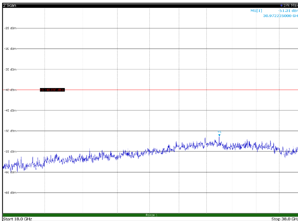
Channel: MIDDLE, Modulation: QPSK, BW=10MHz, Range: 18GHz - 38GHz, Polarization: Vertical
