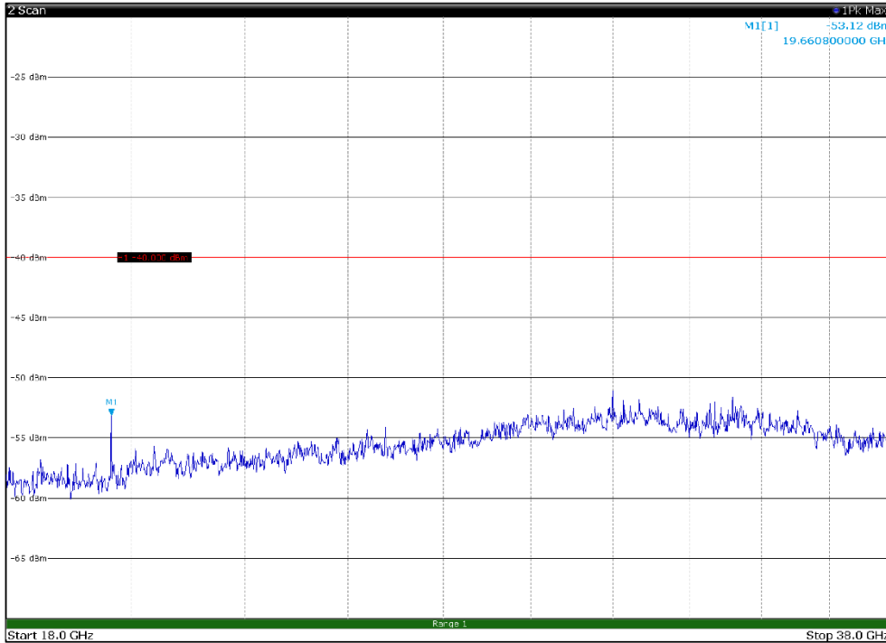
Channel: BOTTOM, Modulation: 256QAM, BW=5MHz, Range: 18GHz - 38GHz, Polarization: Horizontal
