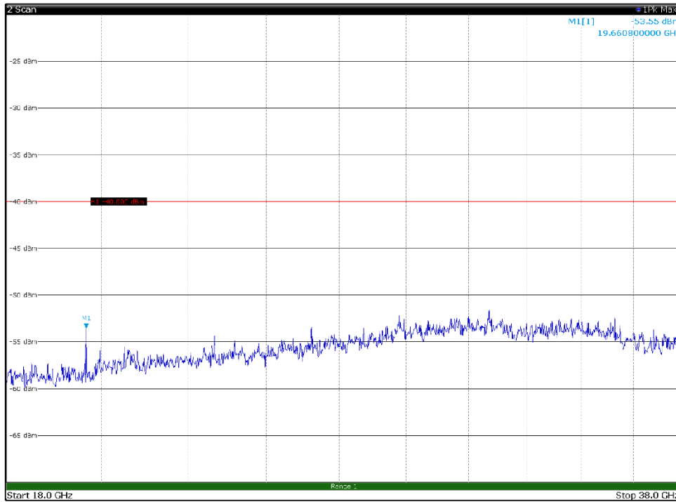
Channel: MIDDLE, Modulation: 16QAM, BW=10MHz, Range: 18GHz - 38GHz, Polarization: Horizontal
