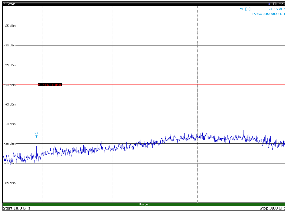
Channel: BOTTOM, Modulation: 16QAM, BW=10MHz, Range: 18GHz - 38GHz, Polarization: Horizontal
