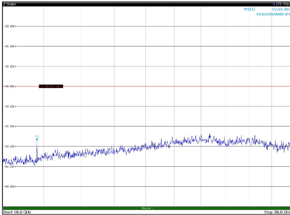
Channel: BOTTOM, Modulation: QPSK, BW=10MHz, Range: 18GHz - 38GHz, Polarization: Horizontal
