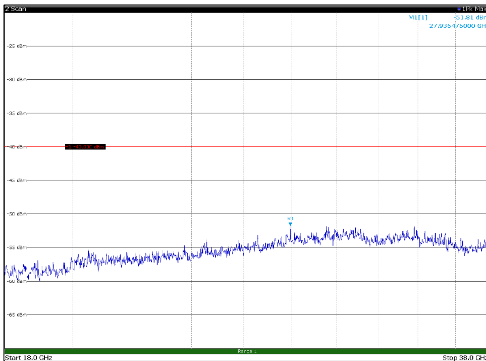
Channel: TOP, Modulation: QPSK, BW=10MHz, Range: 18GHz - 38GHz, Polarization: Vertical
