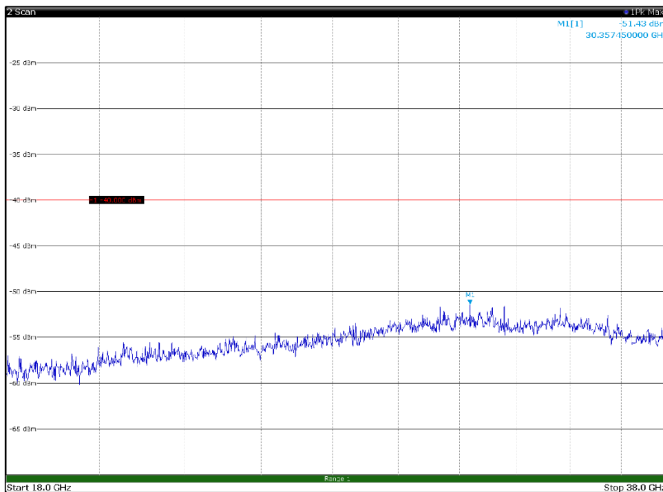
Channel: TOP, Modulation: 16QAM, BW=10MHz, Range: 18GHz - 38GHz, Polarization: Vertical
