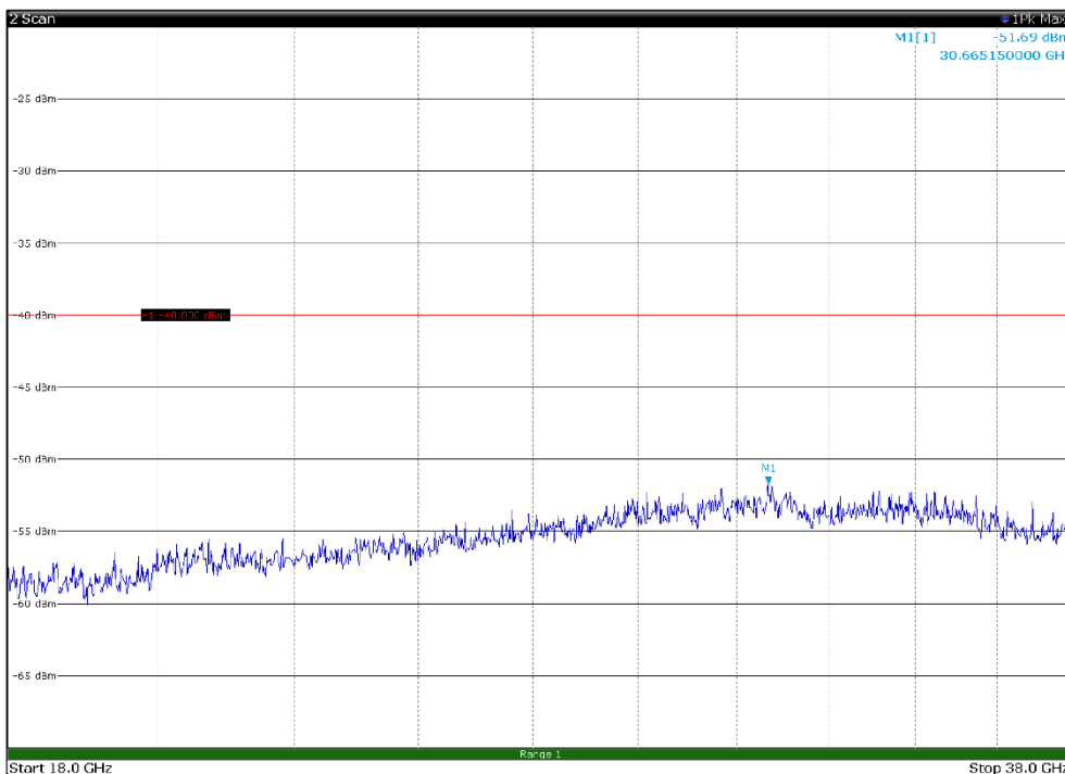
Channel: BOTTOM, Modulation: QPSK, BW=5MHz, Range: 18GHz - 38GHz, Polarization: Vertical
