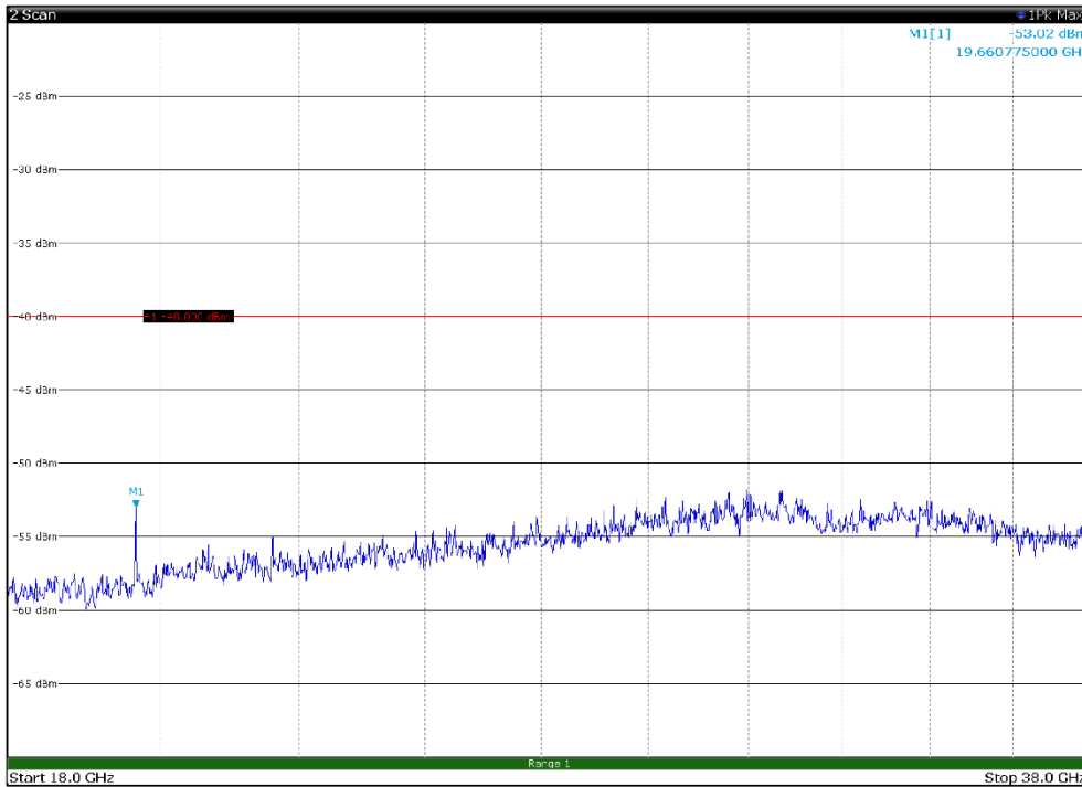
Channel: BOTTOM, Modulation: QPSK, BW=5MHz, Range: 18GHz - 38GHz, Polarization: Horizontal
