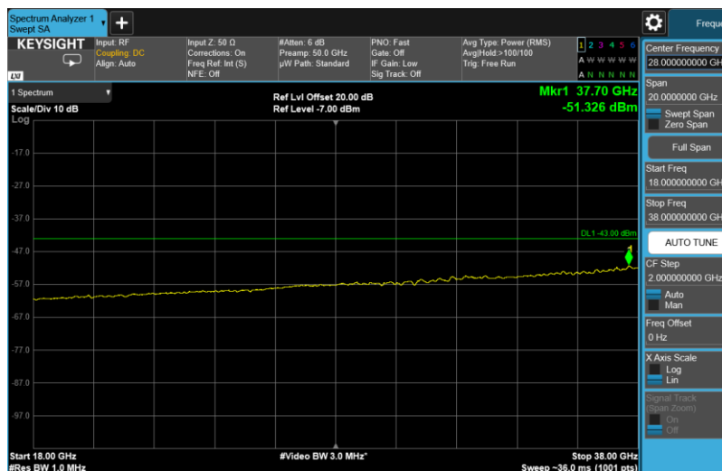
Channel: TOP, Modulation: 256QAM, BW=20MHz, Range: 18GHz - 38GHz
