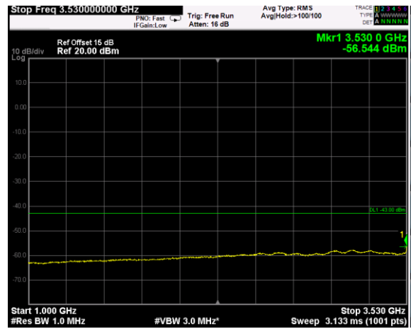
Channel: TOP, Modulation: 16QAM, BW=20MHz, Range: 1GHz - 3530MHz
