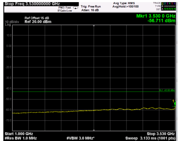
Channel: BOTTOM, Modulation: QPSK, BW=20MHz, Range: 1GHz - 3530MHz
