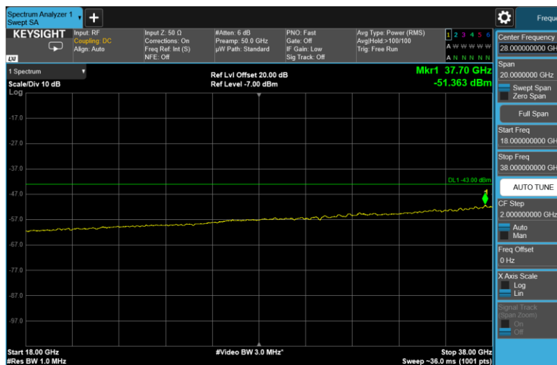
Channel: TOP, Modulation: 64QAM, BW=20MHz, Range: 18GHz - 38GHz
