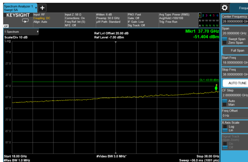
Channel: TOP, Modulation: 16QAM, BW=15MHz, Range: 18GHz - 38GHz
