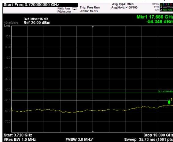
Channel: TOP, Modulation: 16QAM, BW=10MHz, Range: 3720MHz - 18GHz
