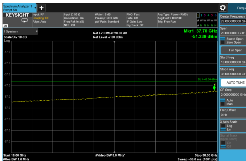
Channel: TOP, Modulation: 64QAM, BW=10MHz, Range: 18GHz - 38GHz
