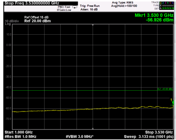
Channel: MIDDLE, Modulation: 16QAM, BW=15MHz, Range: 1GHz - 3530MHz
