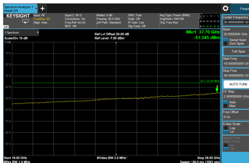
Channel: TOP, Modulation: 16QAM, BW=20MHz, Range: 18GHz - 38GHz
