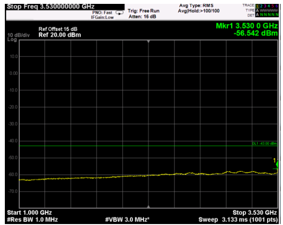
Channel: TOP, Modulation: 64QAM, BW=20MHz, Range: 1GHz - 3530MHz
