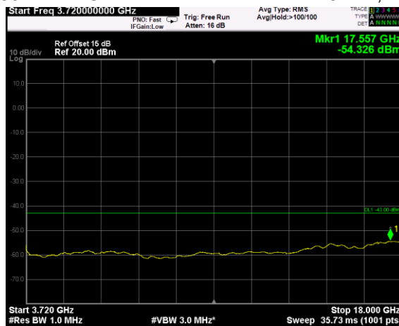
Channel: TOP, Modulation: 16QAM, BW=15MHz, Range: 3720MHz - 18GHz
