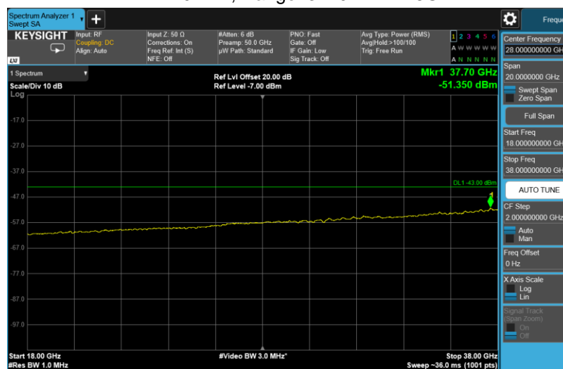
Channel: TOP, Modulation: 16QAM, BW=20MHz, Range: 18GHz - 38GHz
