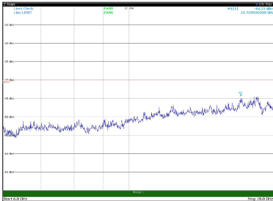
Channel: TOP, Modulation: 256QAM, BW=20MHz, Range: 6GHz -18GHz, Polarization: Vertical
