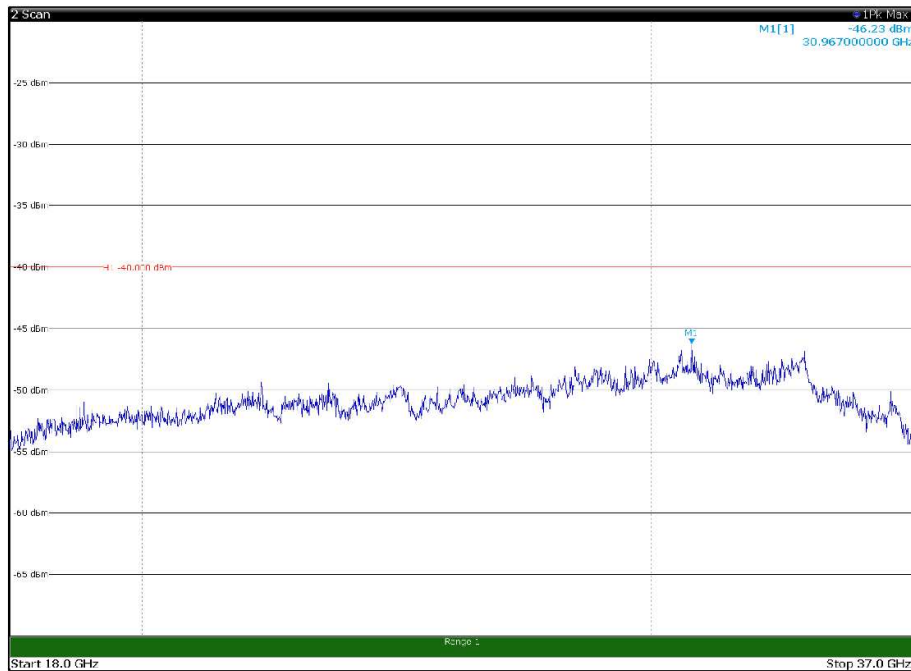
Channel: TOP, Modulation: 256QAM, BW=20MHz, Range: 18GHz - 37GHz, Polarization: Vertical
