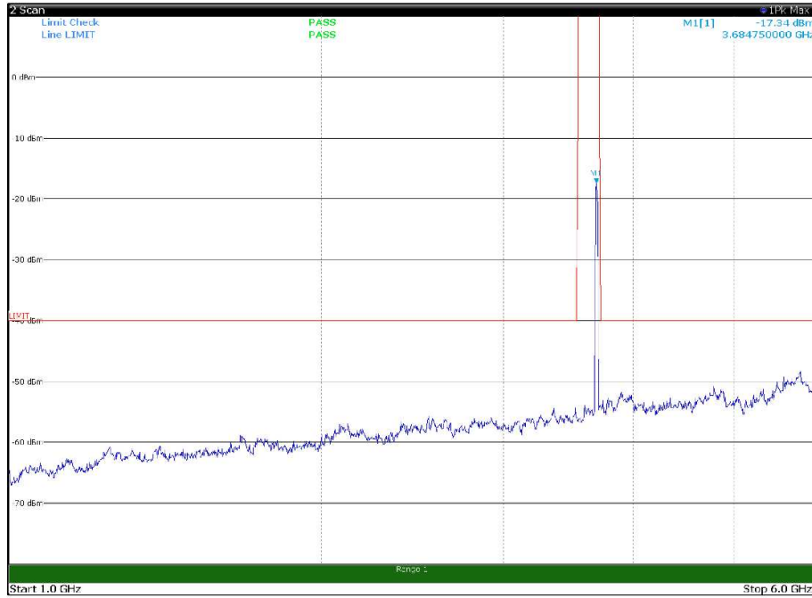
Channel: TOP, Modulation: 256QAM, BW=20MHz, Range: 1GHz -6GHz, Polarization: Horizontal
