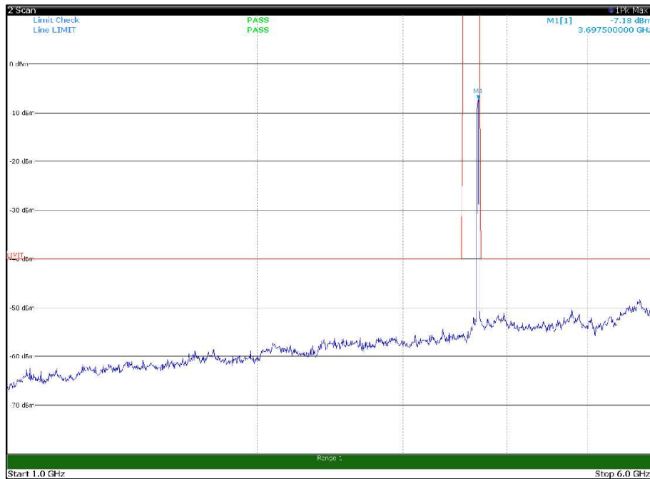
Channel: TOP, Modulation: 256QAM, BW=20MHz, Range: 1GHz -6GHz, Polarization: Vertical
