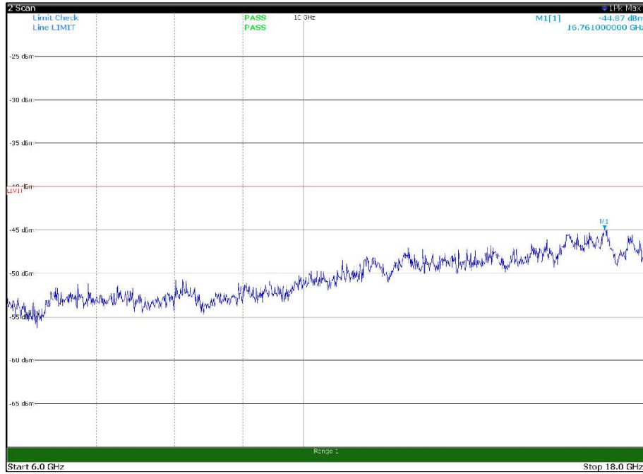
Channel: TOP, Modulation: 256QAM, BW=20MHz, Range: 6GHz -18GHz, Polarization: Horizontal
