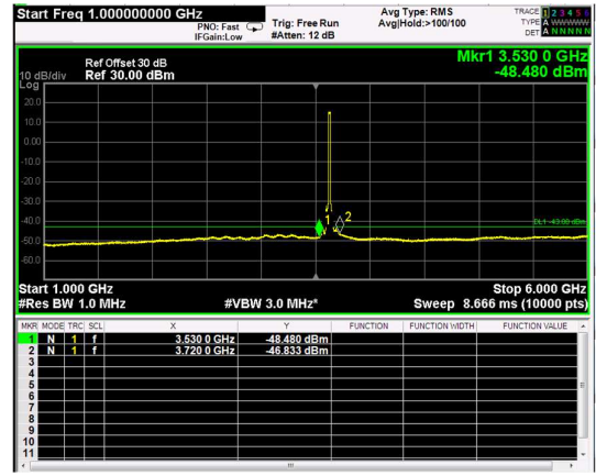
Channel: MIDDLE, Modulation: 64QAM, BW=20MHz, Range: 1GHz - 6GHz
