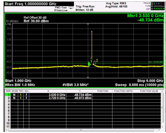
Channel: MIDDLE, Modulation: 16QAM, BW=20MHz, Range: 1GHz - 6GHz
