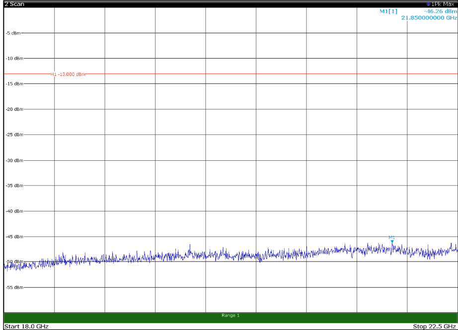
Channel: BOTTOM, Modulation: 256QAM, BW=10MHz, Range: 18GHz - 22.5GHz, Polarization: Vertical
