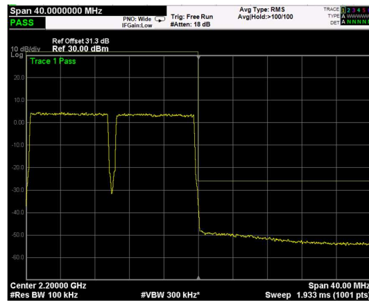
High Band Edge, 2 Carrier, Modulation: 16QAM, BW=10MHz
