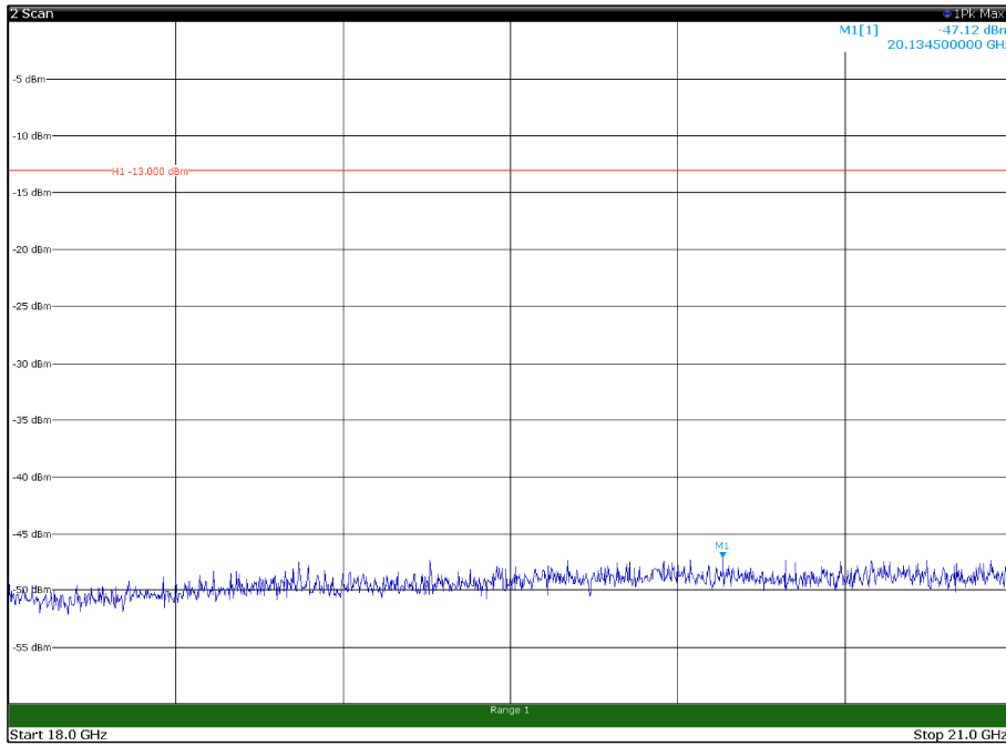
Channel: MIDDLE, Modulation: 256QAM, BW=20MHz, Range: 18GHz - 21GHz, Polarization: Horizontal
