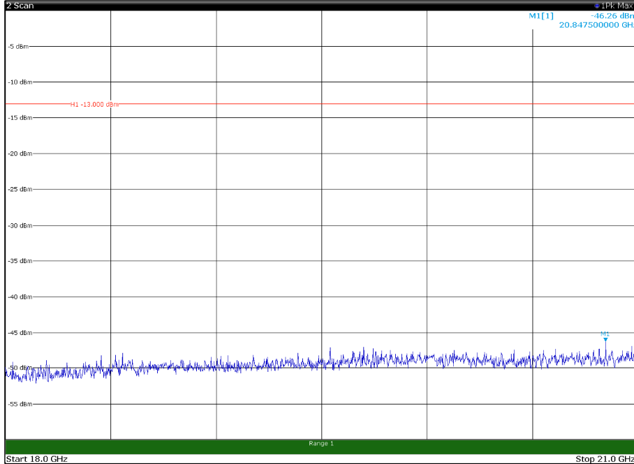
Channel: TOP, Modulation: 256QAM, BW=20MHz, Range: 18GHz - 21GHz, Polarization: Vertical
