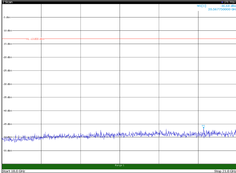
Channel: BOTTOM, Modulation: 256QAM, BW=20MHz, Range: 18GHz - 21GHz, Polarization: Vertical
