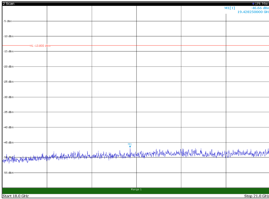
Channel: BOTTOM, Modulation: 256QAM, BW=20MHz, Range: 18GHz - 21GHz, Polarization: Horizontal
