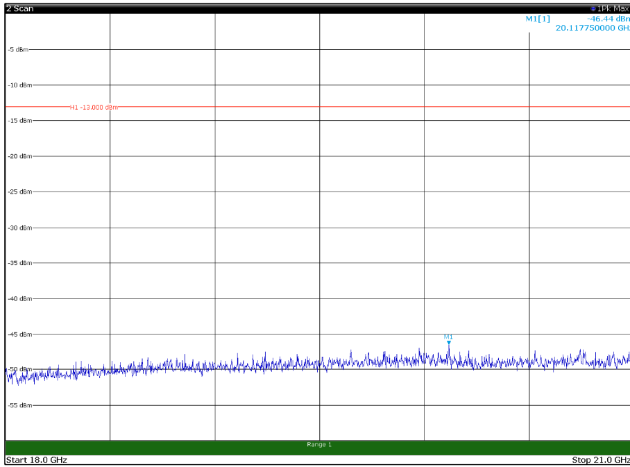
Channel: TOP, Modulation: 64QAM, BW=20MHz, Range: 18GHz - 21GHz, Polarization: Horizontal
