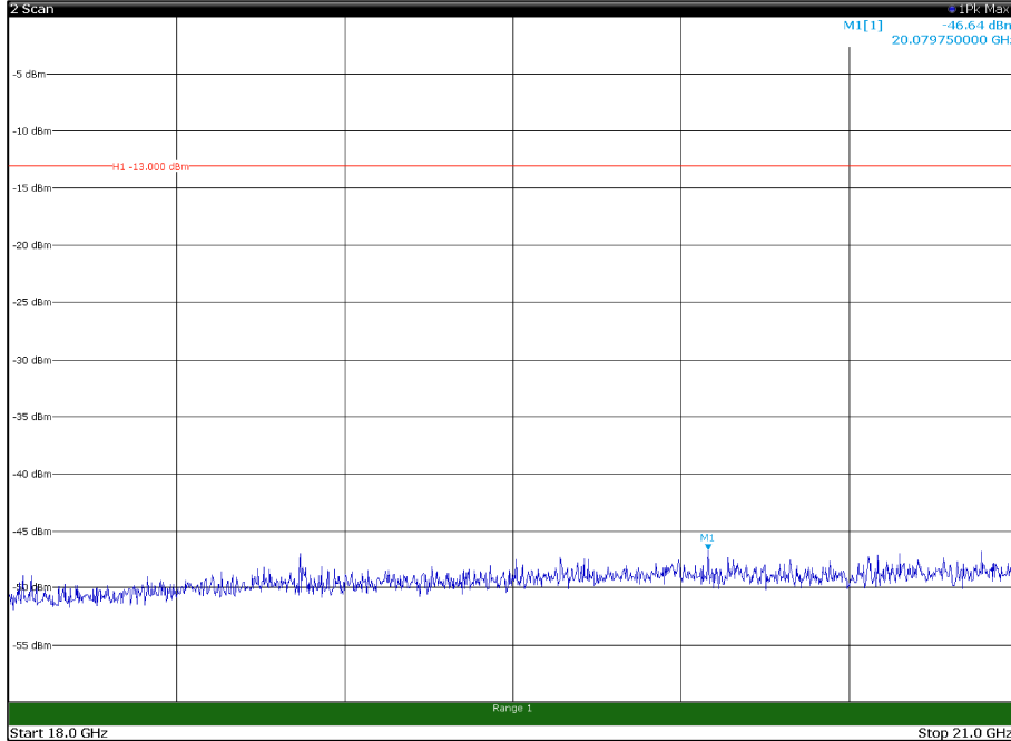
Channel: MIDDLE, Modulation: 256QAM, BW=20MHz, Range: 18GHz - 21GHz, Polarization: Vertical
