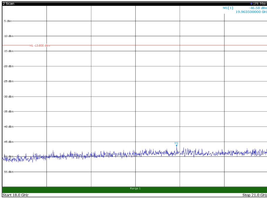
Channel: MIDDLE, Modulation: 64QAM, BW=20MHz, Range: 18GHz - 21GHz, Polarization: Horizontal
