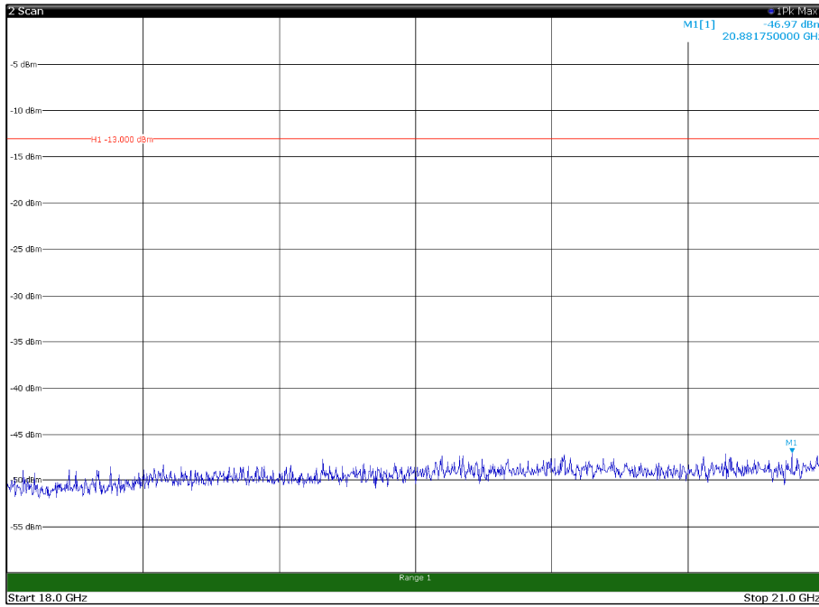
Channel: TOP, Modulation: 256QAM, BW=20MHz, Range: 18GHz - 21GHz, Polarization: Horizontal
