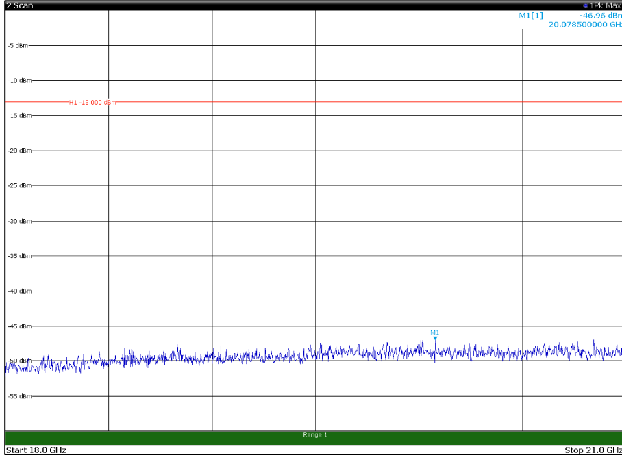
Channel: MIDDLE, Modulation: 64QAM, BW=20MHz, Range: 18GHz - 21GHz, Polarization: Vertical
