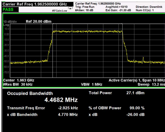
Channel: MIDDLE, Modulation: 64QAM, BW=5MHz
