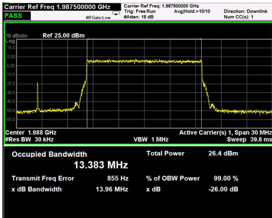
Channel: TOP, Modulation: 64QAM, BW=15MHz
