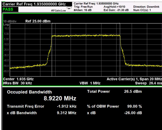
Channel: BOTTOM, Modulation: 64QAM, BW=10MHz
