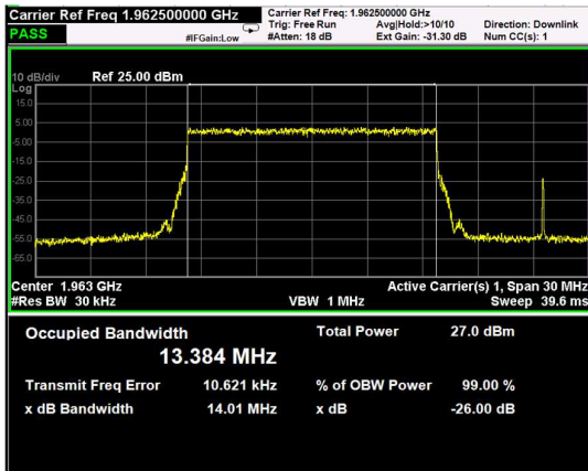
Channel: MIDDLE, Modulation: 64QAM, BW=15MHz
