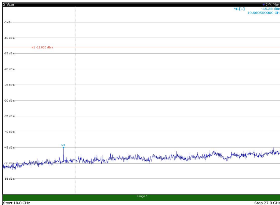
Channel: MIDDLE, Modulation: 256QAM, BW=20MHz, Range: 18GHz - 27GHz, Polarization: Vertical
