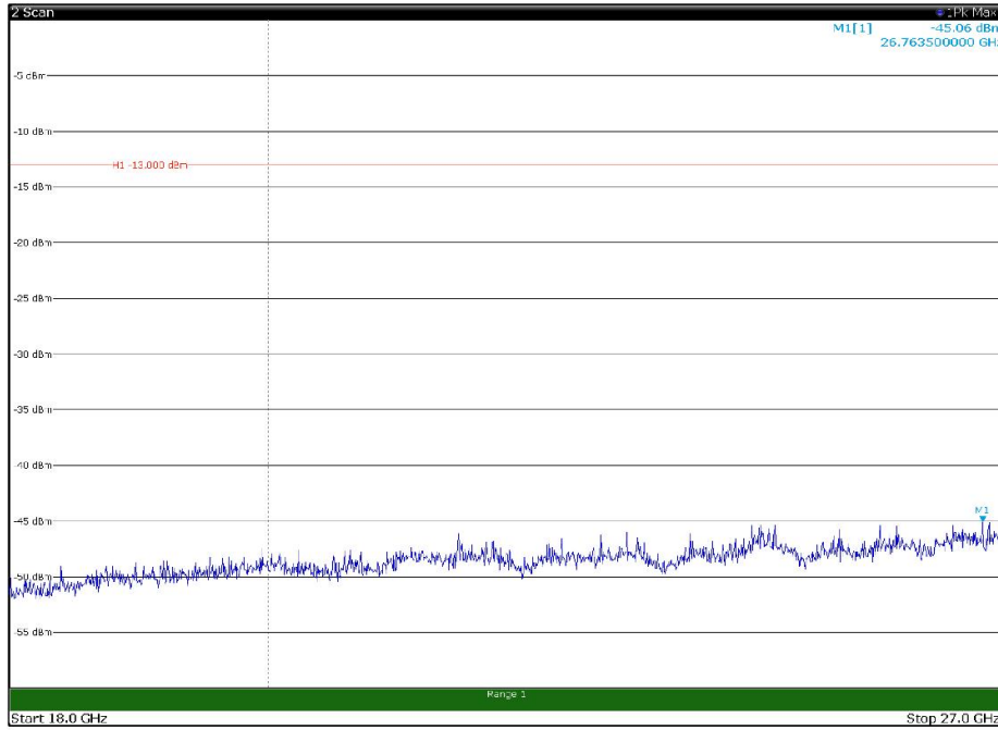
Channel: MIDDLE, Modulation: 256QAM, BW=20MHz, Range: 18GHz - 27GHz, Polarization: Horizontal
