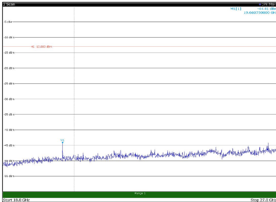
Channel: TOP, Modulation: 256QAM, BW=20MHz, Range: 18GHz - 27GHz, Polarization: Vertical
