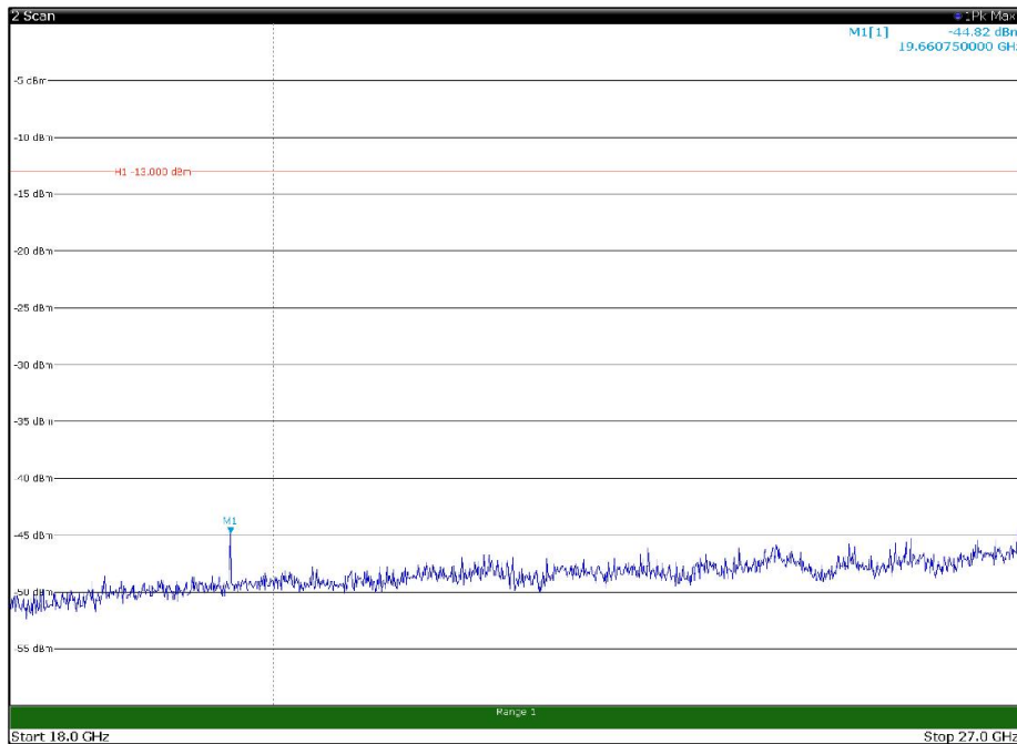
Channel: BOTTOM, Modulation: 256QAM, BW=20MHz, Range: 18GHz - 27GHz, Polarization: Vertical
