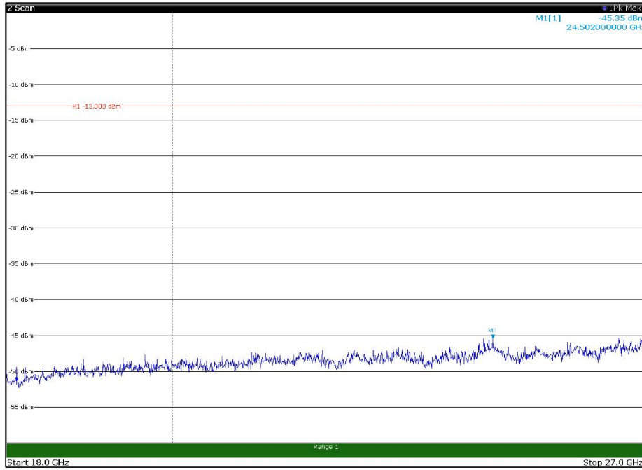
Channel: MIDDLE, Modulation: QPSK, BW=20MHz, Range: 18GHz - 27GHz, Polarization: Horizontal
