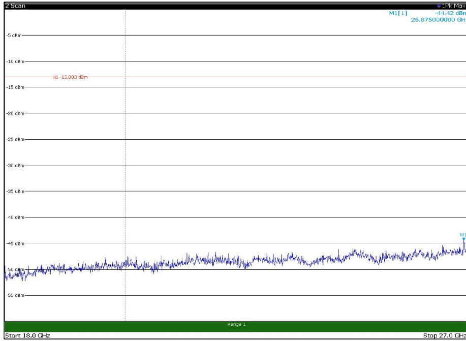
Channel: BOTTOM, Modulation: 16QAM, BW=20MHz, Range: 18GHz - 27GHz, Polarization: Horizontal
