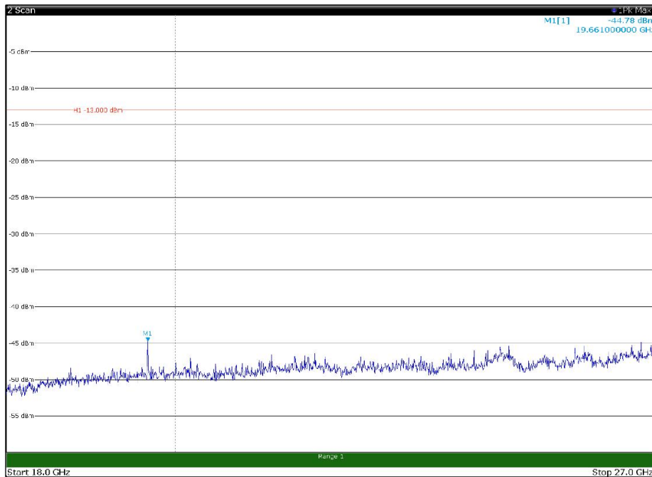
Channel: BOTTOM, Modulation: 16QAM, BW=20MHz, Range: 18GHz - 27GHz, Polarization: Vertical
