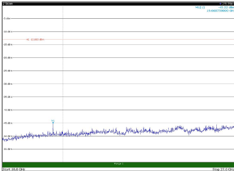
Channel: MIDDLE, Modulation: 16QAM, BW=20MHz, Range: 18GHz - 27GHz, Polarization: Vertical
