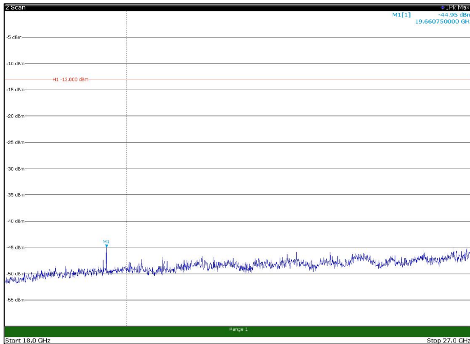
Channel: TOP, Modulation: QPSK, BW=20MHz, Range: 18GHz - 27GHz, Polarization: Vertical
