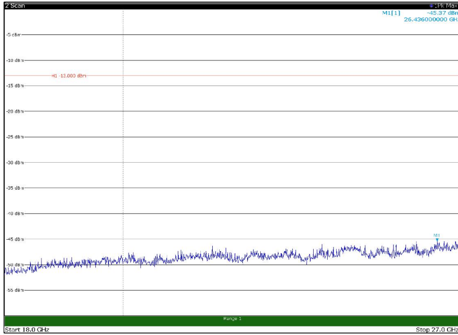
Channel: TOP, Modulation: QPSK, BW=20MHz, Range: 18GHz - 27GHz, Polarization: Horizontal
