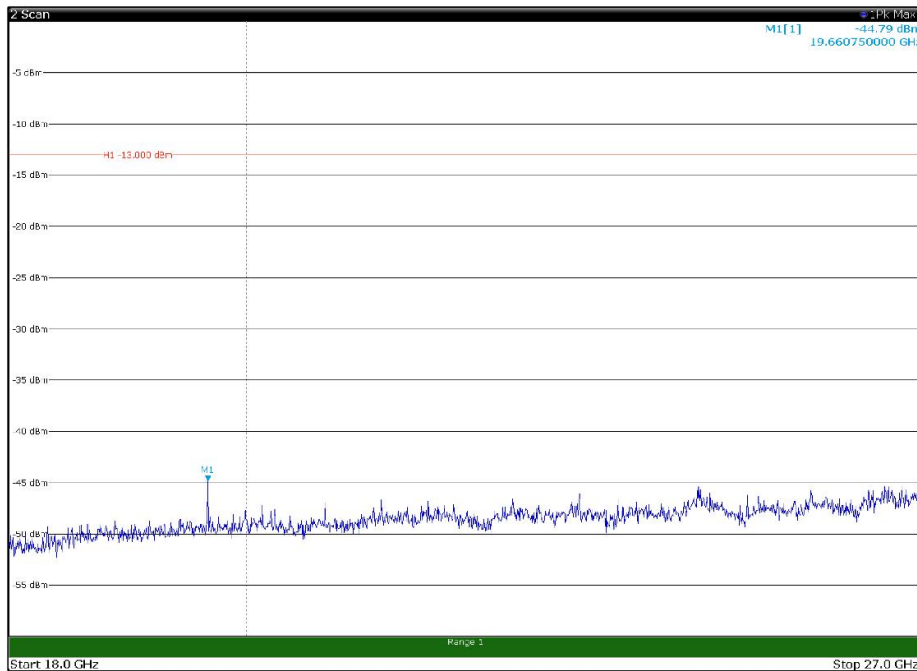
Channel: TOP, Modulation: 16QAM, BW=20MHz, Range: 18GHz - 27GHz, Polarization: Vertical
