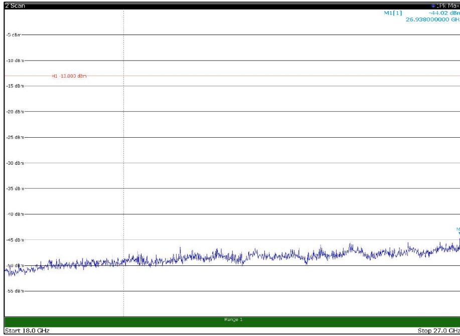
Channel: TOP, Modulation: 256QAM, BW=15MHz, Range: 18GHz - 27GHz, Polarization: Horizontal
