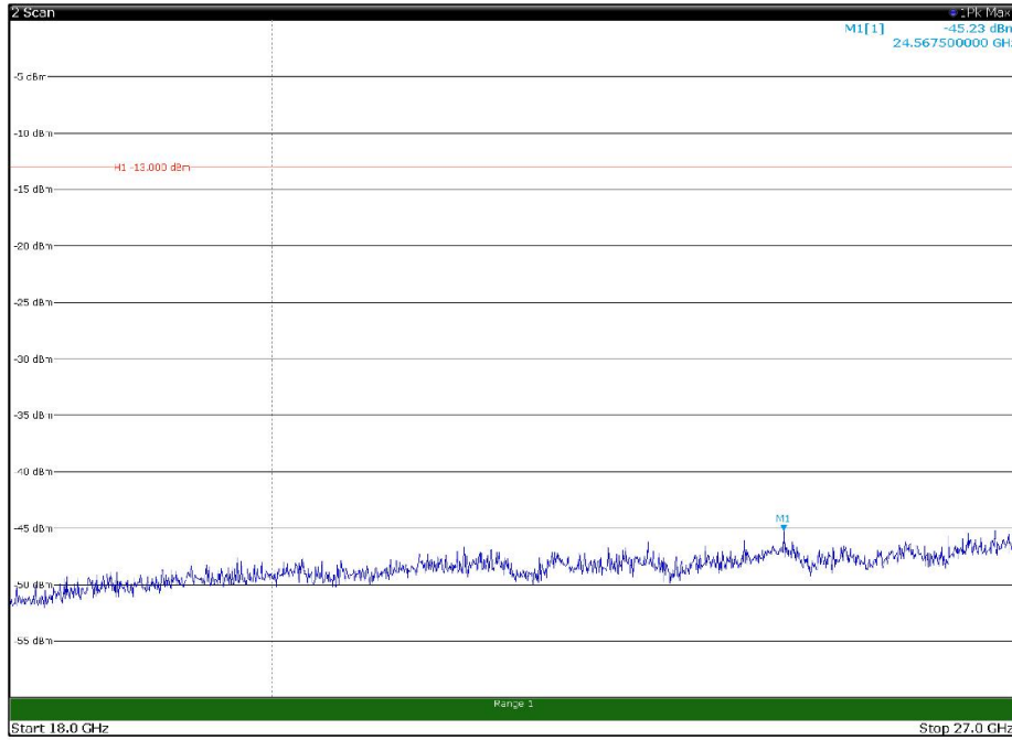
Channel: BOTTOM, Modulation: QPSK, BW=20MHz, Range: 18GHz - 27GHz, Polarization: Horizontal
