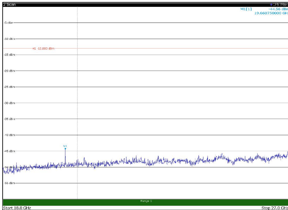
Channel: TOP, Modulation: 256QAM, BW=15MHz, Range: 18GHz - 27GHz, Polarization: Vertical
