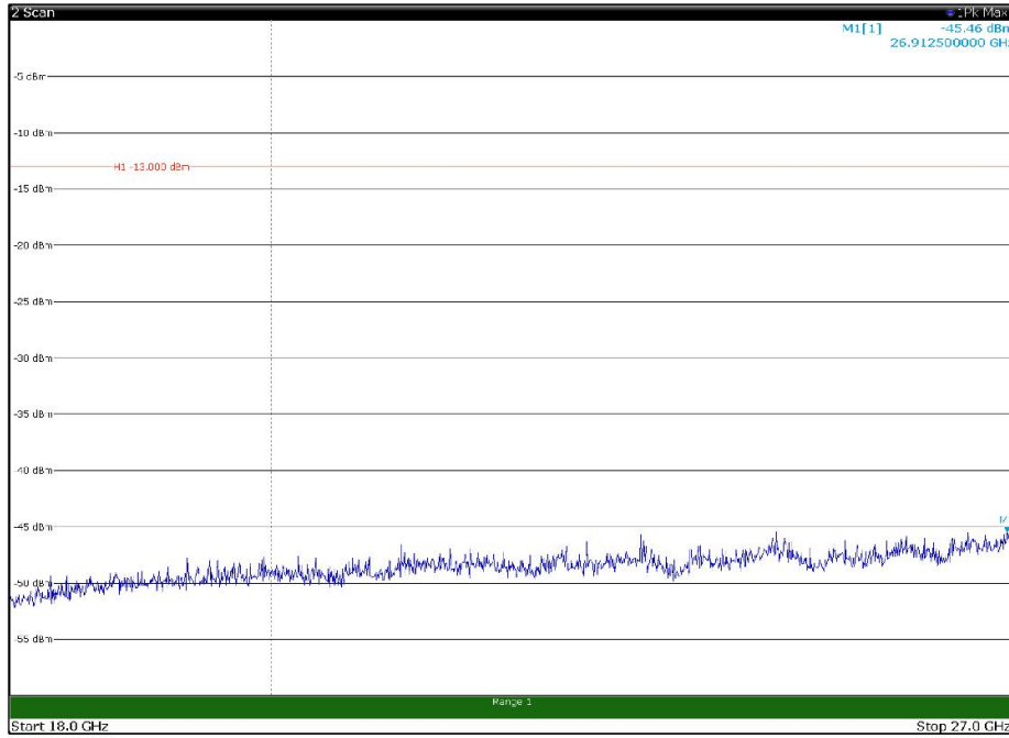
Channel: MIDDLE, Modulation: 256QAM, BW=15MHz, Range: 18GHz - 27GHz, Polarization: Horizontal
