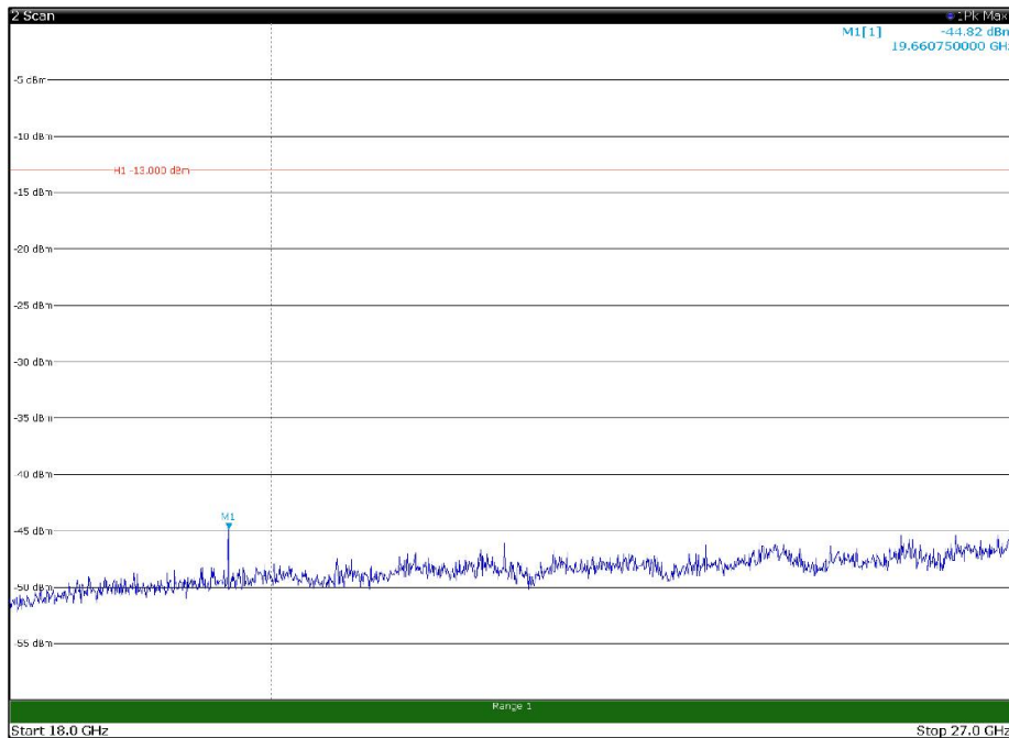
Channel: MIDDLE, Modulation: QPSK, BW=20MHz, Range: 18GHz - 27GHz, Polarization: Vertical
