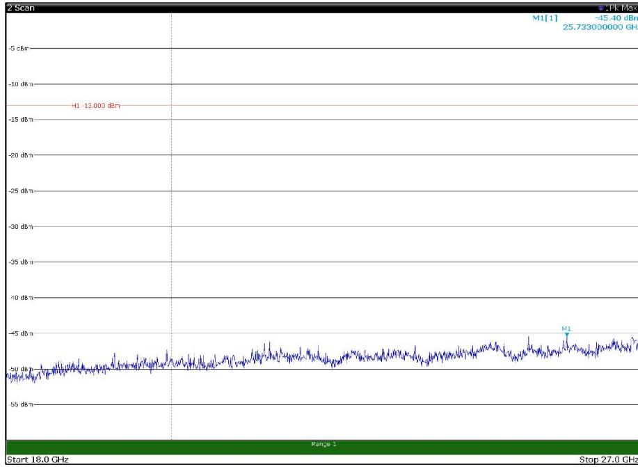
Channel: TOP, Modulation: 16QAM, BW=20MHz, Range: 18GHz - 27GHz, Polarization: Horizontal
