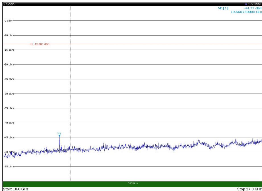
Channel: MIDDLE, Modulation: 256QAM, BW=10MHz, Range: 18GHz - 27GHz, Polarization: Vertical
