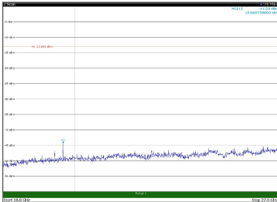
Channel: TOP, Modulation: QPSK, BW=10MHz, Range: 18GHz - 27GHz, Polarization: Vertical
