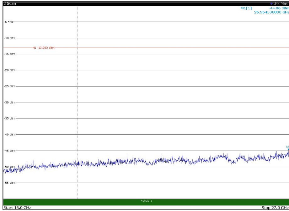
Channel: MIDDLE, Modulation: QPSK, BW=10MHz, Range: 18GHz - 27GHz, Polarization: Horizontal
