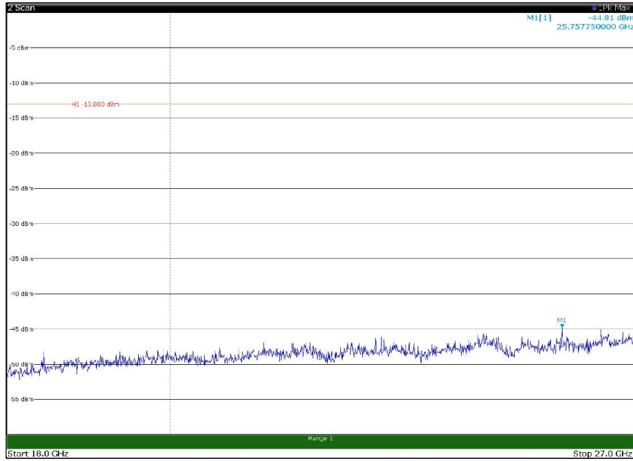
Channel: MIDDLE, Modulation: 64QAM, BW=10MHz, Range: 18GHz - 27GHz, Polarization: Horizontal
