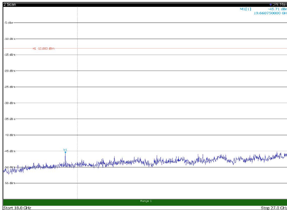
Channel: MIDDLE, Modulation: 16QAM, BW=10MHz, Range: 18GHz - 27GHz, Polarization: Vertical
