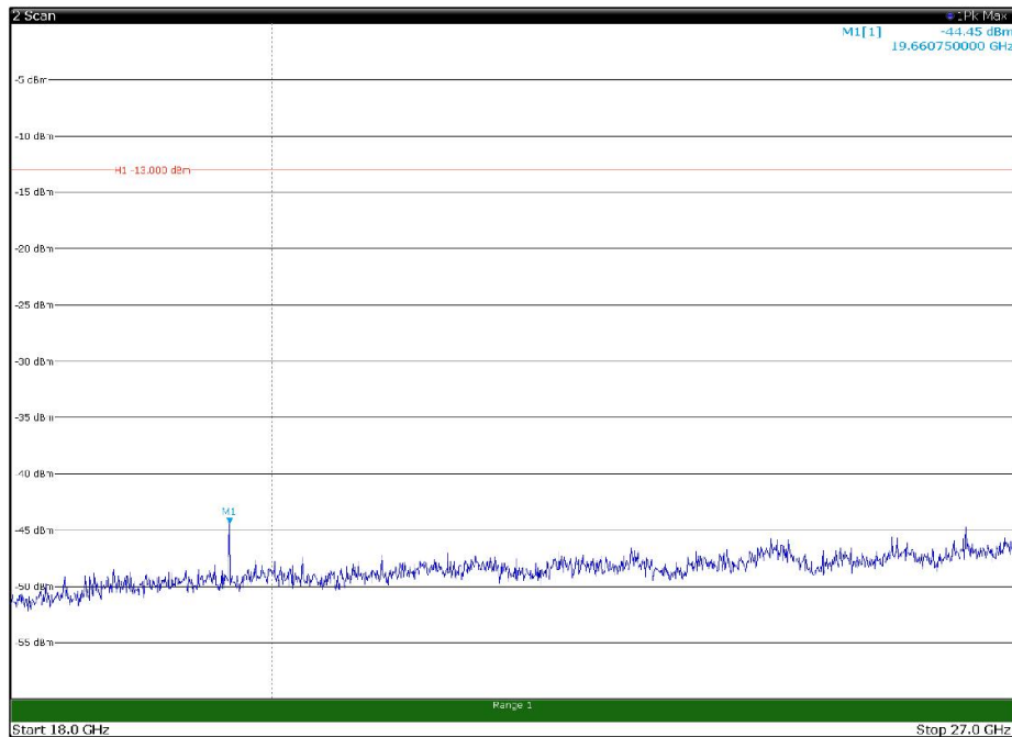
Channel: BOTTOM, Modulation: 256QAM, BW=10MHz, Range: 18GHz - 27GHz, Polarization: Vertical
