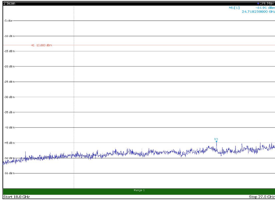
Channel: BOTTOM, Modulation: 256QAM, BW=10MHz, Range: 18GHz - 27GHz, Polarization: Horizontal
