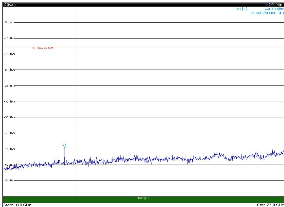
Channel: MIDDLE, Modulation: QPSK, BW=10MHz, Range: 18GHz - 27GHz, Polarization: Vertical
