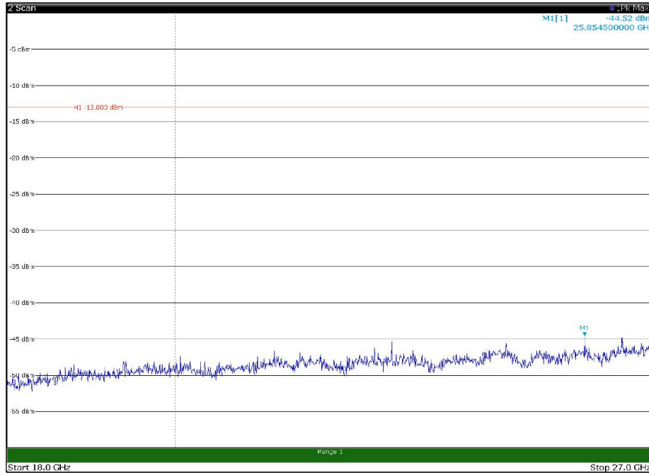
Channel: TOP, Modulation: QPSK, BW=10MHz, Range: 18GHz - 27GHz, Polarization: Horizontal
