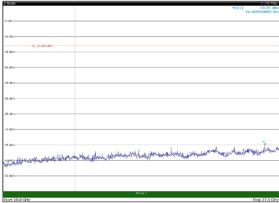
Channel: MIDDLE, Modulation: 256QAM, BW=10MHz, Range: 18GHz - 27GHz, Polarization: Horizontal
