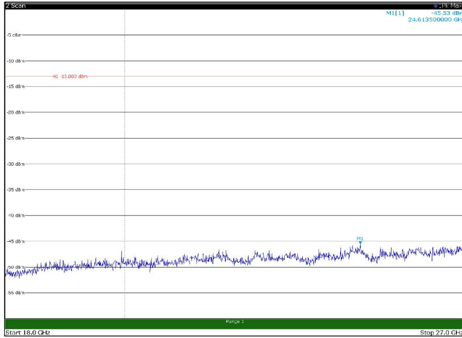
Channel: BOTTOM, Modulation: 16QAM, BW=10MHz, Range: 18GHz - 27GHz, Polarization: Horizontal
