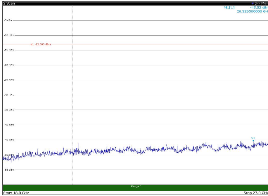
Channel: MIDDLE, Modulation: 16QAM, BW=10MHz, Range: 18GHz - 27GHz, Polarization: Horizontal
