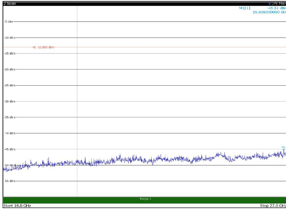
Channel: BOTTOM, Modulation: QPSK, BW=10MHz, Range: 18GHz - 27GHz, Polarization: Horizontal
