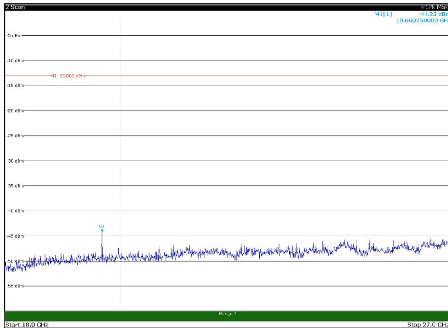
Channel: BOTTOM, Modulation: QPSK, BW=10MHz, Range: 18GHz - 27GHz, Polarization: Vertical
