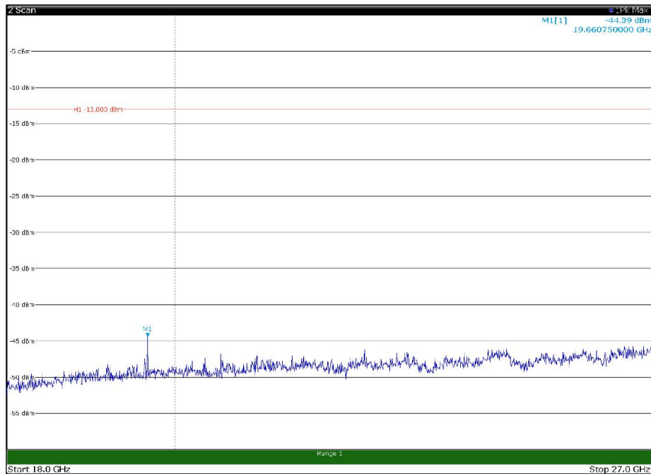
Channel: MIDDLE, Modulation: 64QAM, BW=10MHz, Range: 18GHz - 27GHz, Polarization: Vertical
