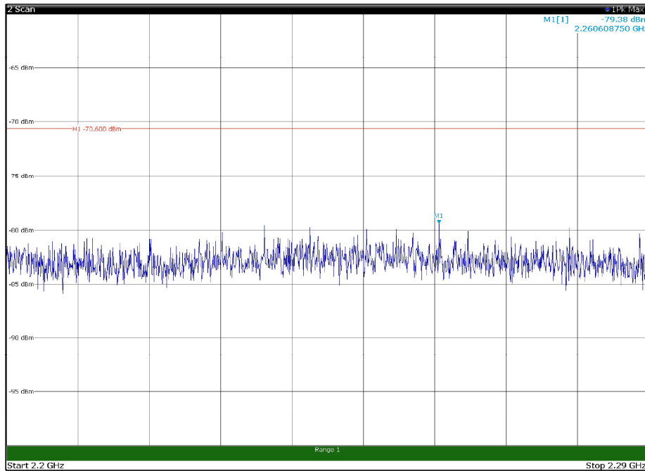
Channel: MIDDLE, Modulation: QPSK, BW=5MHz, Range: 2200MHz-2290GHz, Polarization: Vertical
