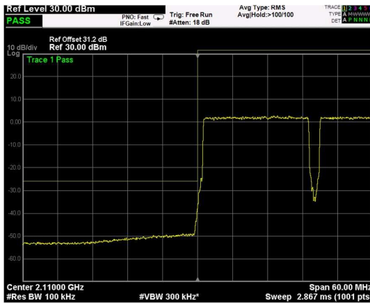
Low Band Edge, 2 Carrier, Modulation: 16QAM, BW=20MHz
