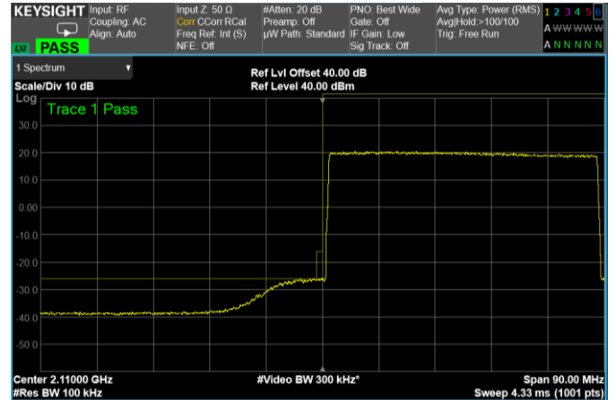
45 MHz signal, Low Band Edge, 1 carrier, nominal input signal + 3dB
