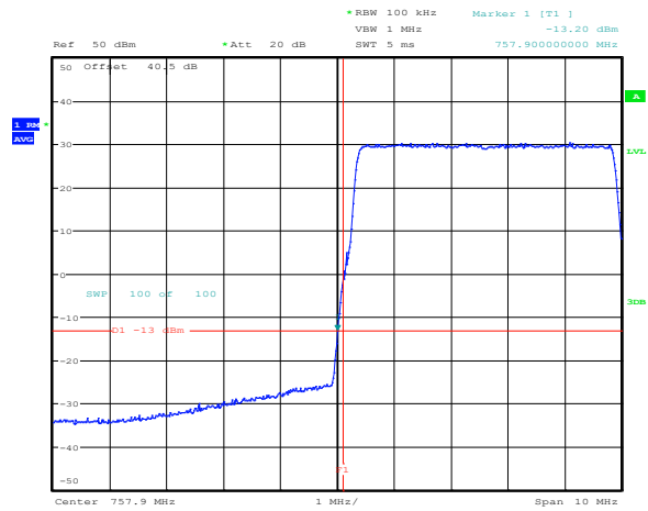
Figure 8.5-16: Conducted lower band edge at 758 MHz at AGC threshold + 3 dB (700FistNet)
