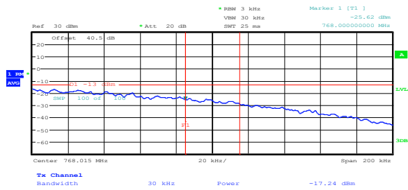
Figure 8.5-19: Conducted upper band edge at 768 MHz at AGC threshold (700FistNet)
