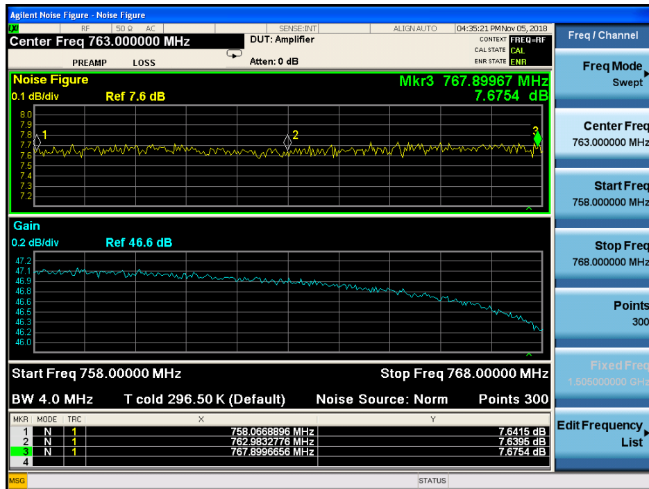
Figure 8.4-1: Noise figure
