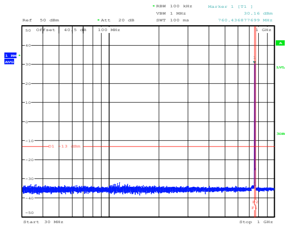
Figure 8.5-1: Conducted spurious emissions below 1 GHz for low channel (700FirtsNet)
