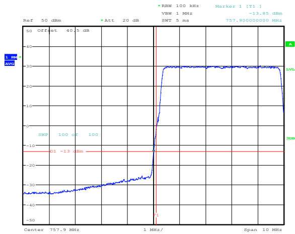
Figure 8.5-15: Conducted lower band edge at 758 MHz at AGC threshold (700FistNet)
