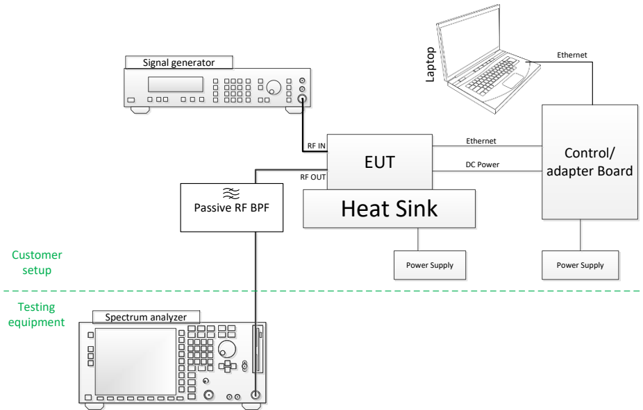
Figure 3.6-1: Setup diagram
