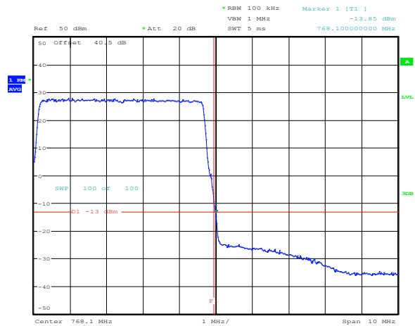
Figure 8.5-20: Conducted upper band edge at 768 MHz at AGC threshold + 3 dB (700FistNet)
