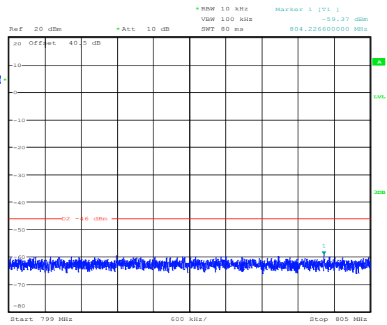
Figure 8.5-8: Conducted spurious emissions 799-805 MHz for mid channel (700FirstNet)
