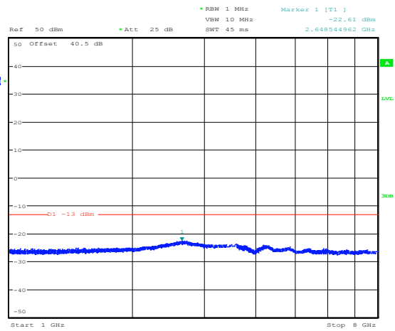
Figure 8.5-5: Conducted spurious emissions above 1 GHz for mid channel (700FirstNet)
