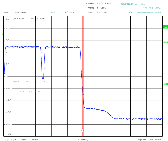
Figure 8.5-28: Conducted upper band edge at 768 MHz at AGC threshold + 3 dB (intermodulation) (700FistNet)
