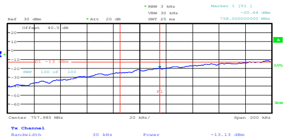
Figure 8.5-16: Conducted lower band edge at 758 MHz at AGC threshold + 3 dB (700FistNet)
