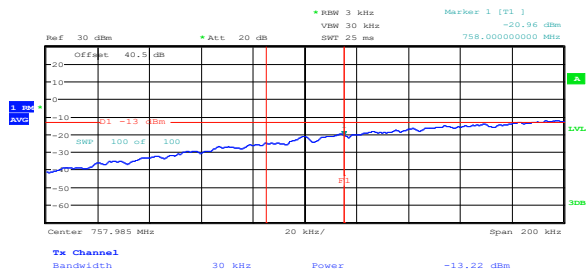
Figure 8.5-15: Conducted lower band edge at 758 MHz at AGC threshold (700FistNet)
