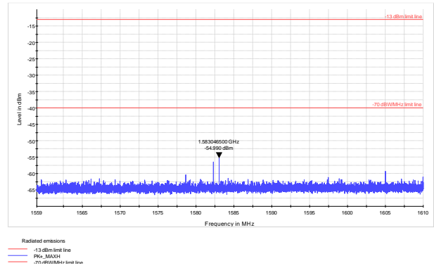
Figure 8.6-8: Radiated spurious emissions within 1559–1610 MHz – Mid Channel (700FirstNet)
