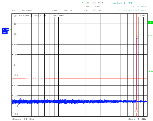
Figure 8.5-3: Conducted spurious emissions below 1 GHz for high channel (700FirtsNet)
