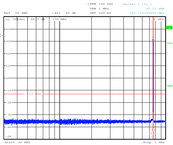
Figure 8.5-2: Conducted spurious emissions below 1 GHz for mid channel (700FirtsNet)
