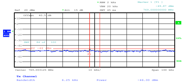
Figure 8.5-12: Conducted spurious emissions 769-775MHz for Mid channel (700FirstNet)
