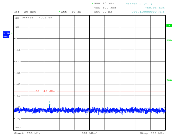
Figure 8.5-9: Conducted spurious emissions 799-805 MHz for high channel (700FirstNet)
