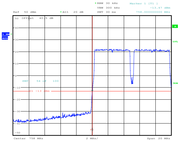
Figure 8.5-23: Conducted lower band edge at 758 MHz at AGC threshold (intermodulation) (700FistNet)
