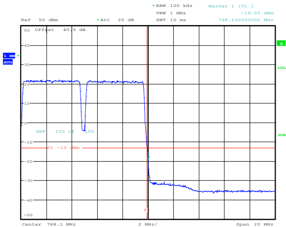
Figure 8.5-27: Conducted upper band edge at 768 MHz at AGC threshold (intermodulation) (700FistNet)
