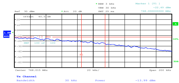
Figure 8.5-20: Conducted upper band edge at 768 MHz at AGC threshold + 3 dB (700FistNet)
