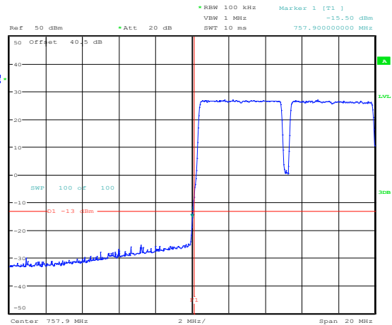
Figure 8.5-24: Conducted lower band edge at 758 MHz at AGC threshold + 3 dB (intermodulation) (700FistNet)
