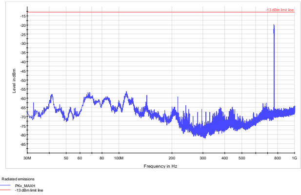
Figure 8.6-2: Radiated spurious emissions within 30 MHz to 1 GHz – Middle Channel (700FirstNet)
