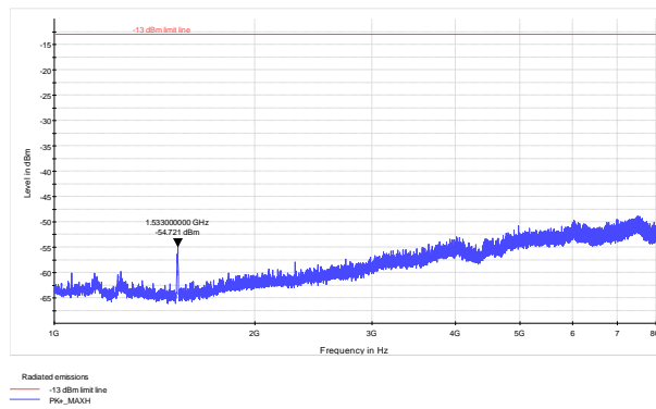
Figure 8.6-4: Radiated spurious emissions within 1 to 8 GHz – Low Channel (700FirstNet)
