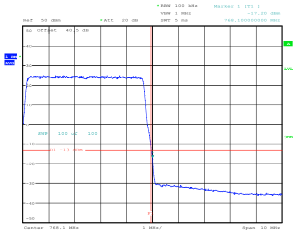
Figure 8.5-19: Conducted upper band edge at 768 MHz at AGC threshold (700FistNet)
