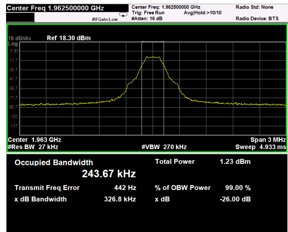
MSK Signal, Nominal Input Signal, Input
