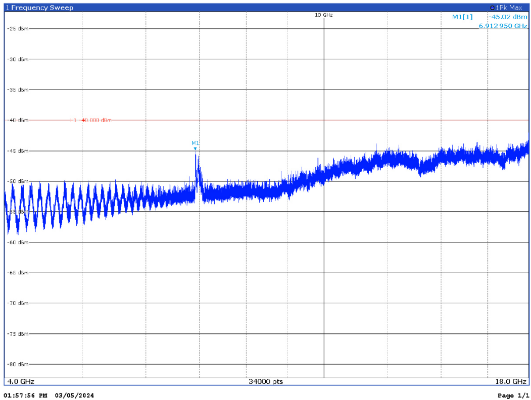
100 MHz signal, Bottom=Middle=Top Channel, 4GHz - 18GHz, H Pol
