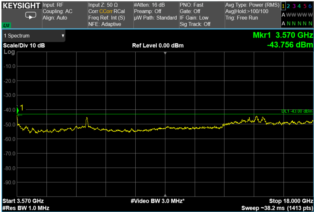
100 MHz signal, bottom=middle=top channel, Range: 3.57GHz – 18GHz
