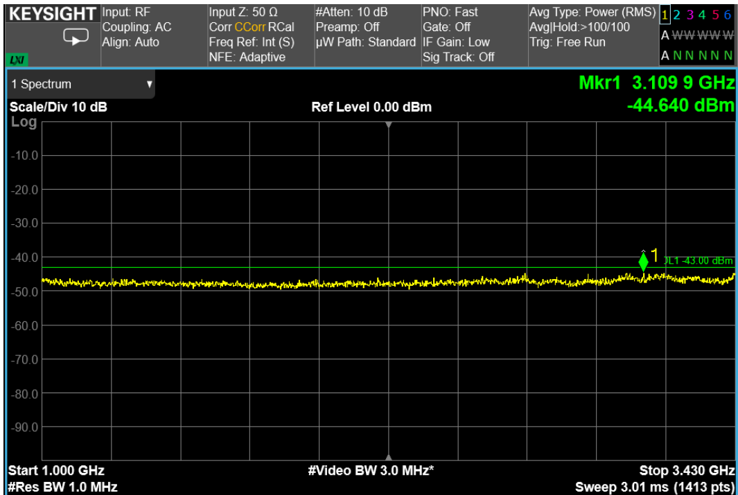
100 MHz signal, bottom=middle=top channel, Range: 1GHz – 3.43GHz
