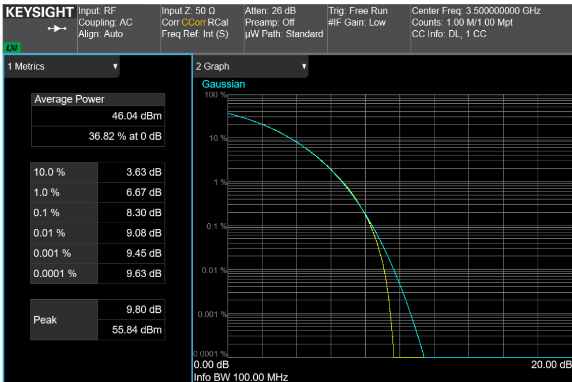
100 MHz signal, bottom=middle=top channel, nominal input signal
