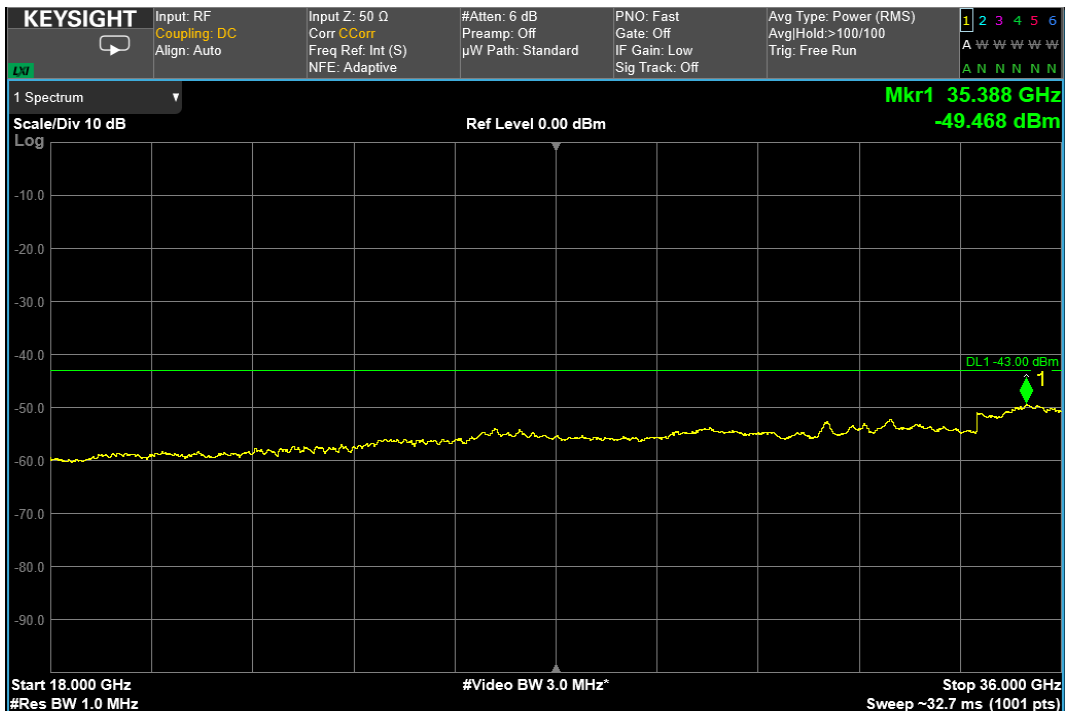
100 MHz signal, bottom=middle=top channel, Range: 18GHz – 36GHz
