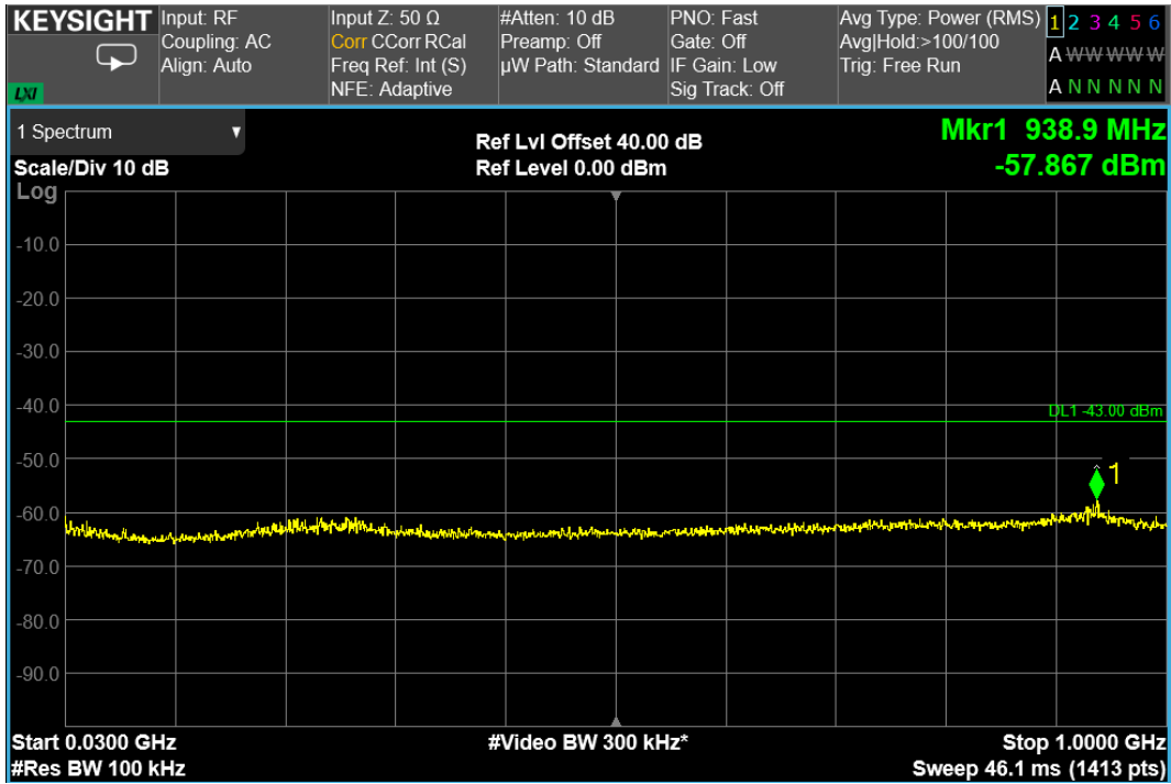
100 MHz signal, bottom=middle=top channel, Range: 30MHz - 1GHz
