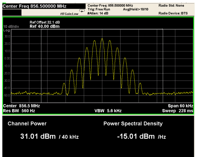
Mod. FM
