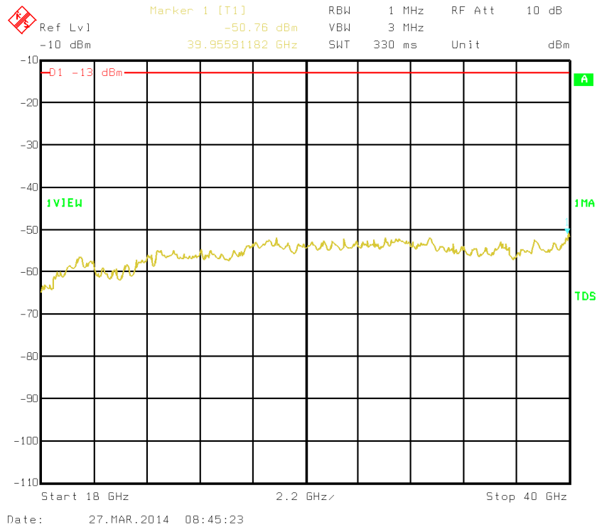
18GHz-40GHz – V Pol
