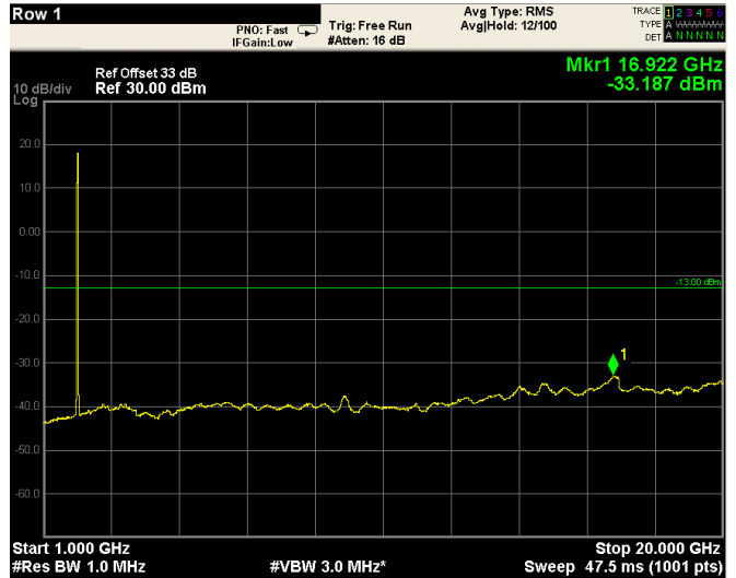
1GHz-20GHz
