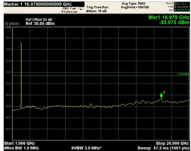
1GHz-20GHz
