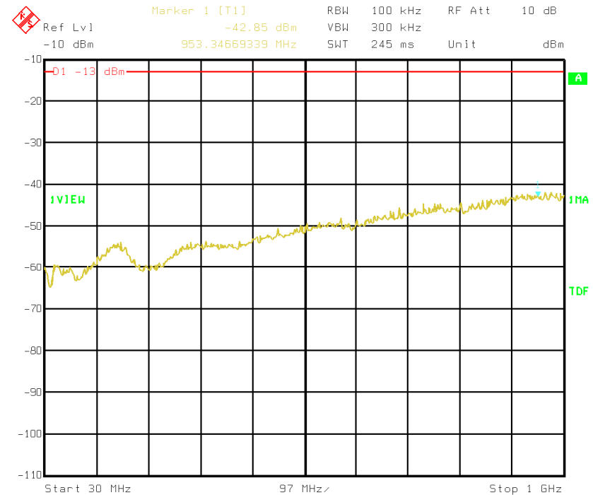
30MHz-1GHz – V Pol
