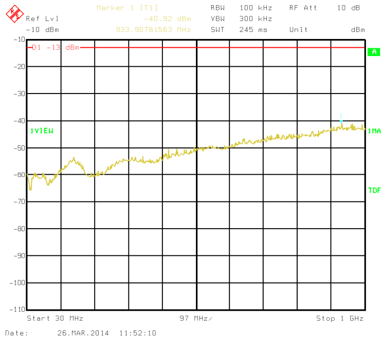
30MHz-1GHz – V Pol
