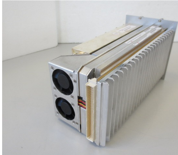
TDFE-8S module, rear view
