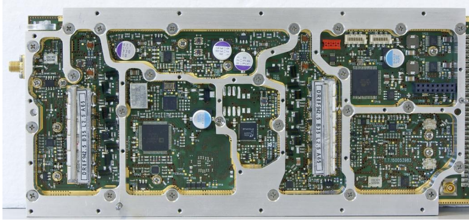
Down-link module
