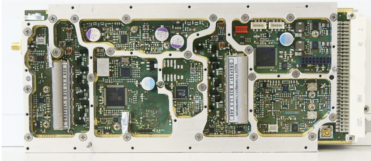
Down-link module
