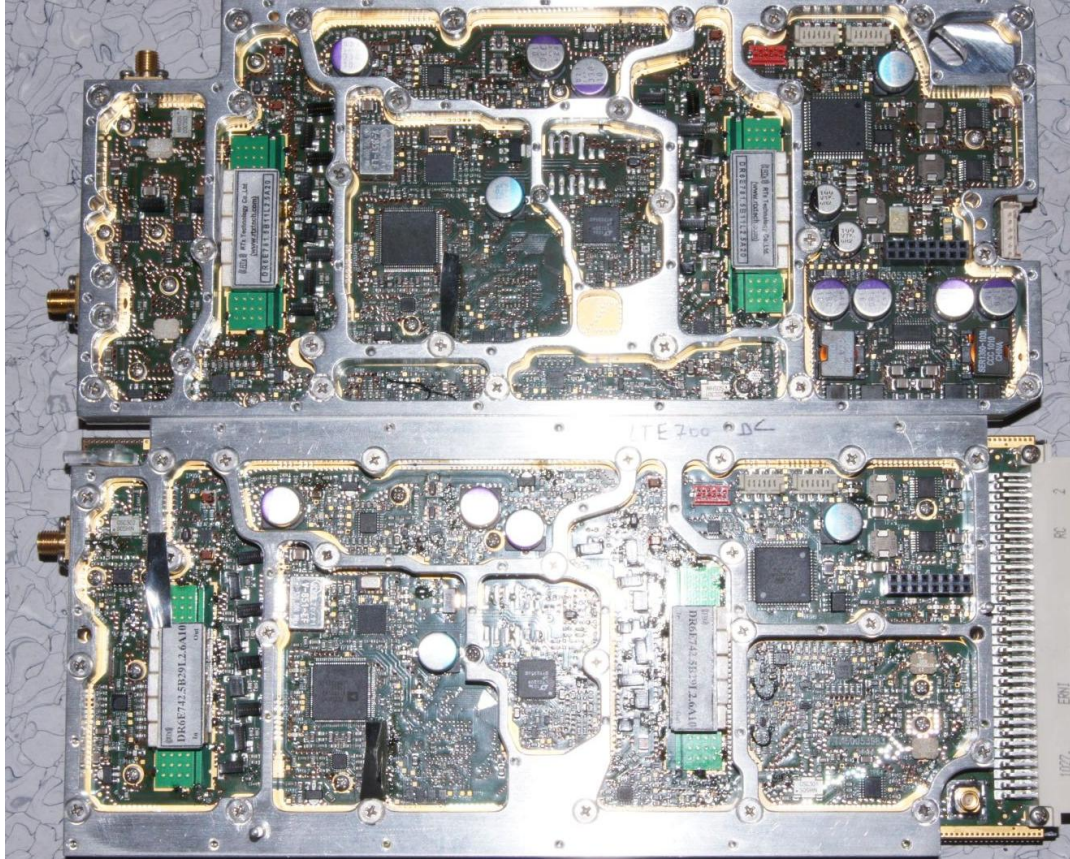
Down-link and Up-link module
