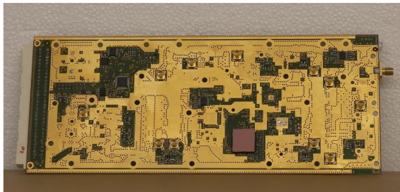
Down-link module
