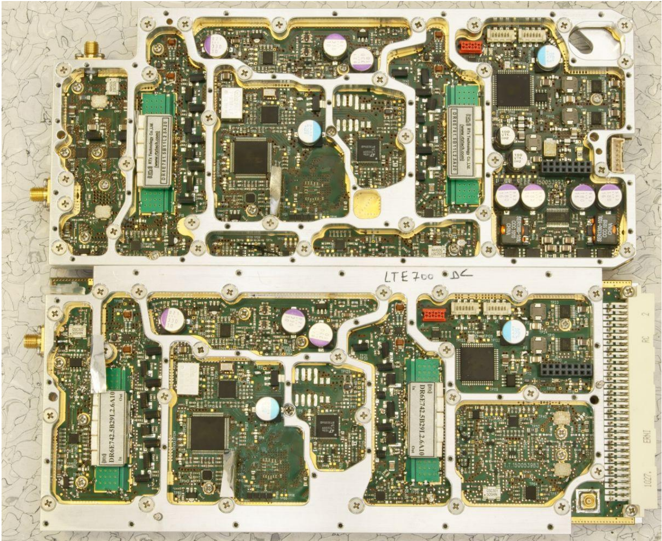
Down-link and Up-link module
