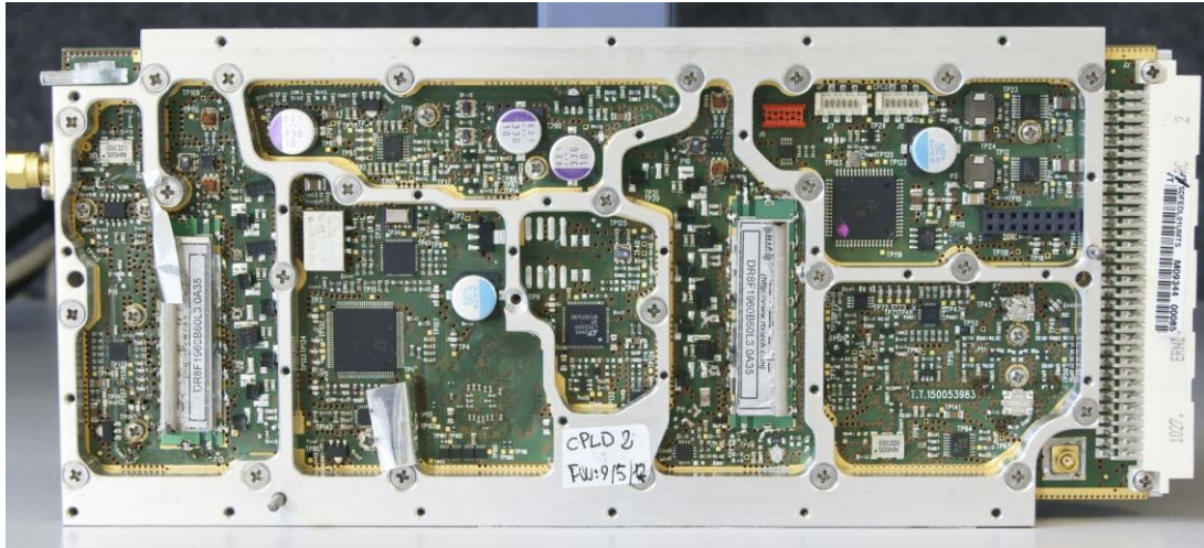
Down-link module
