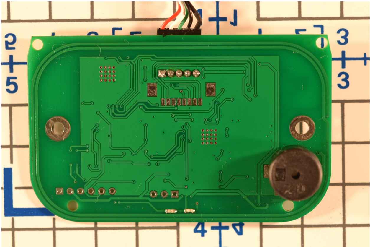
ADRB-USB-V2 PCB Bottom View
