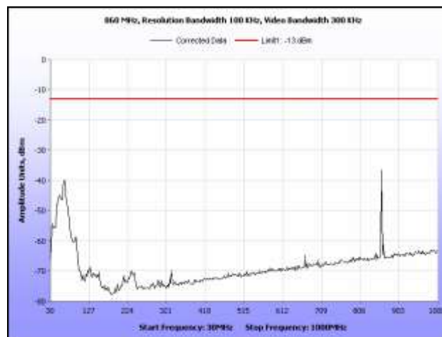
Plot 29. Radiated Spurious Emissions, 860 MHz, 30 MHz – 1 GHz
