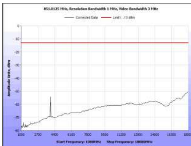
Plot 26. Radiated Spurious Emissions, 851.0125 MHz, 1 GHz – 18 GHz
