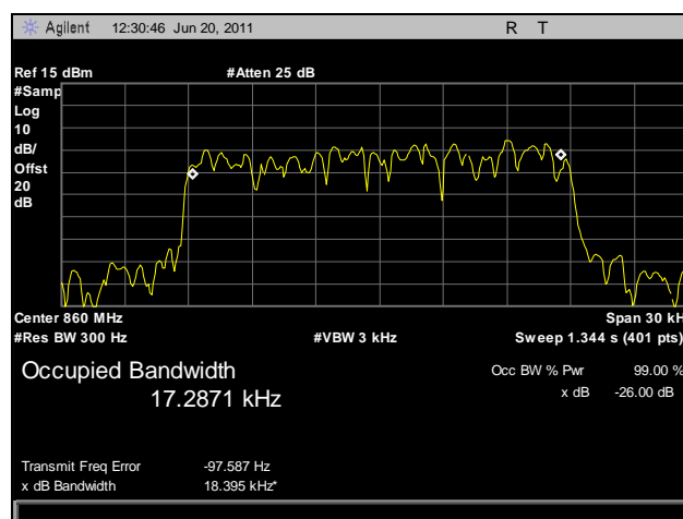
Plot 11. Occupied Bandwidth, Power In, 860 MHz
