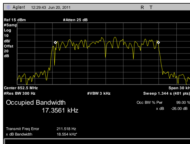
Plot 10. Occupied Bandwidth, Power In, 852.5 MHz
