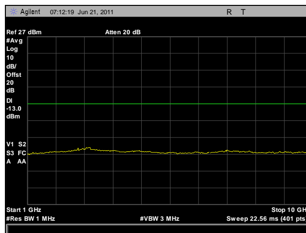
Plot 24. Conducted Spurious Emissions, 968.9875 MHz, 1 GHz – 10 GHz
