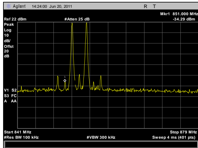
Plot 33. Intermodulation, Low Channel
