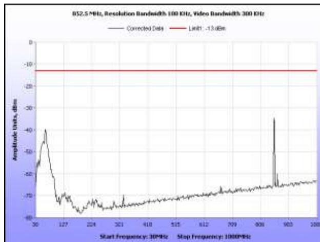
Plot 27. Radiated Spurious Emissions, 852.5 MHz, 30 MHz – 1 GHz
