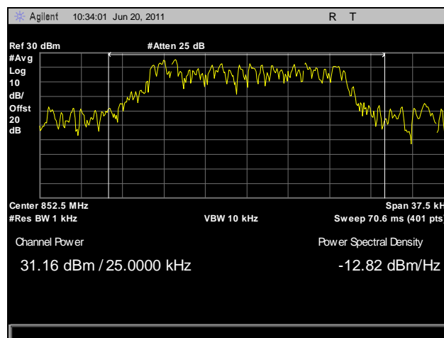
Plot 6. RF Power Output, Power Out, 852.5 MHz
