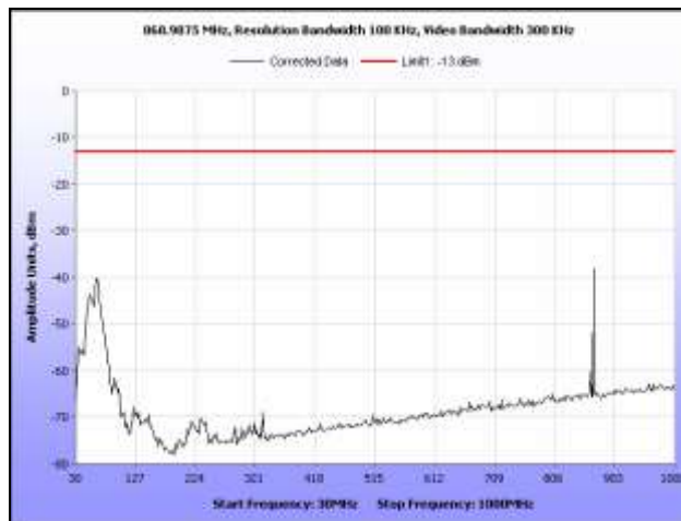
Plot 31. Radiated Spurious Emissions, 868.9875 MHz, 30 MHz – 1 GHz
