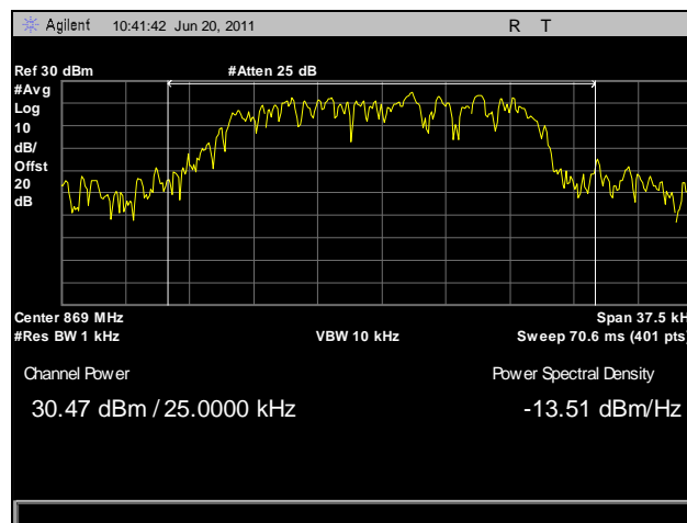
Plot 8. RF Power Output, Power Out, 868.9875
