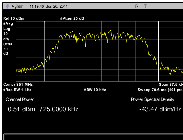
Plot 1. RF Power Output, Power In, 851.0125 MHz
