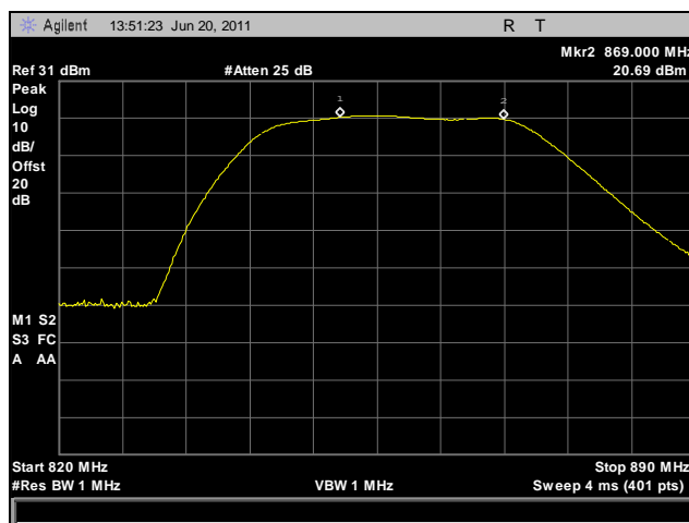
Plot 35. Filter Response
