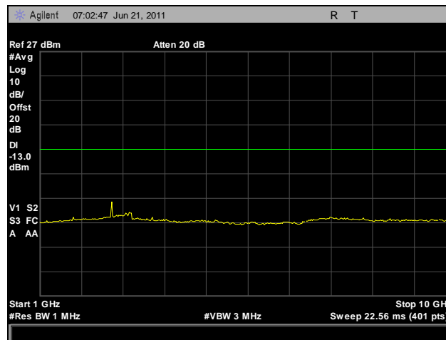
Plot 23. Conducted Spurious Emissions, 860 MHz, 1 GHz – 10 GHz
