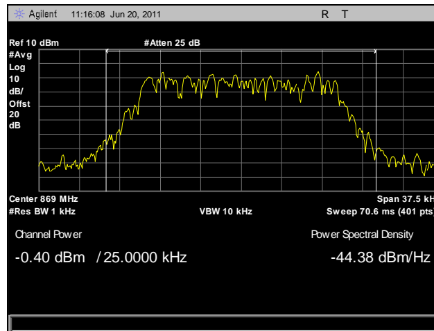
Plot 4. RF Power Output, Power In, 868.9875 MHz
