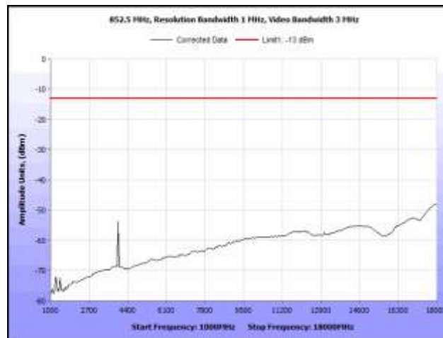
Plot 28. Radiated Spurious Emissions, 852.5 MHz, 1 GHz – 18 GHz
