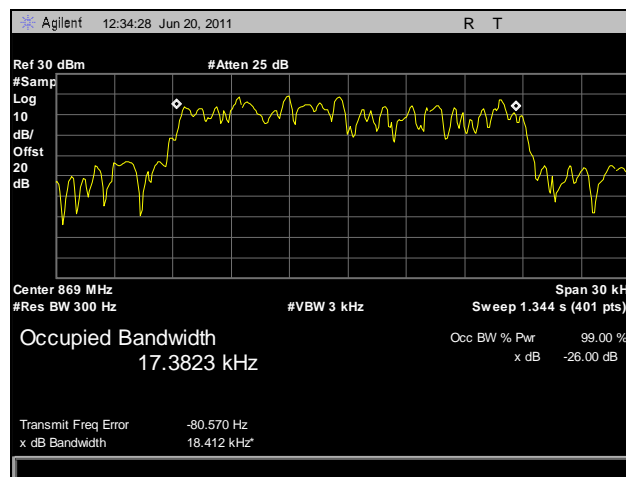
Plot 16. Occupied Bandwidth, Power Out, 868.9875 MHz
