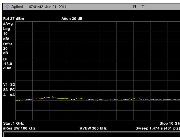
Plot 19. Conducted Spurious Emissions, 860 MHz, 1 GHz – 10 GHz
