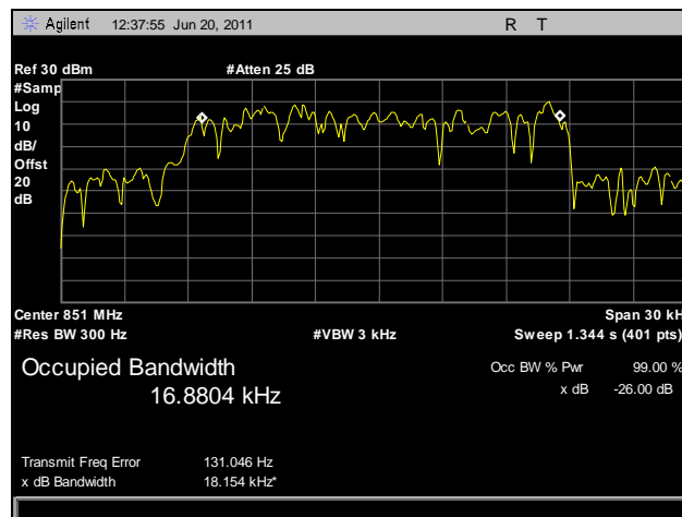
Plot 13. Occupied Bandwidth, Power Out, 851.0125 MHz
