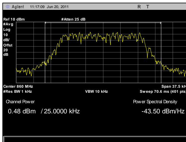
Plot 3. RF Power Output, Power In, 860 MHz
