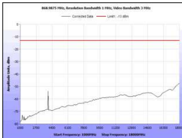
Plot 32. Radiated Spurious Emissions, 868.9875 MHz, 1 GHz – 18 GHz
