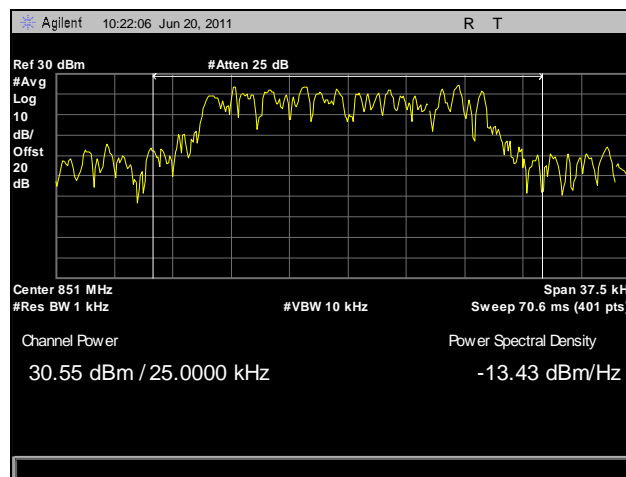
Plot 5. RF Power Output, Power Out, 851.0125 MHz
