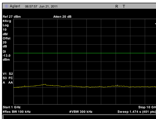
Plot 18 Conducted Spurious Emissions, 852.5 MHz, 1 GHz – 10 GHz
