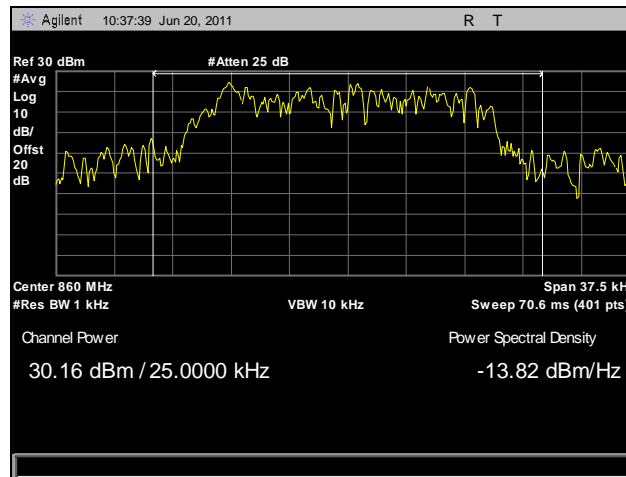
Plot 7. RF Power Output, Power Out, 860 MHz
