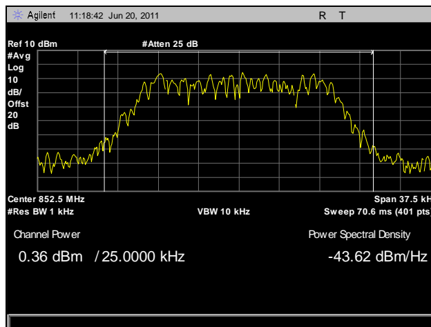
Plot 2. RF Power Output, Power In, 852.5 MHz
