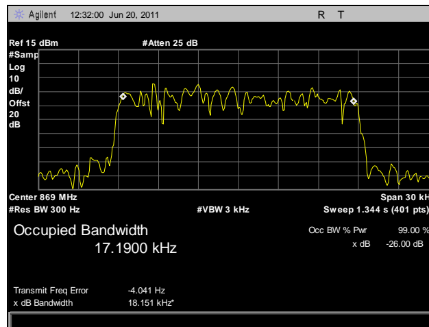
Plot 12. Occupied Bandwidth, Power In, 868.9875 MHz
