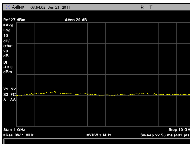
Plot 21. Conducted Spurious Emissions, 851.0125 MHz, 1 GHz – 10 GHz
