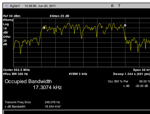
Plot 14. Occupied Bandwidth, Power Out, 852.5 MHz
