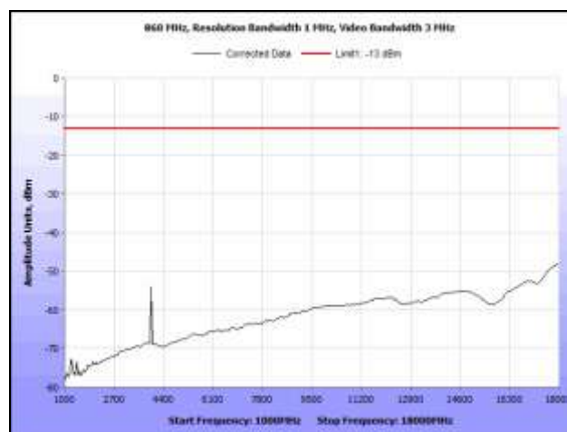
Plot 30. Radiated Spurious Emissions, 860 MHz, 1 GHz – 18 GHz
