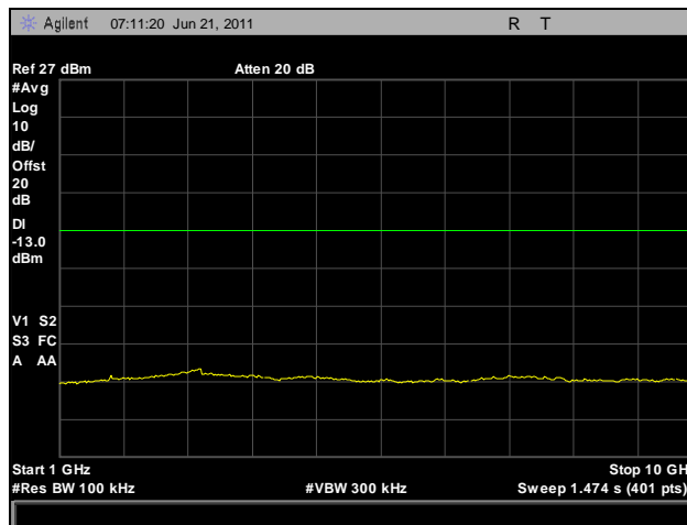
Plot 20. Conducted Spurious Emissions, 868.9875 MHz, 1 GHz – 10 GHz
