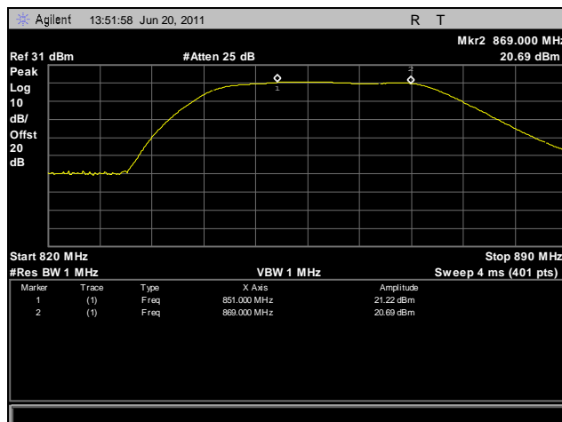
Plot 36. Filter Response with Marker Table
