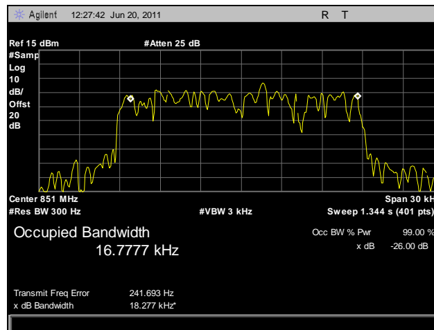
Plot 9. Occupied Bandwidth, Power In, 851.0125 MHz
