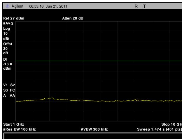
Plot 17. Conducted Spurious Emissions, 851.0125 MHz, 1 GHz – 10 GHz
