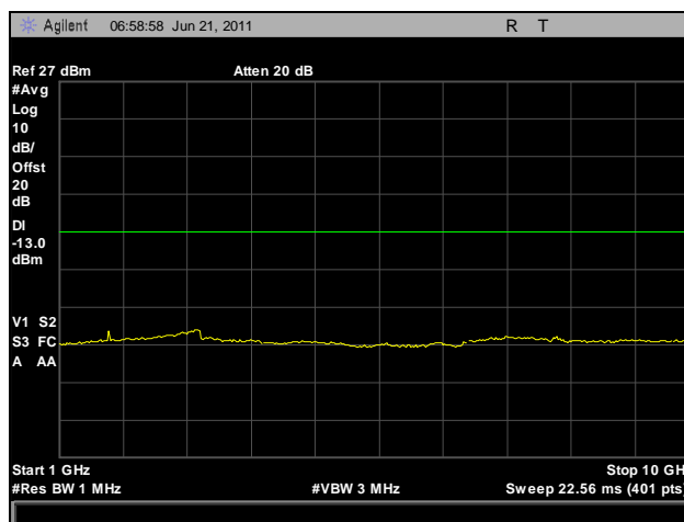
Plot 22. Conducted Spurious Emissions, 852.5 MHz, 1 GHz – 10 GHz
