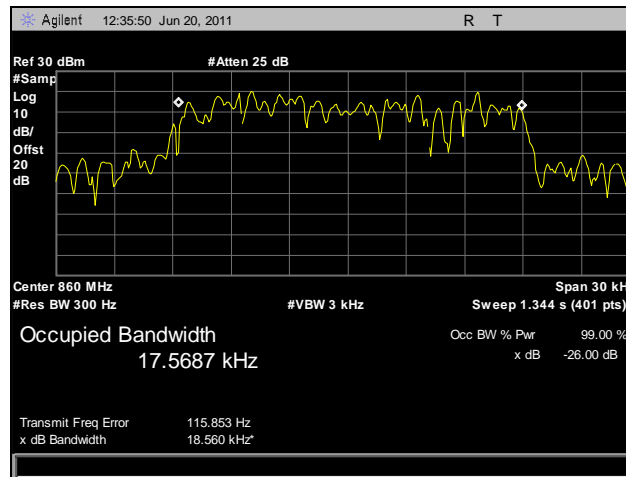
Plot 15. Occupied Bandwidth, Power Out, 860 MHz
